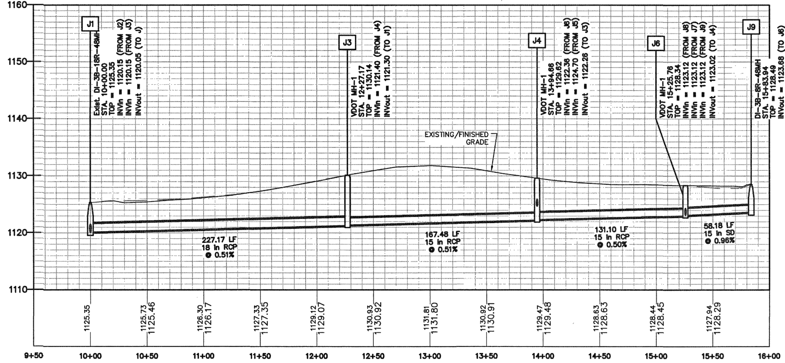
PROFILE - LINE J SCALE VERTICAL: 1" = 10' HORIZONTAL: 1" = 50'
