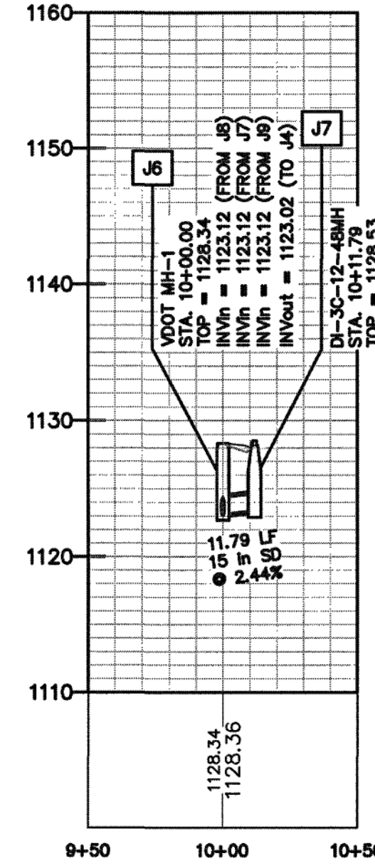
PROFILE - LINE J7 SCALE VERTICAL: 1" = 10' HORIZONTAL: 1" = 50'
