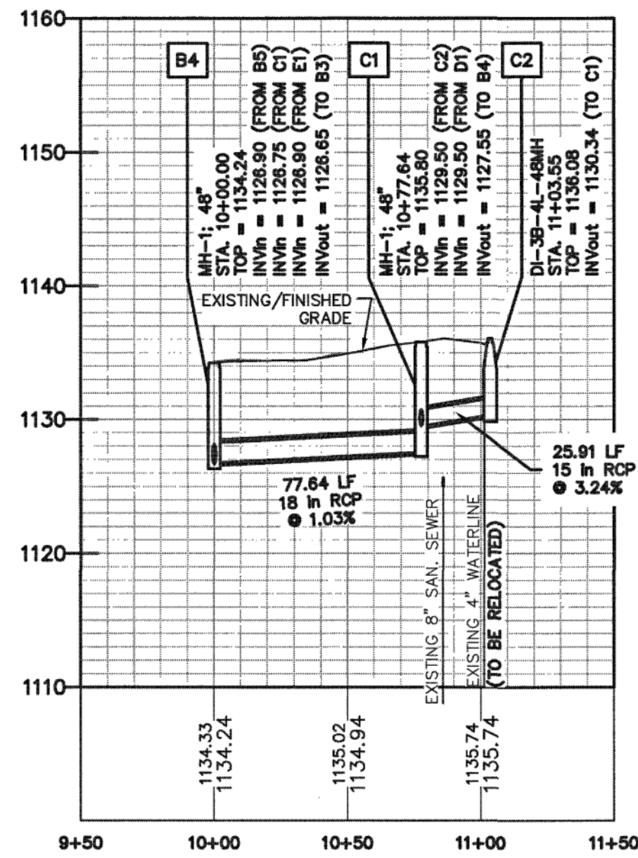
PROFILE - LINE C SCALE VERTICAL: 1" = 10' HORIZONTAL: 1" = 50'
