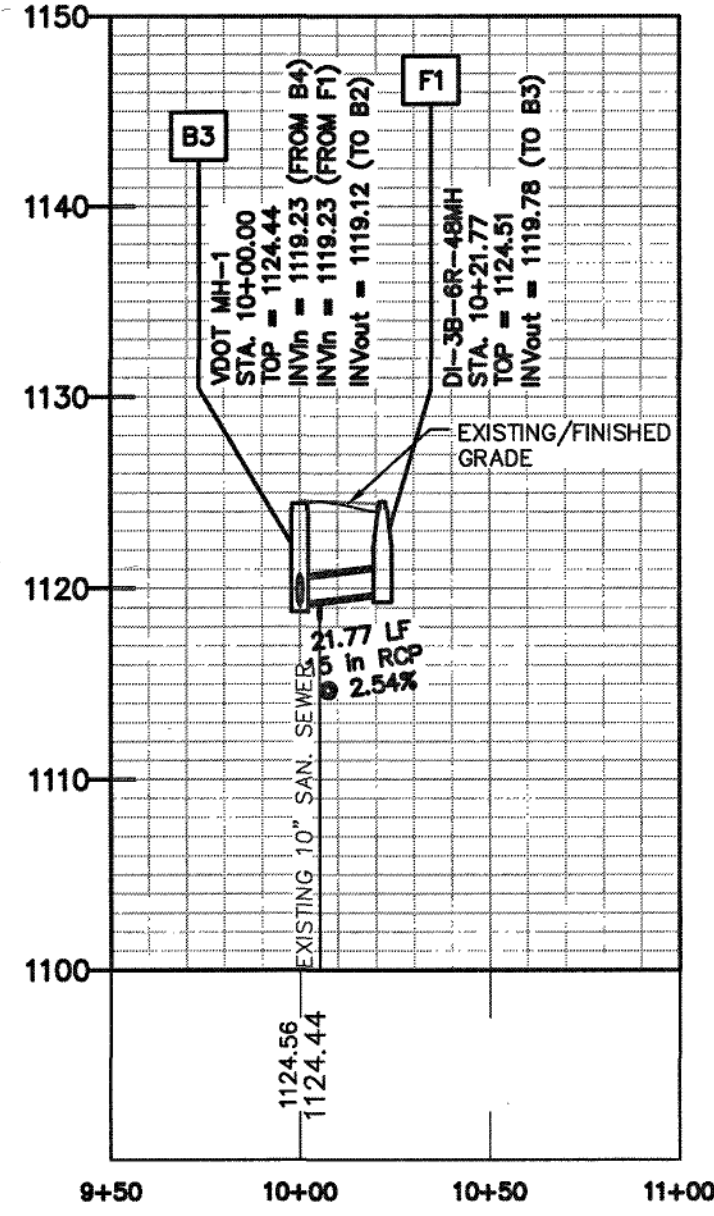
PROFILE - LINE F SCALE VERTICAL: 1" = 10' HORIZONTAL: 1" = 50'
