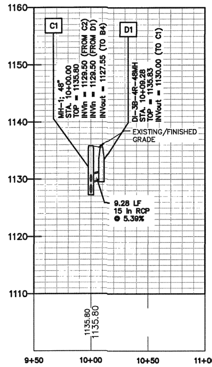
PROFILE - LINE D SCALE VERTICAL: 1" = 10' HORIZONTAL: 1" = 50'
