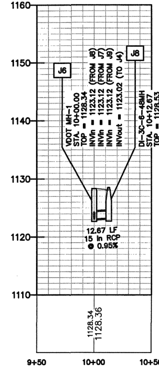
PROFILE - LINE J8 SCALE VERTICAL: 1" = 10' HORIZONTAL: 1" = 50'
