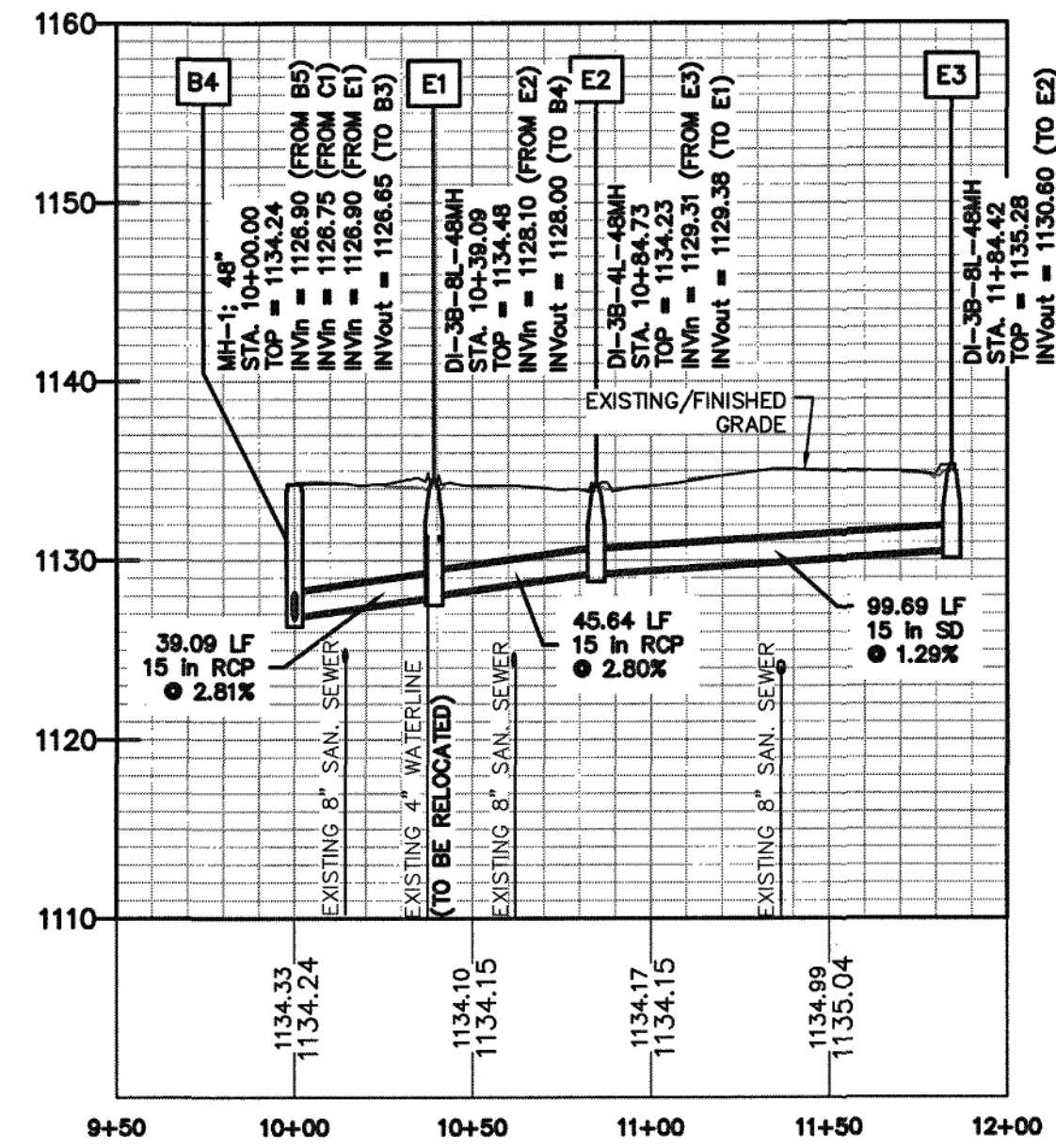
PROFILE - LINE E SCALE VERTICAL: 1" = 10' HORIZONTAL: 1" = 50'
