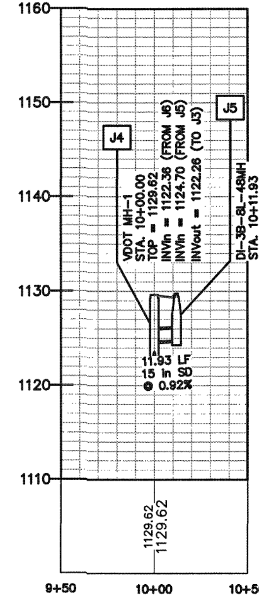
PROFILE - LINE J5 SCALE VERTICAL: 1" = 10' HORIZONTAL: 1" = 50'
