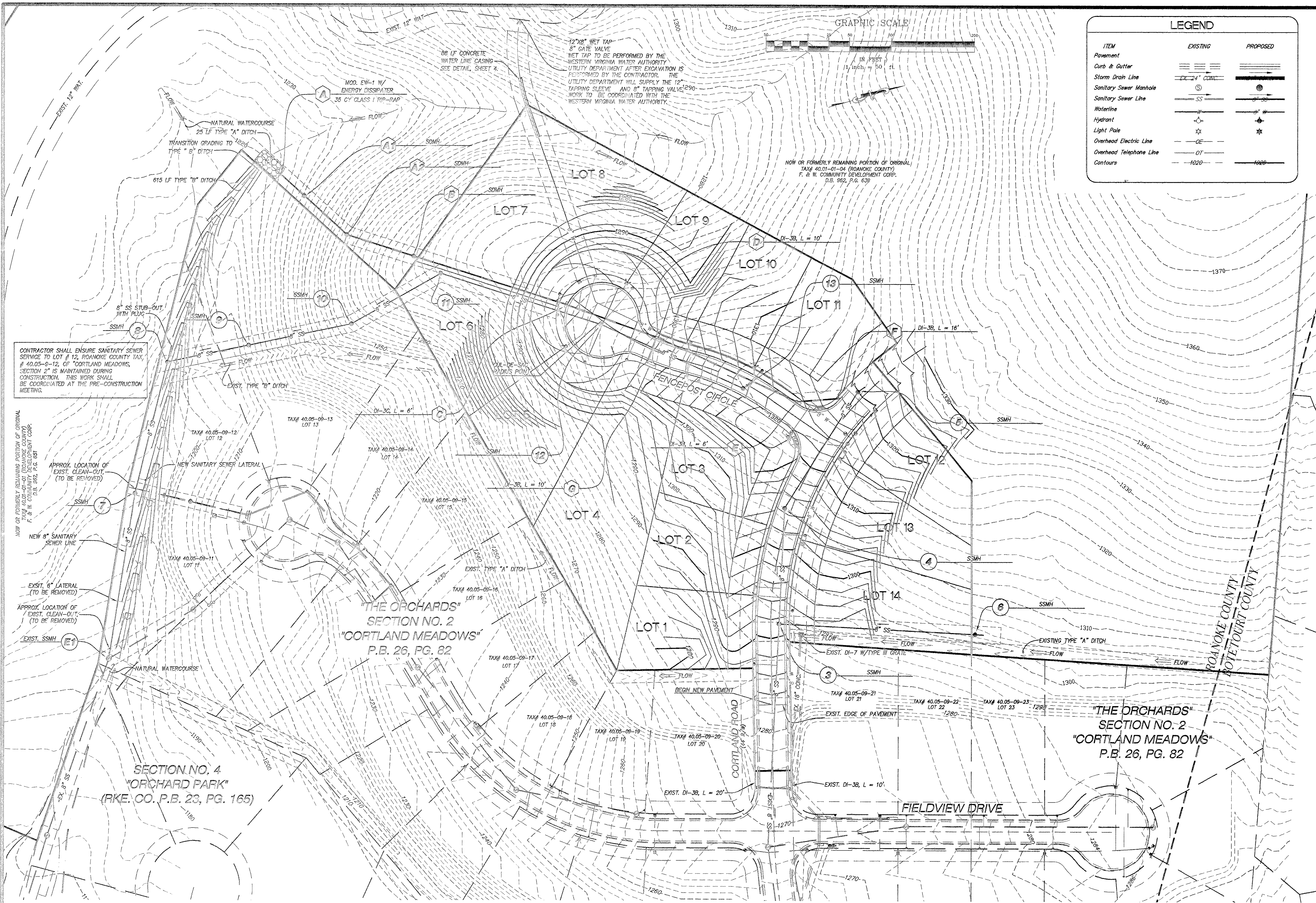
GRADING PLAN
