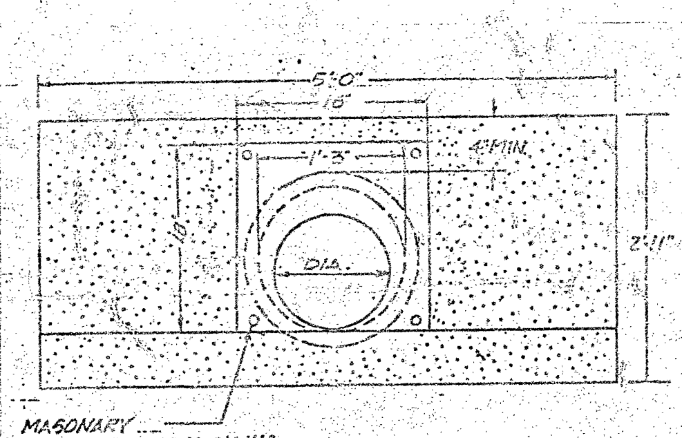
ENDWALL DETAIL "A"
