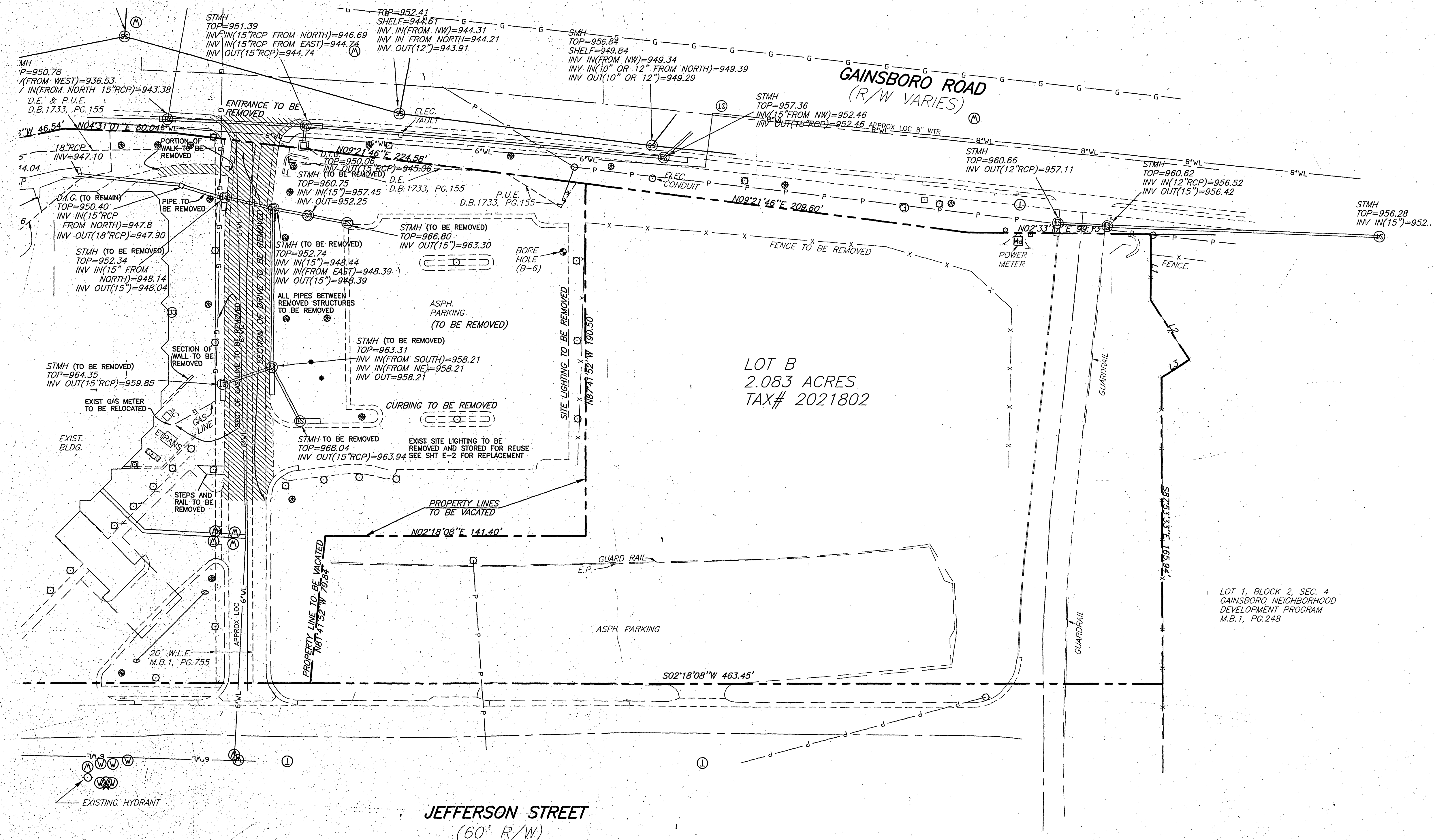
SITE DEMOLITIONS PLAN SCALE: 1"=30'
