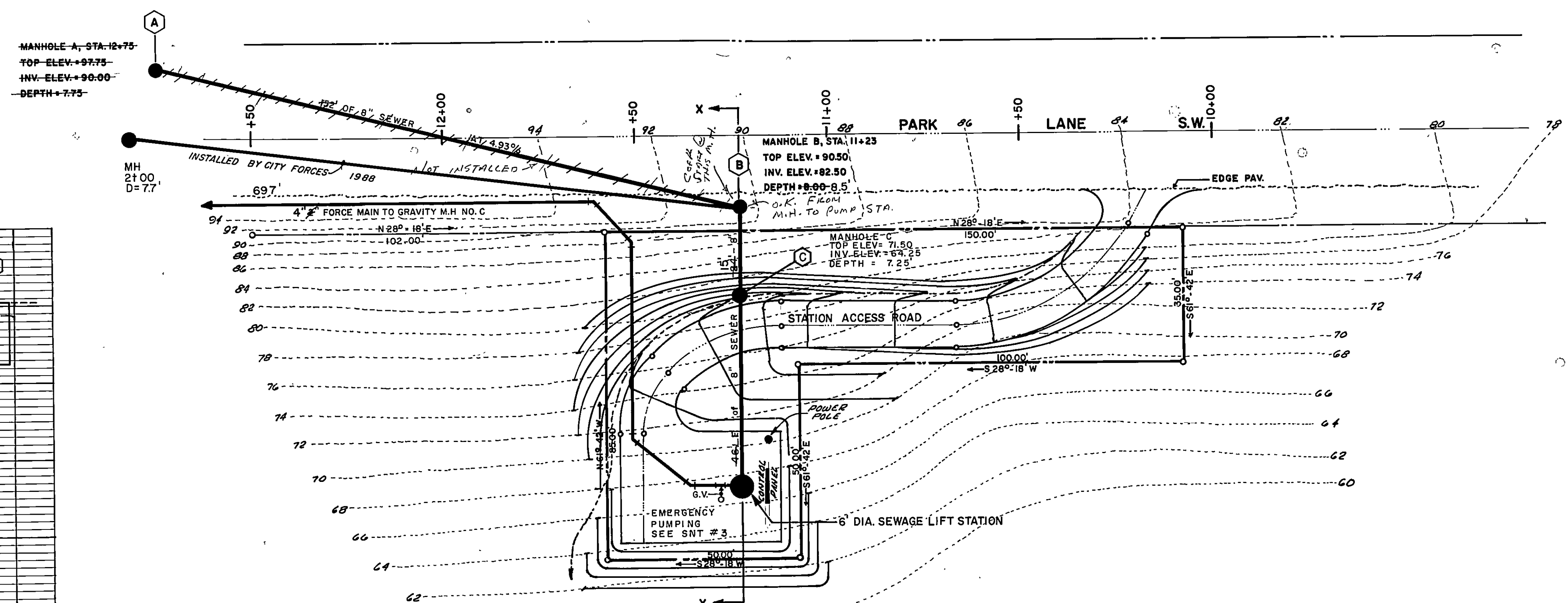
SEWAGE LIFT STATION SITE PLAN SCALE: 1" = 20'
