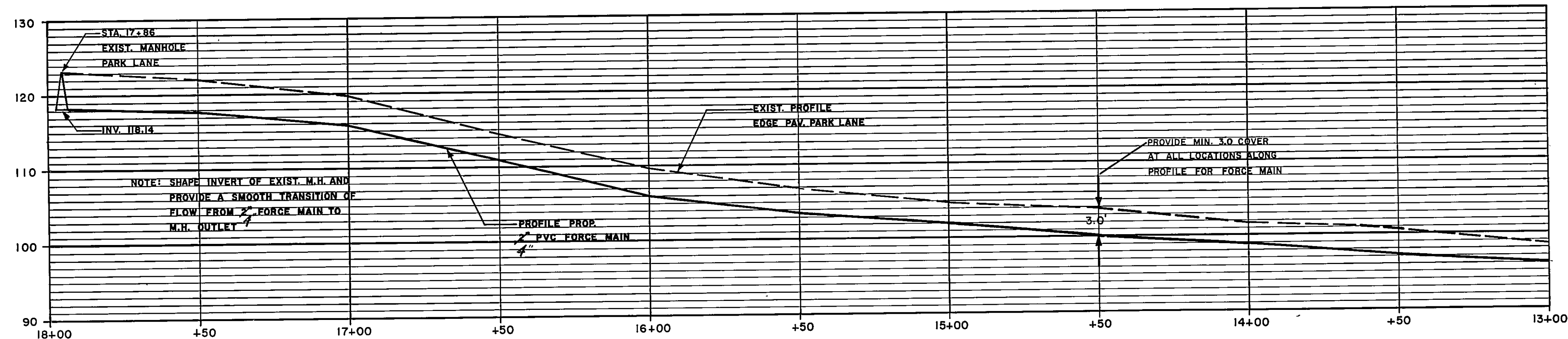
SEWER FORCE MAIN PROFILE SCALE: 1" = 25' HORIZONTAL 1" = 10' VERTICAL
