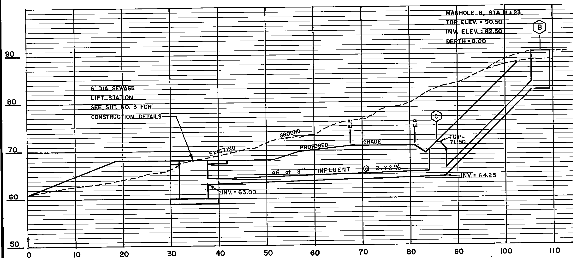
SECTION X-X ELEVATION THRU STATION SITE SCALE: 1" = 10' HORIZONTAL 1" = 10' VERTICAL
