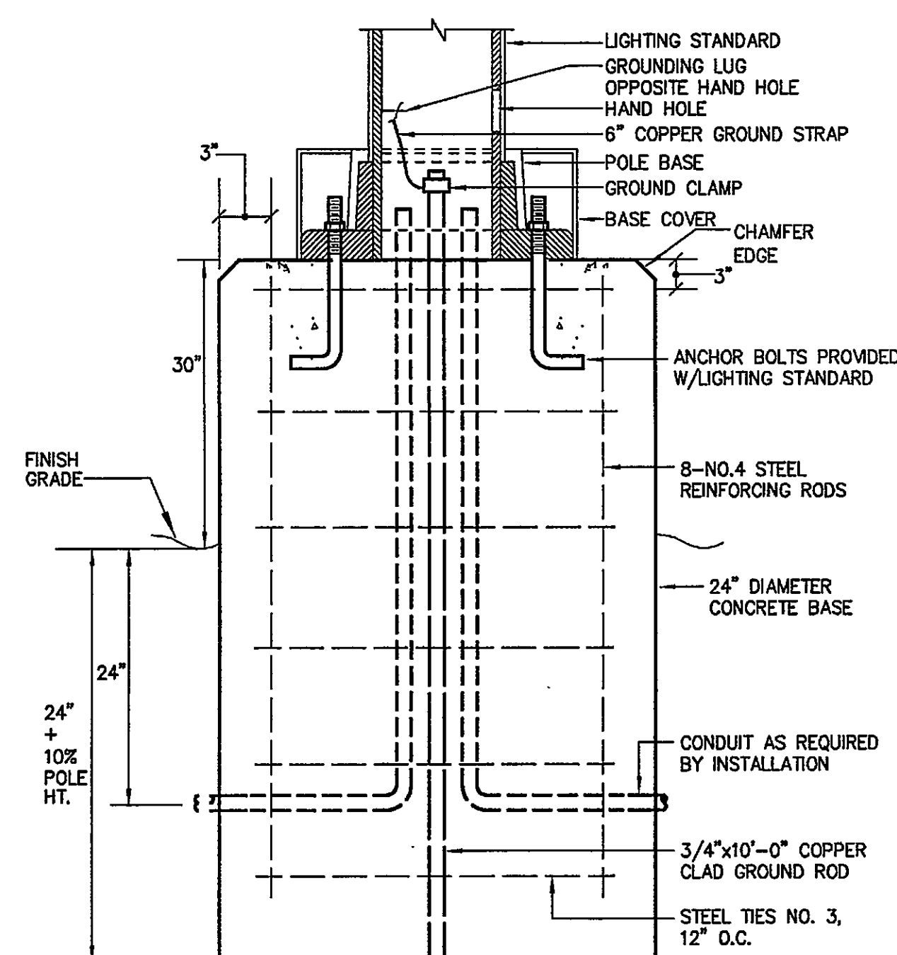
POLE BASE DETAIL FIXTURE TYPES A, C, D AND E NO SCALE
