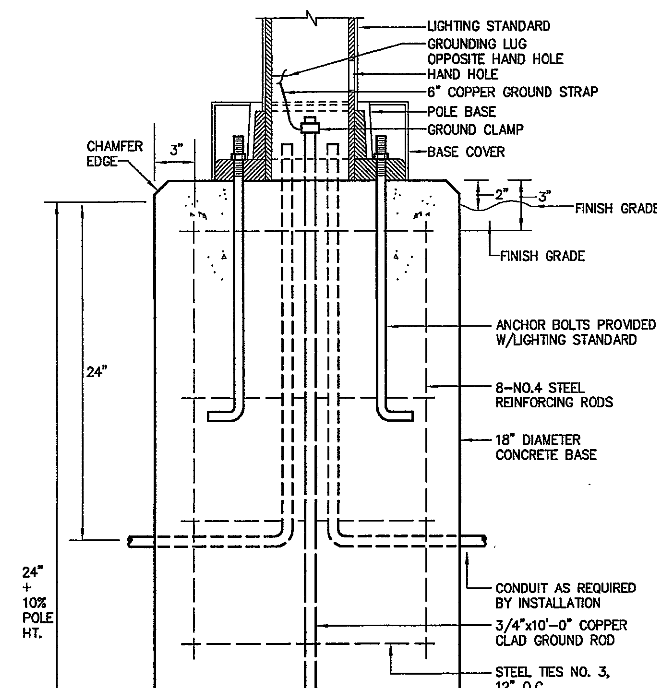
POLE BASE DETAIL FIXTURE TYPE B NO SCALE
