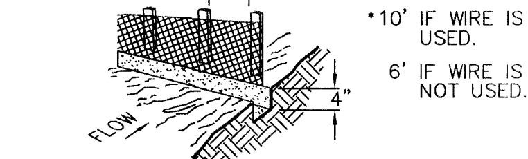
(SF) CONSTRUCTION OF A SILT FENCE
