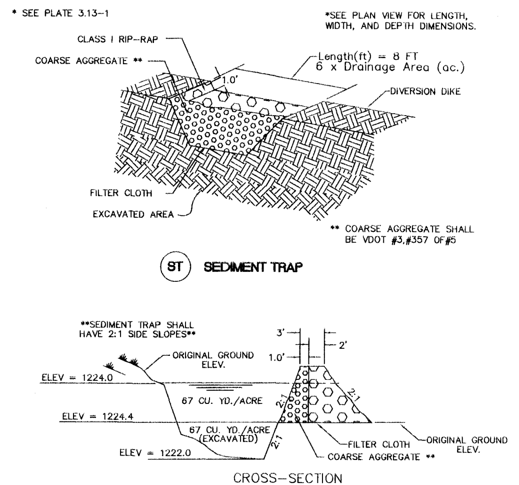
SEDIMENT TRAP DETAIL
