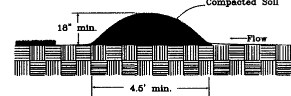
TEMPORARY DIVERSION DIKE
