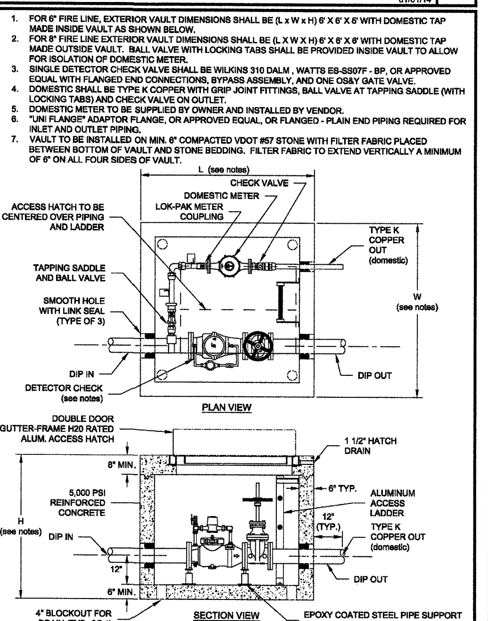
WESTERN VIRGINIA REGIONAL - CONSTRUCTION DETAIL COMMERCIAL METER VAULT 0101/14 W-7
