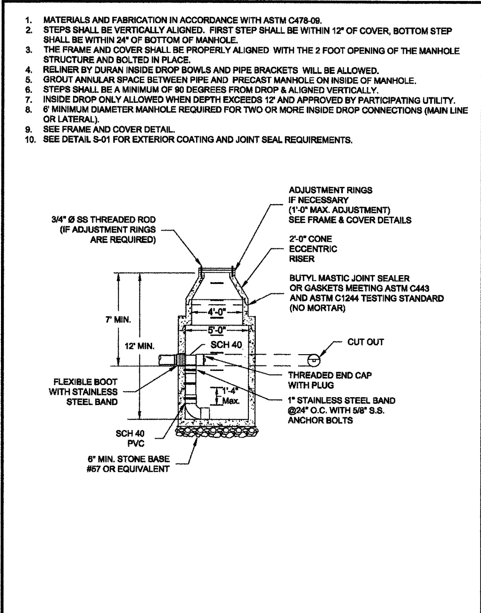
WESTERN VIRGINIA REGIONAL - CONSTRUCTION DETAIL INSIDE DROP MANHOLE 0101/14 S-3
