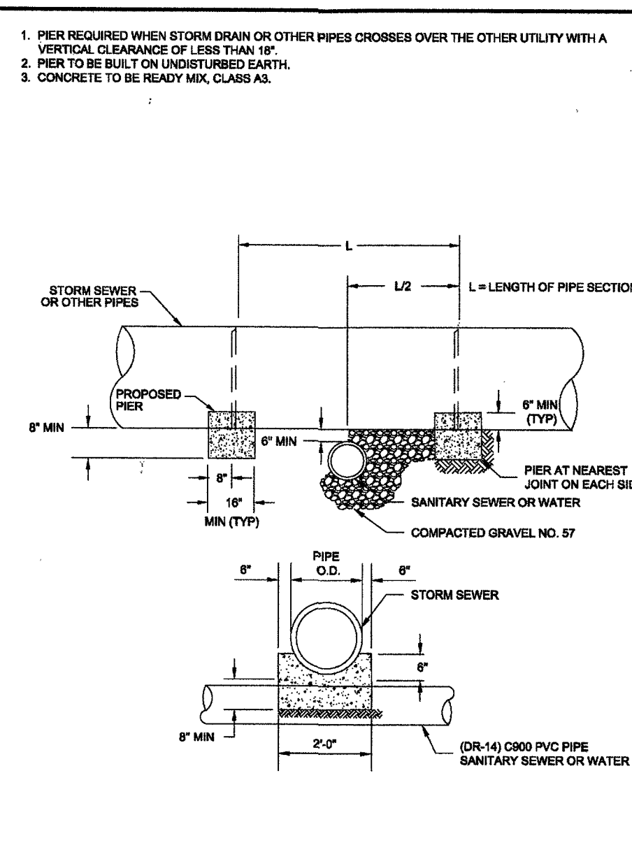
WESTERN VIRGINIA REGIONAL - CONSTRUCTION DETAIL CONCRETE PIER 0101/14 G-8
