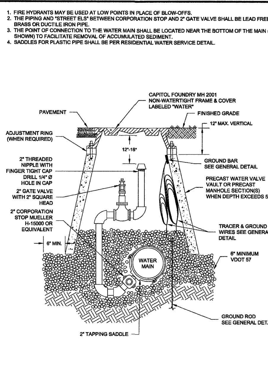
WESTERN VIRGINIA REGIONAL - CONSTRUCTION DETAIL IN-LINE BLOW-OFF ASSEMBLY 0101/14 W-12
