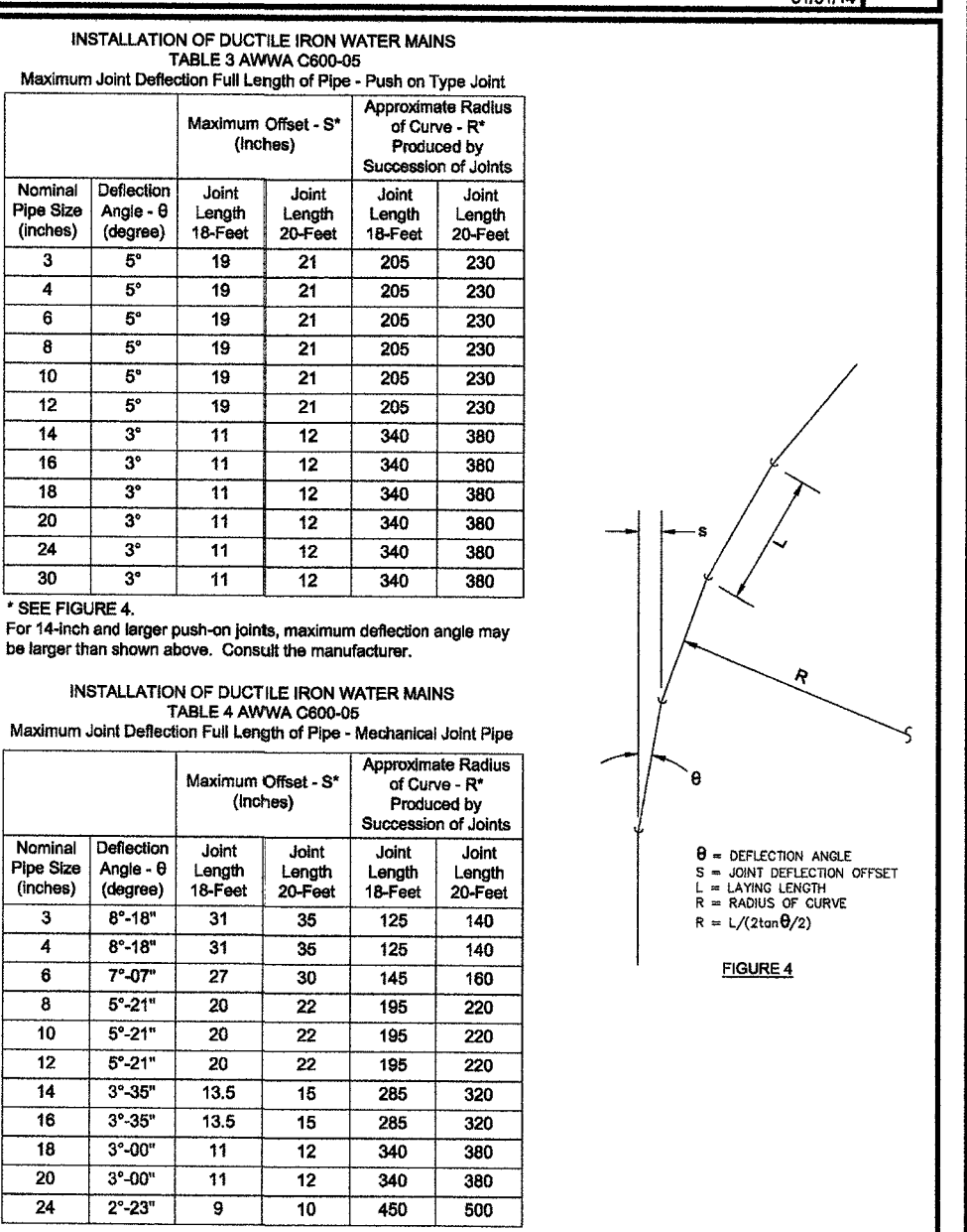
WESTERN VIRGINIA REGIONAL - CONSTRUCTION DETAIL DUCTILE IRON PIPE DEFLECTION ALLOWANCE TABLES 0101/14 W-22
