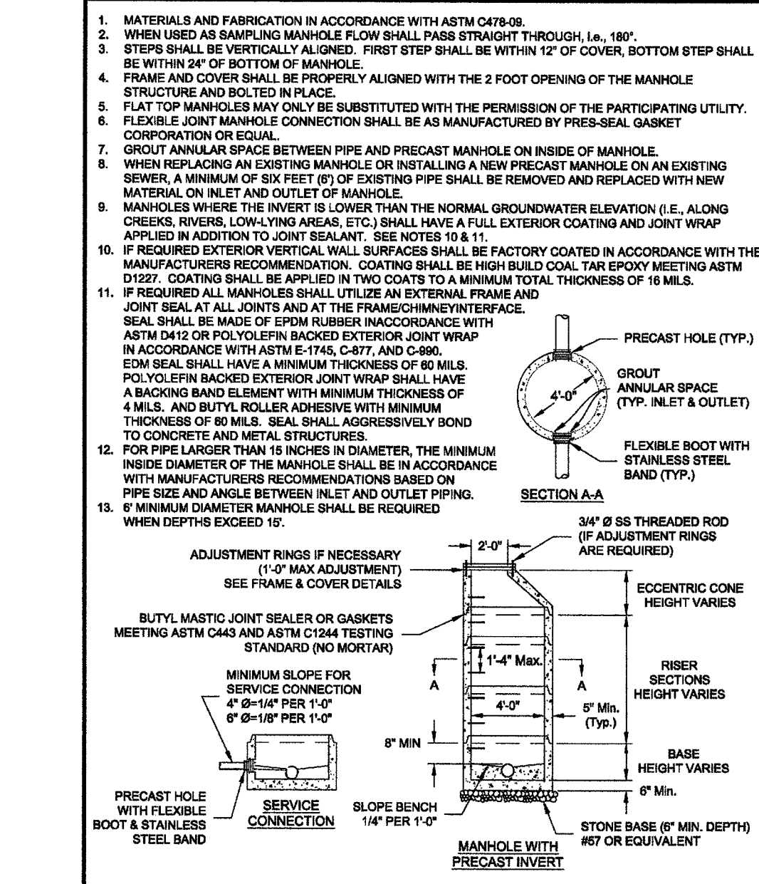
WESTERN VIRGINIA REGIONAL - CONSTRUCTION DETAIL 4" STANDARD MANHOLE FOR PIPE 15" OR SMALLER (FOR DEPTHS UP TO 15 FEET) 0101/14 S-1
