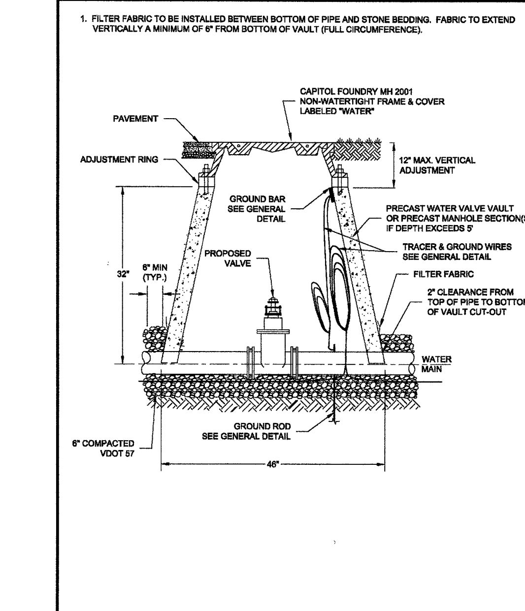
WESTERN VIRGINIA REGIONAL - CONSTRUCTION DETAIL WATER LINE VALVE & VAULT 0101/14 W-9
