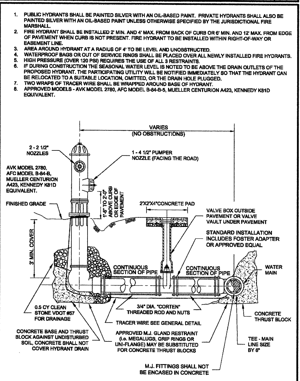
WESTERN VIRGINIA REGIONAL - CONSTRUCTION DETAIL FIRE HYDRANT ASSEMBLY 0101/14 W-17
