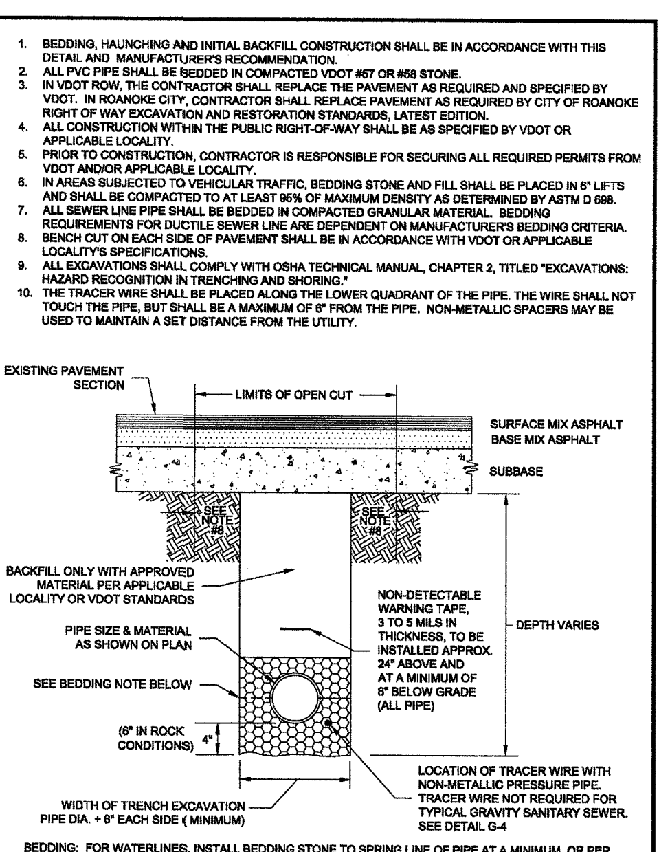
WESTERN VIRGINIA REGIONAL - CONSTRUCTION DETAIL BEDDING AND BACKFILL UNDER PAVEMENT AND IN RIGHT-OF-WAY 0101/14 G-12
