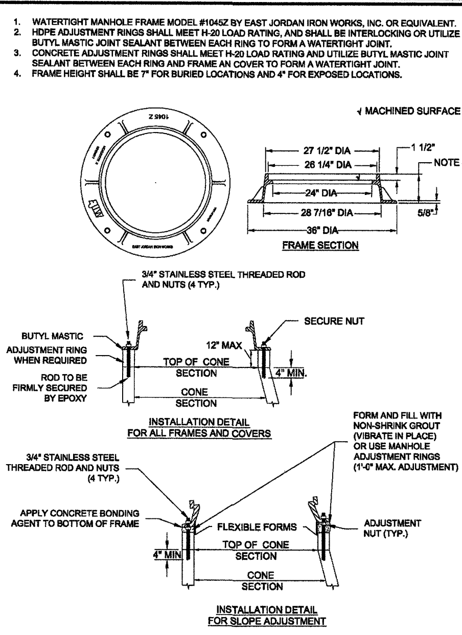
WESTERN VIRGINIA REGIONAL - CONSTRUCTION DETAIL WATERTIGHT MANHOLE FRAME 0101/14 S-4
