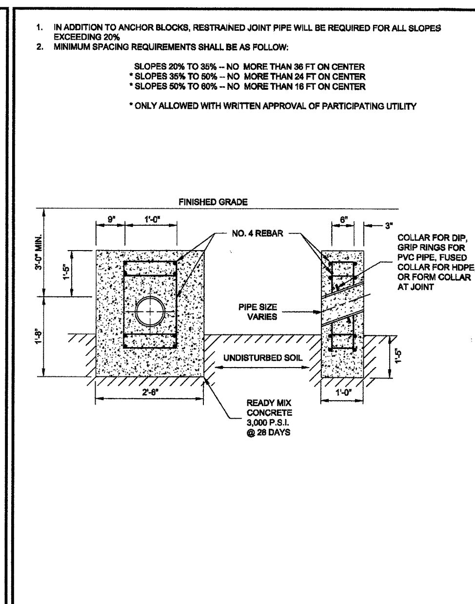
WESTERN VIRGINIA REGIONAL - CONSTRUCTION DETAIL ANCHOR BLOCK 0101/14 G-10
