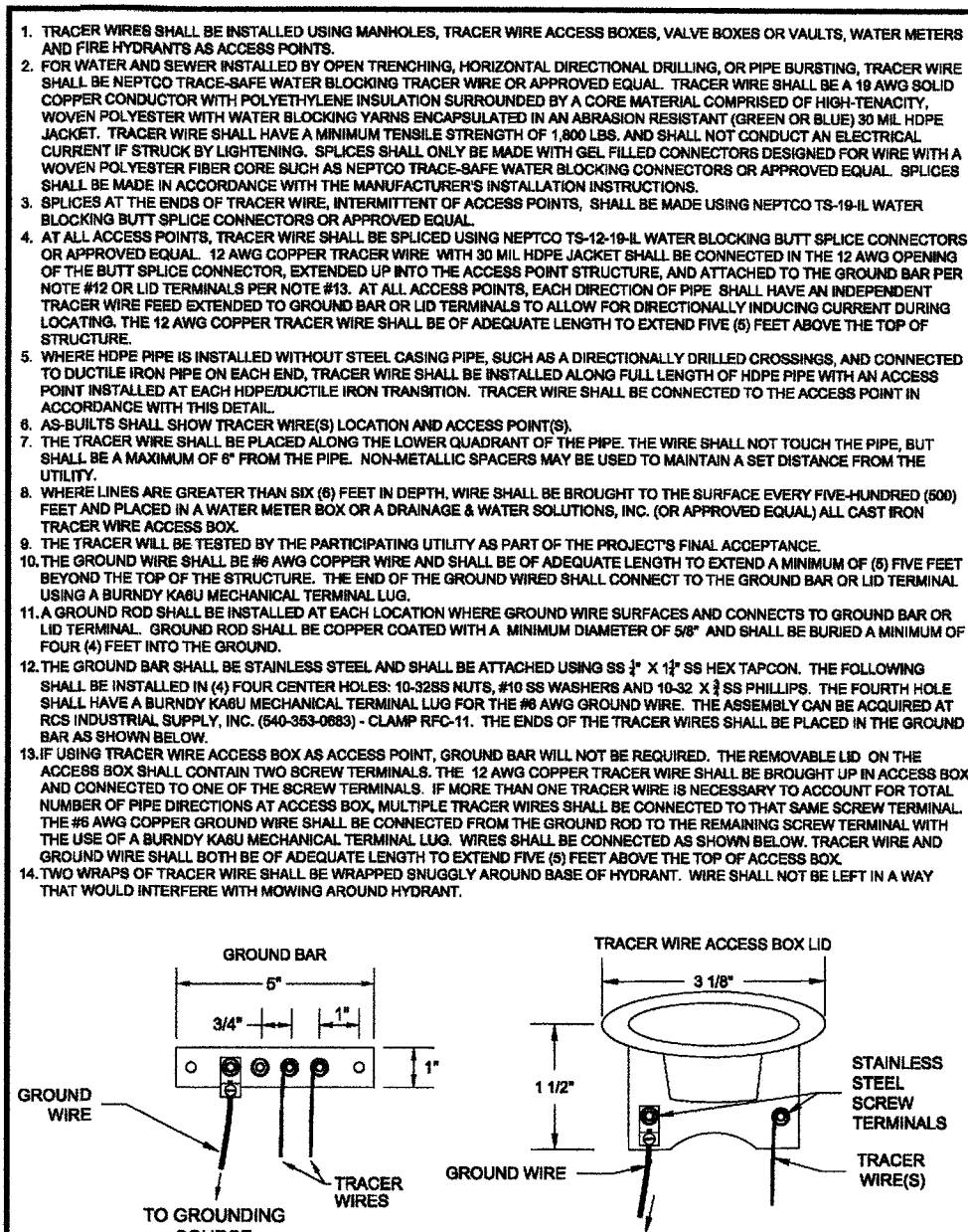
WESTERN VIRGINIA REGIONAL - CONSTRUCTION DETAIL TRACER WIRE FOR NON-METALLIC PRESSURE PIPE 0101/14 G-4
