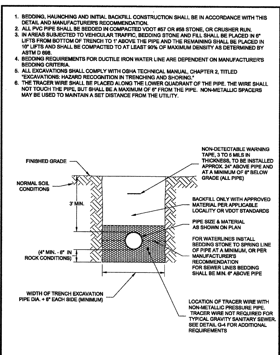
WESTERN VIRGINIA REGIONAL - CONSTRUCTION DETAIL BEDDING AND BACKFILL OUTSIDE OF PAVED AREAS 0101/14 G-11
