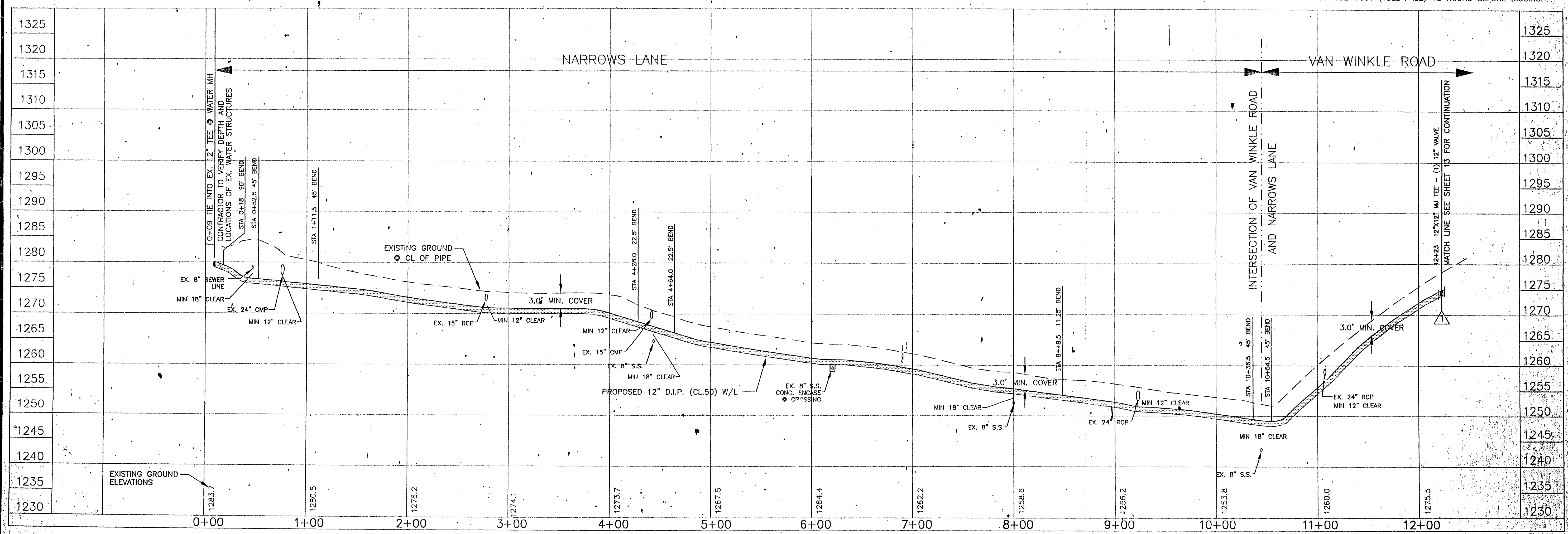
12" WATER LINE PROFILE VIEW-W/L STA 0+00 TO 12+23 SCALE: 1"=50' HORZ. & 1"=10' VERT.
