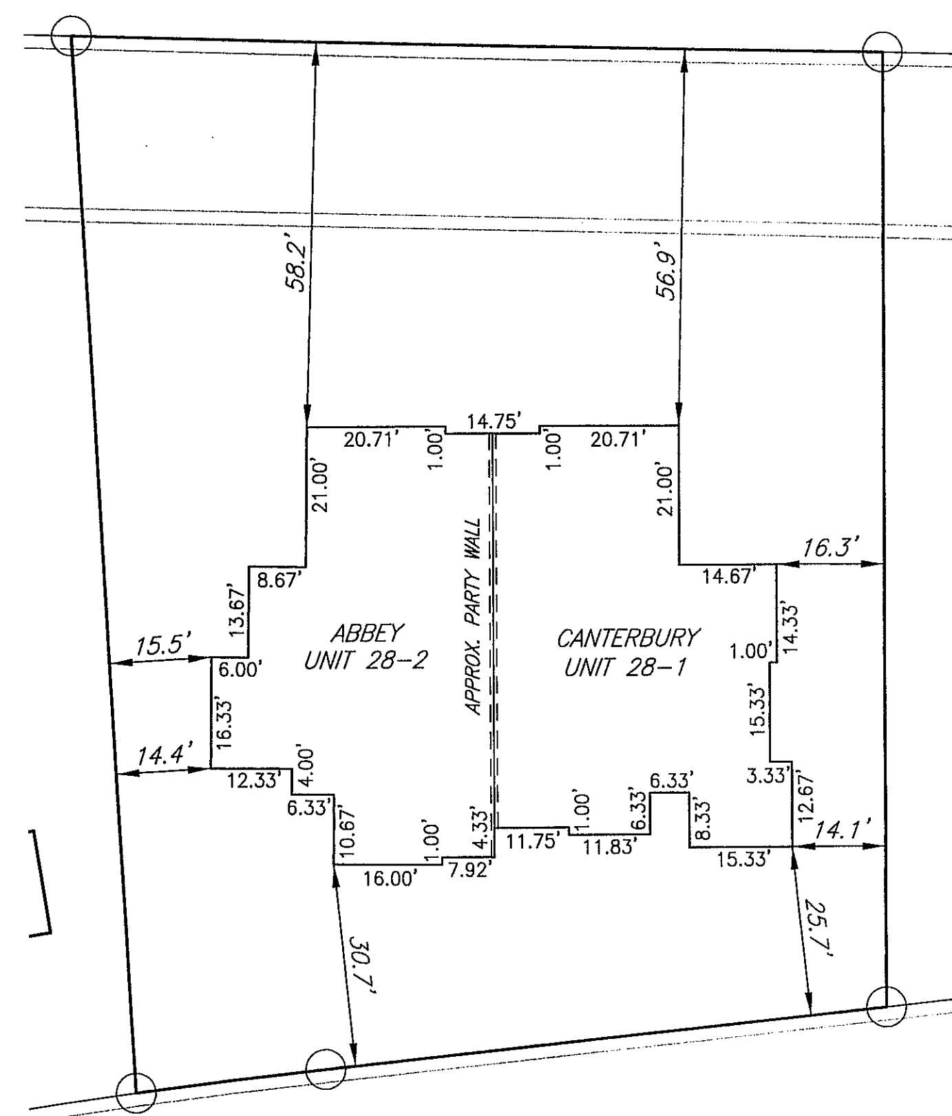
BUILDING 28 DETAIL NEW PHASE 10(B)
