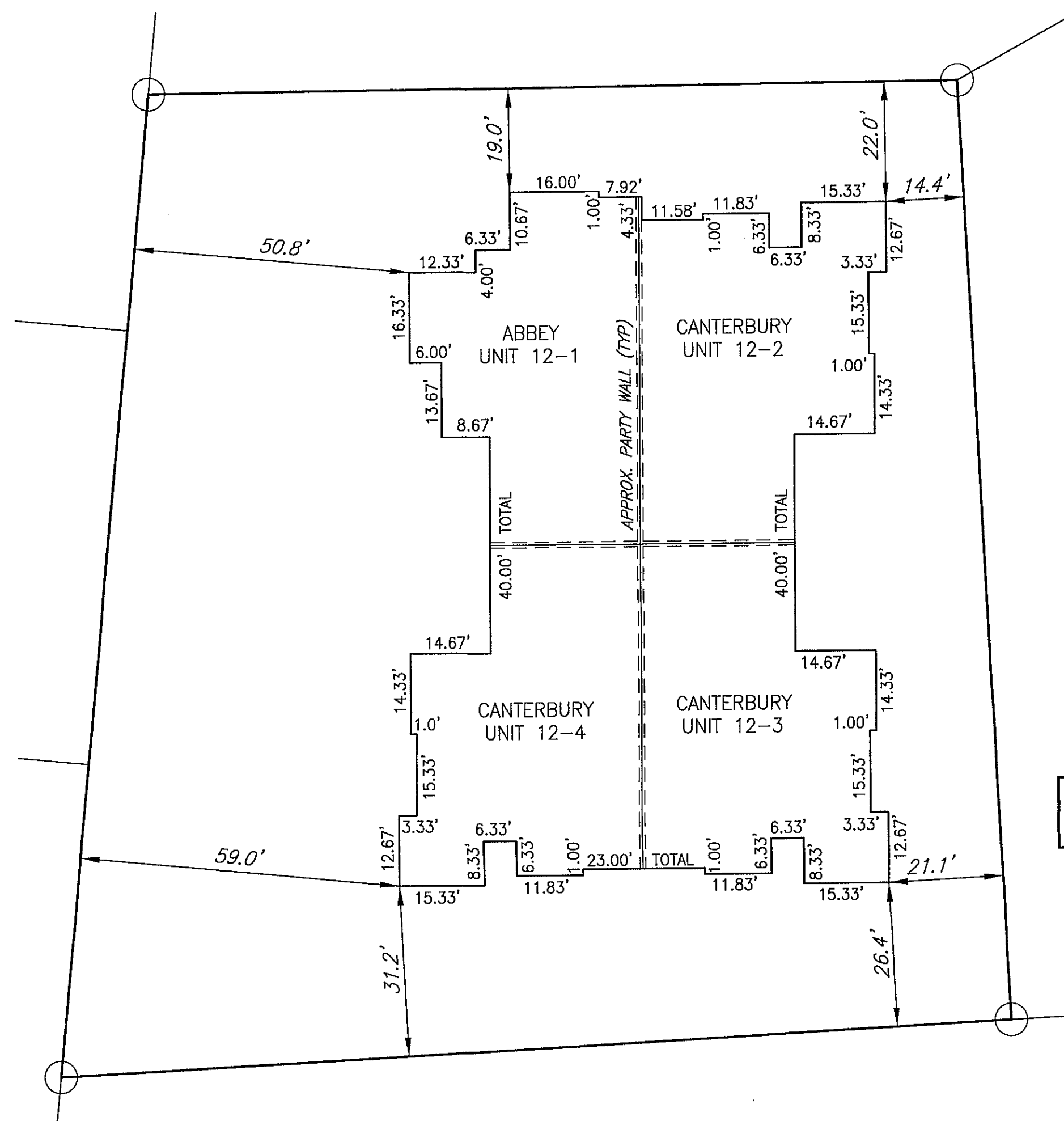
BUILDING 12 DETAIL NEW PHASE 10(A)
