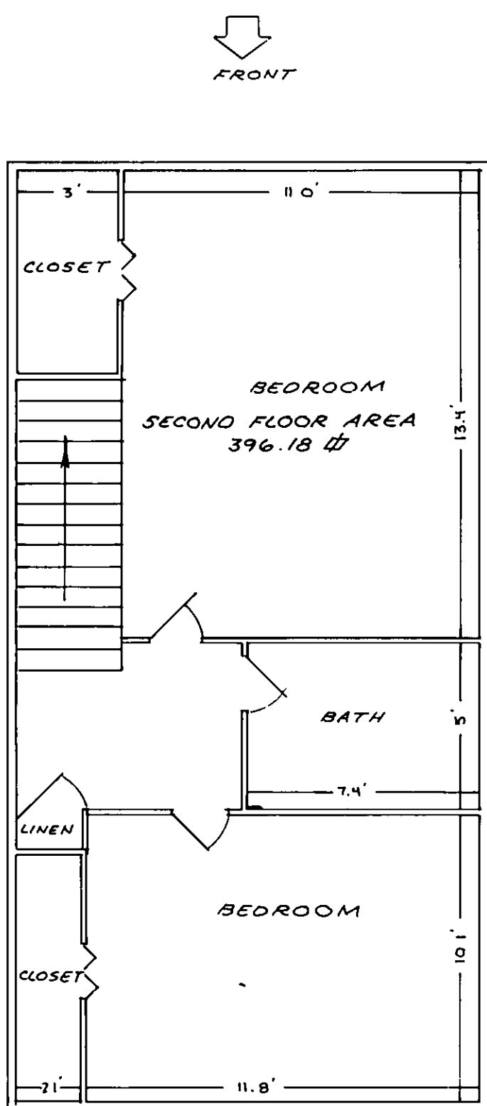
TYPICAL SECOND FLOOR
