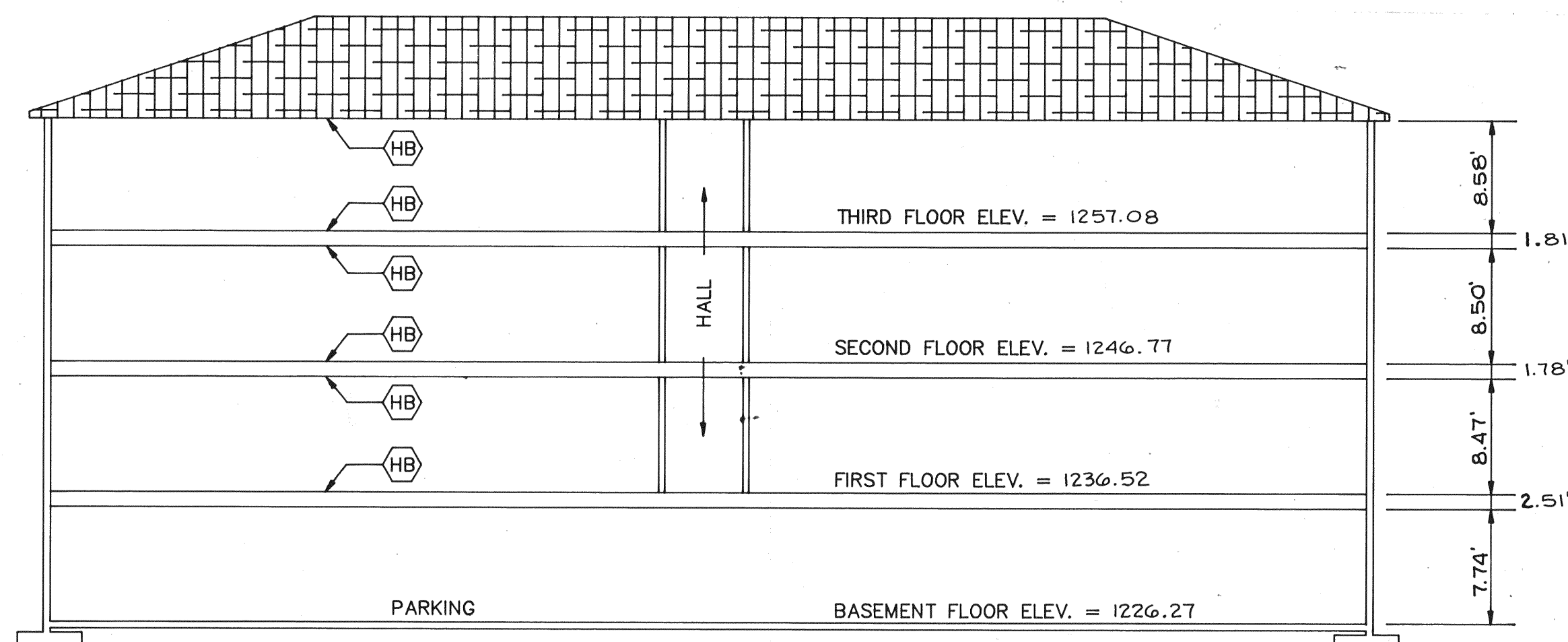
BUILDING NO. 1 ELEVATION
