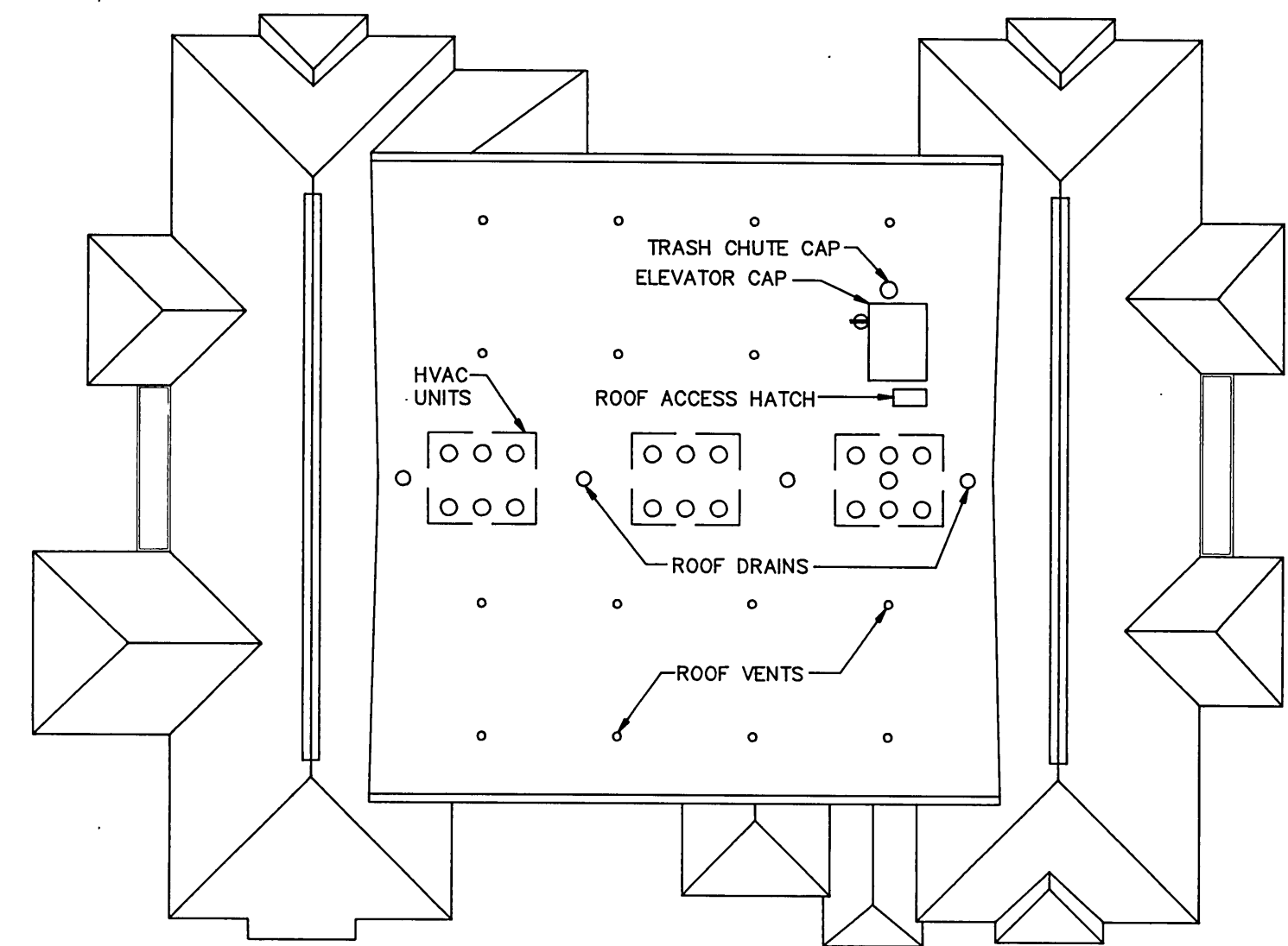
ROOF
