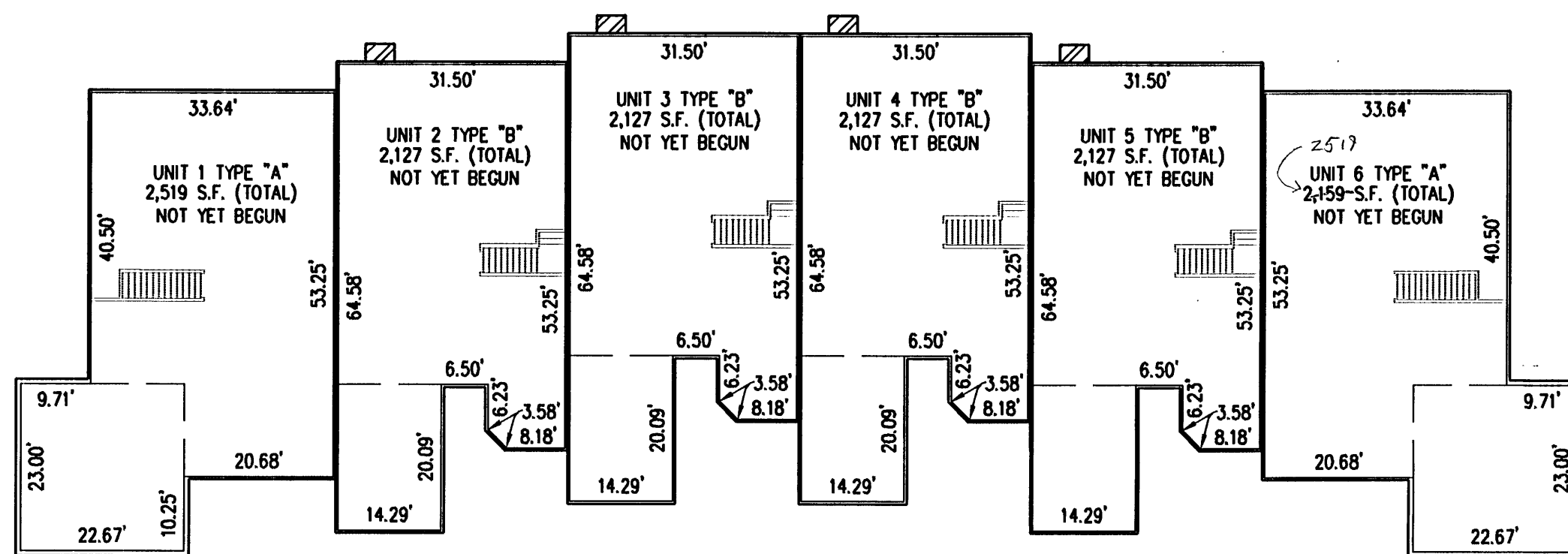
FIRST FLOOR UNITS 1 - 6
