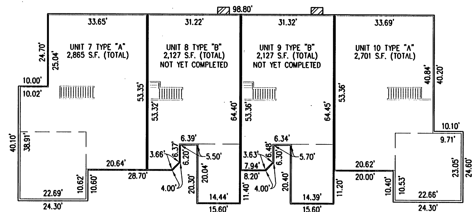
FIRST FLOOR UNITS 7 - 10
