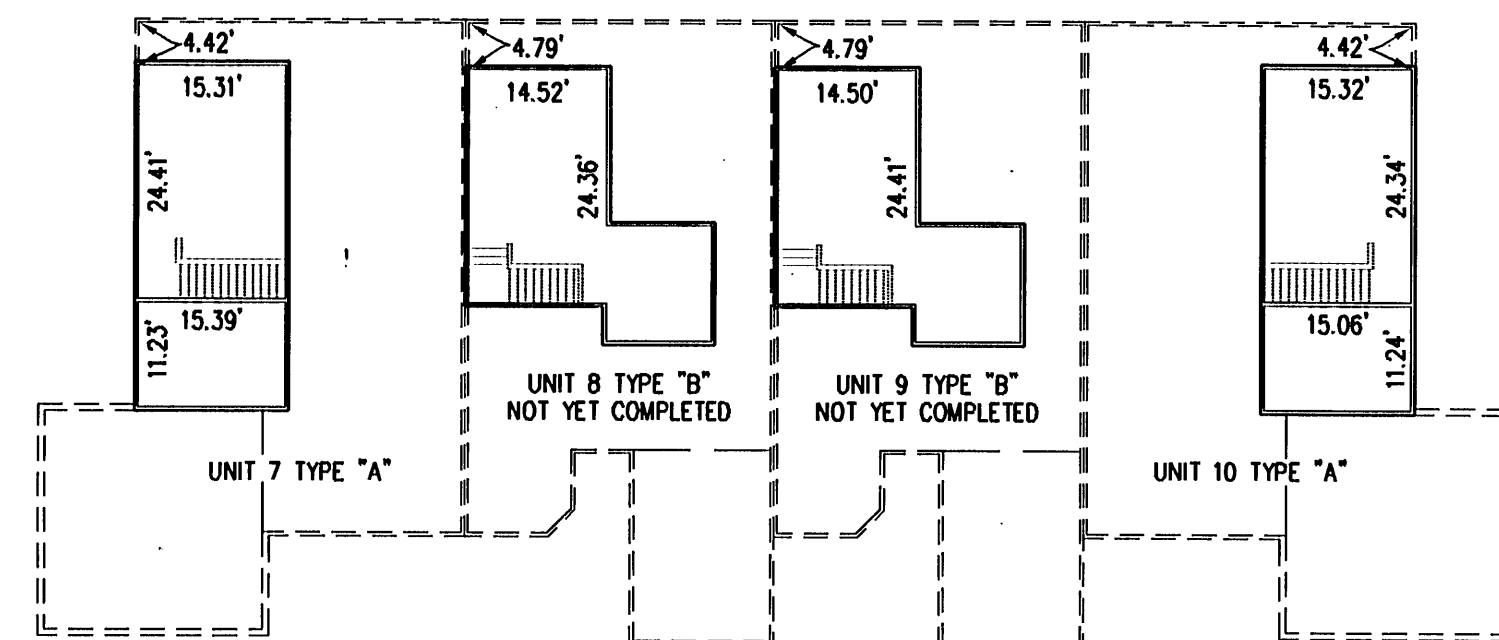
SECOND FLOOR UNITS 7 - 10
