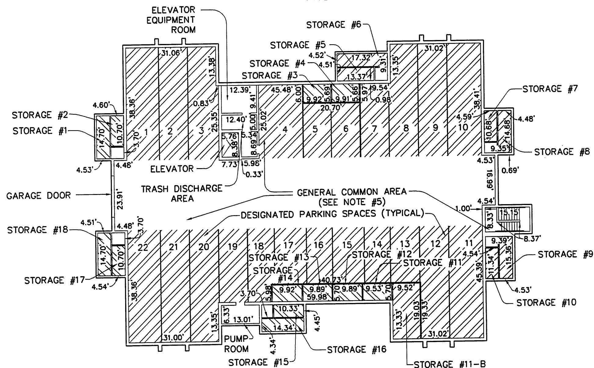
BASEMENT FLOOR
