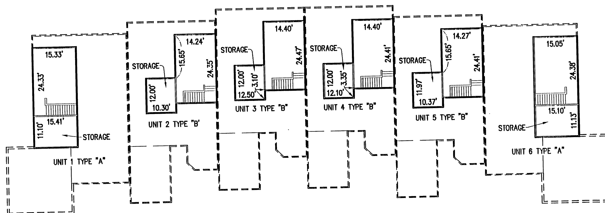
SECOND FLOOR UNITS 1 - 6
