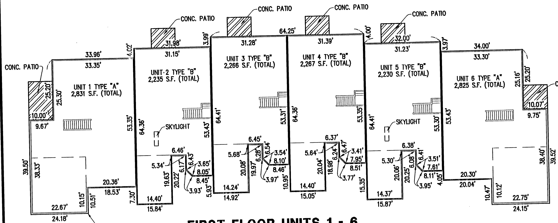
FIRST FLOOR UNITS 1 - 6
