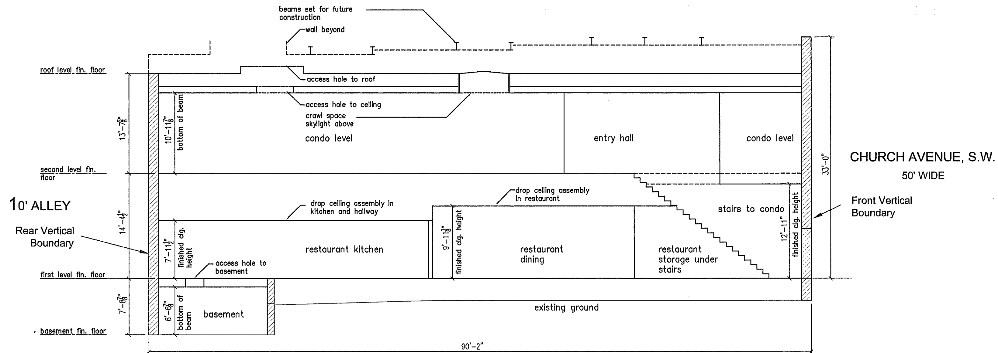
TYPICAL SECTION
