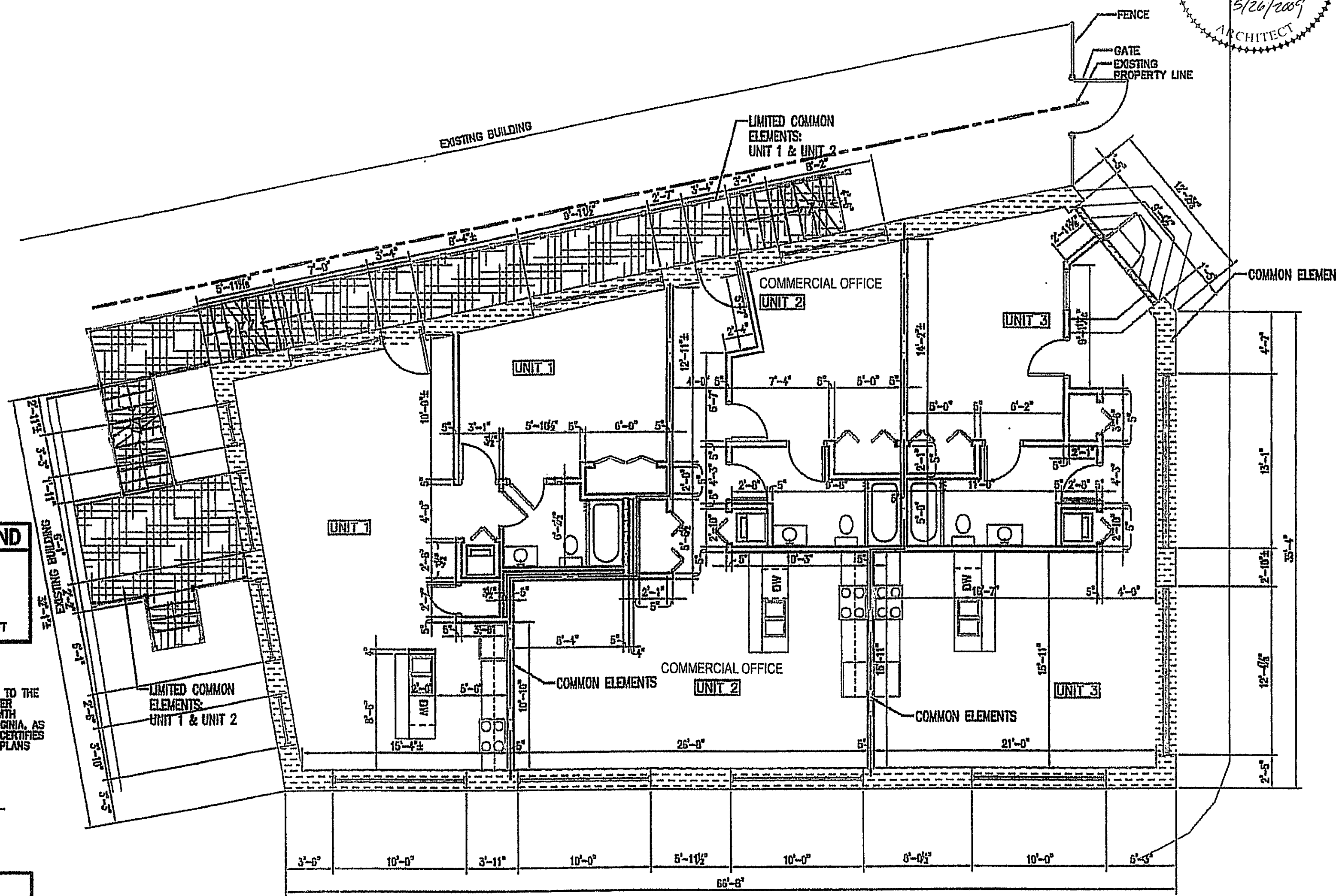
NEW WORK PLAN—MAIN LEVEL 1/4"=1'-0"
