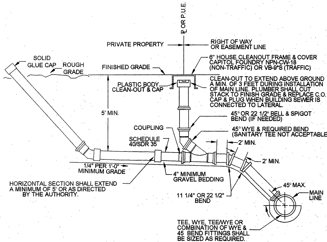
SANITARY SEWER LATERAL FOR DEEP SEWER
