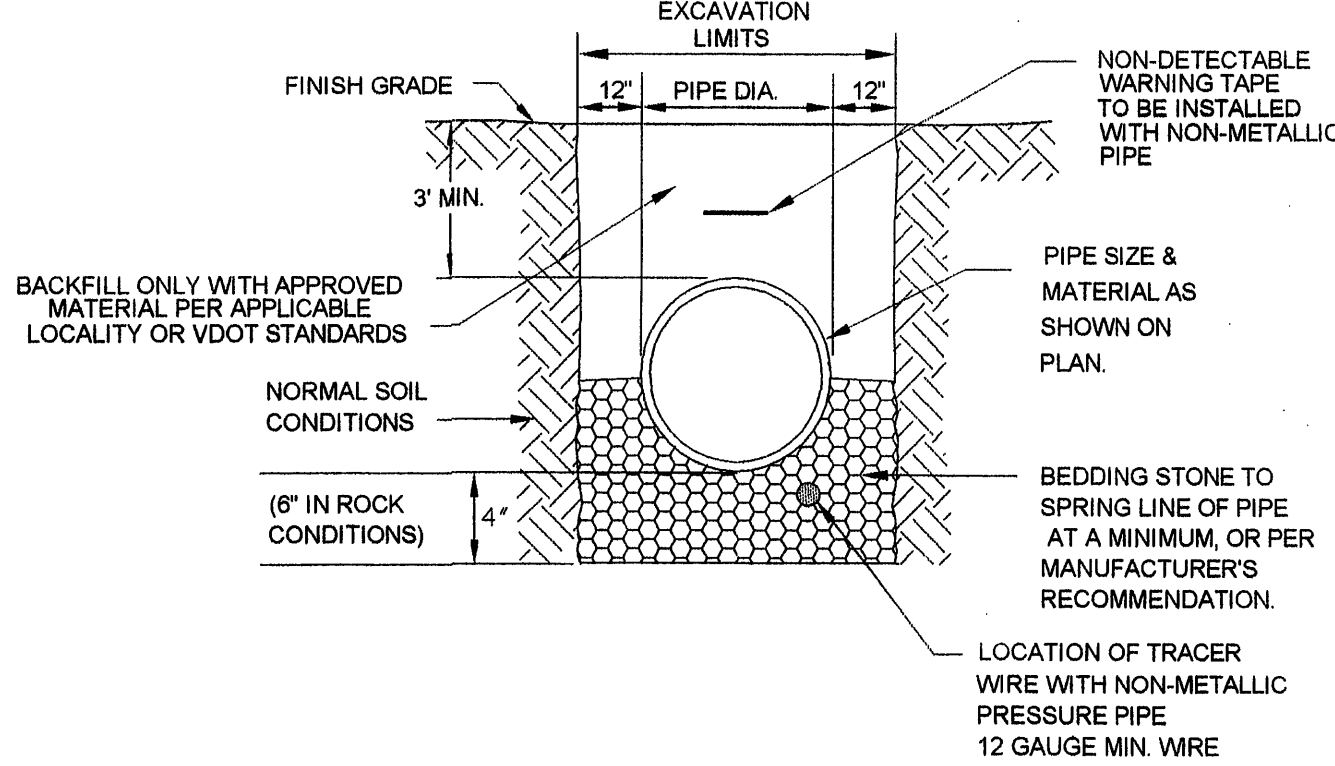
BEDDING AND BACKFILL OUTSIDE OF PAVED AREAS
