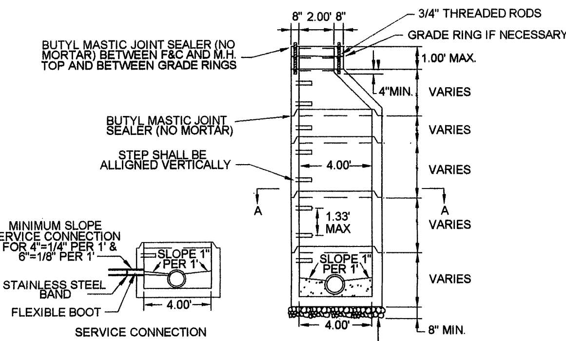
4' STANDARD MANHOLE FOR PIPE 15" OR SMALLER NOT TO SCALE
