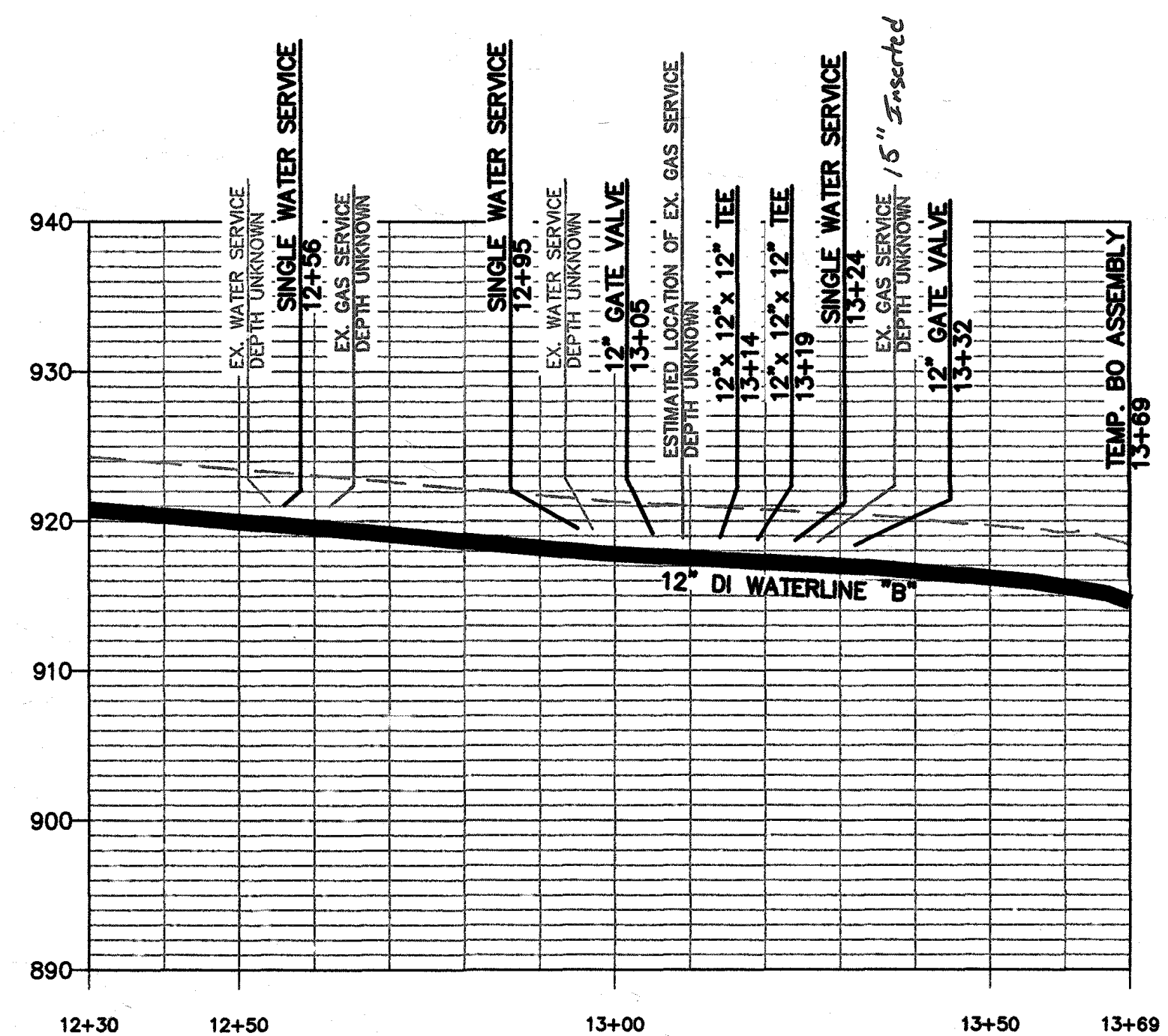
WATERLINE "B" SCALE VERTICAL: 1" = 10' HORIZONTAL: 1" = 20'
