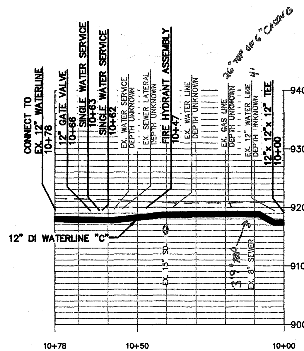
WATERLINE "C" SCALE VERTICAL: 1" = 10' HORIZONTAL: 1" = 20'
