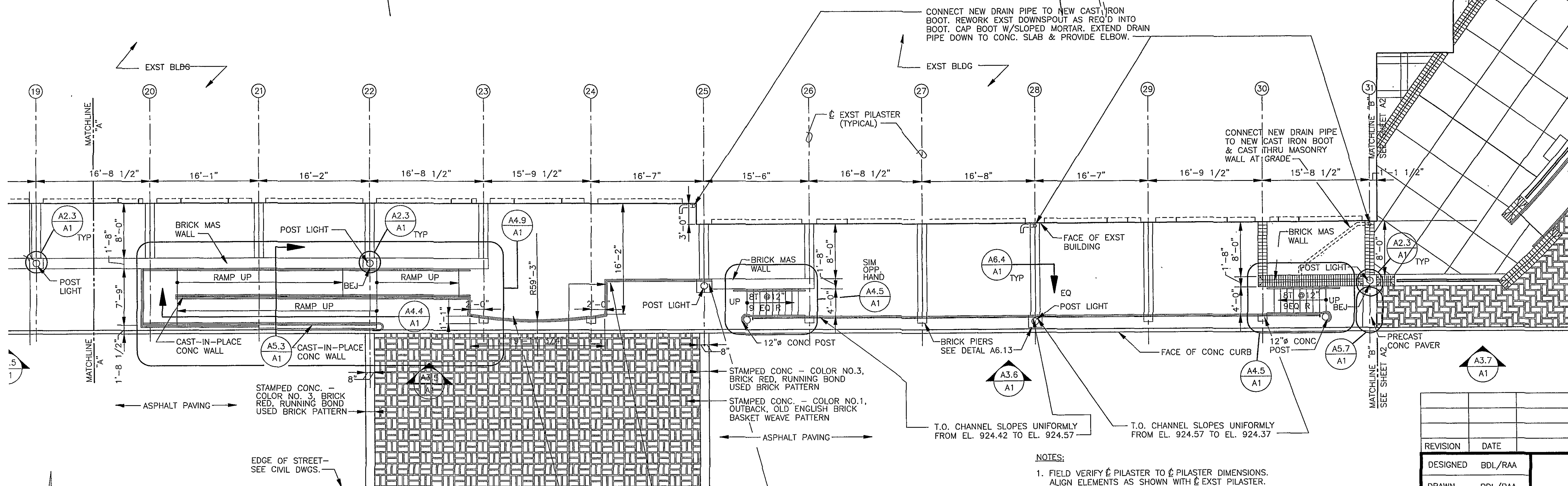
PARTIAL PLAN EAST-ELEVATED WALK
