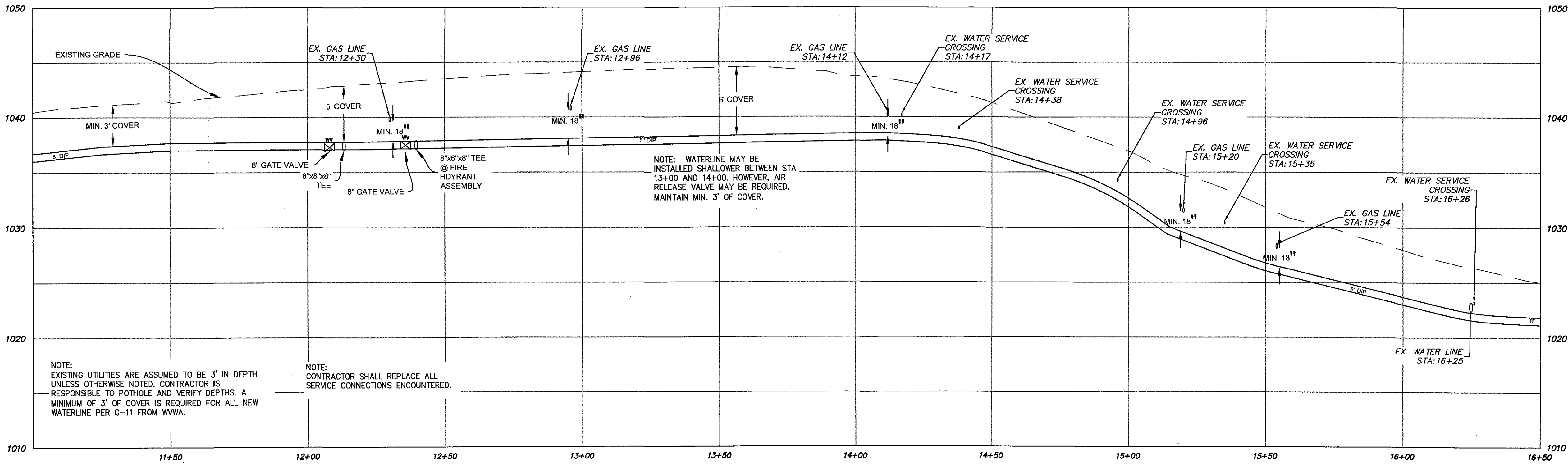
WINDSOR AVE SW WATERLINE STA 11+00 - 16+50 PROFILE 1" = 20' Horizontal 1" = 5' Vertical
