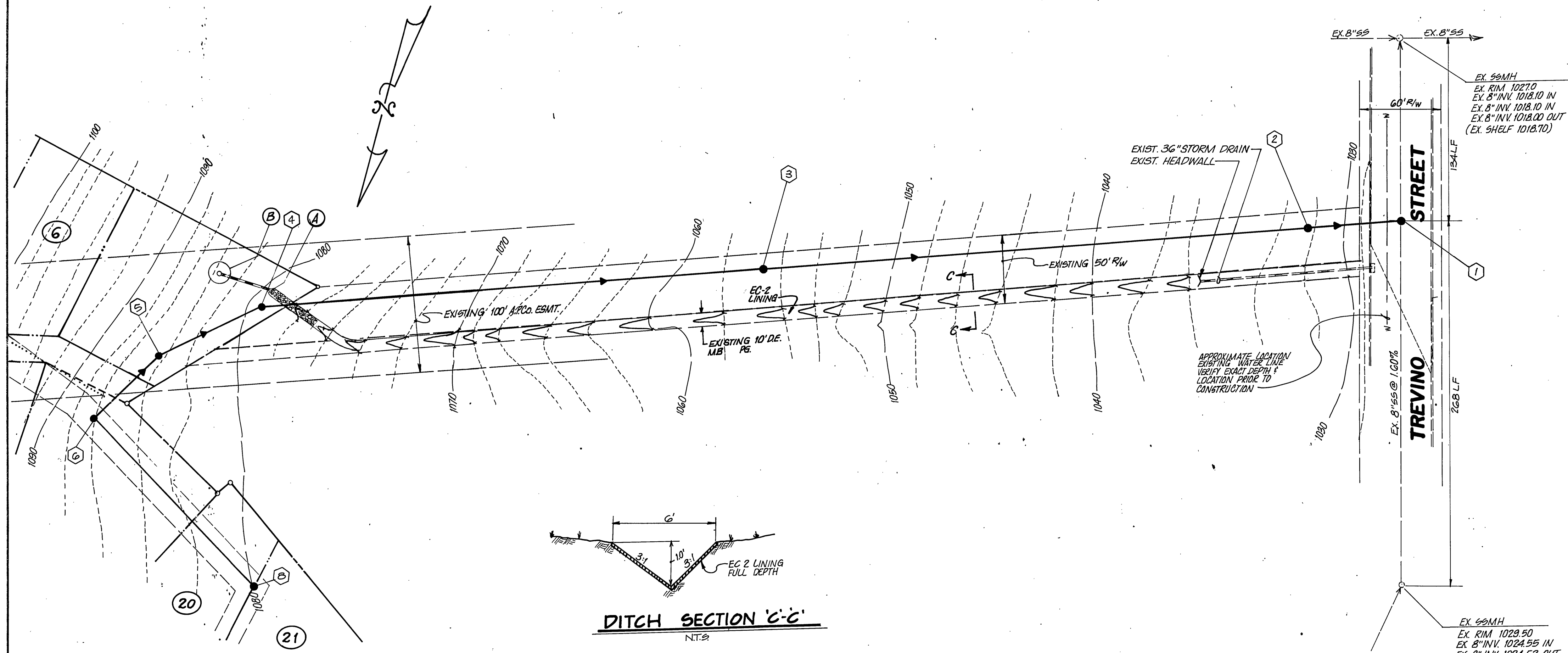
PLAN SCALE: 1"=50'
