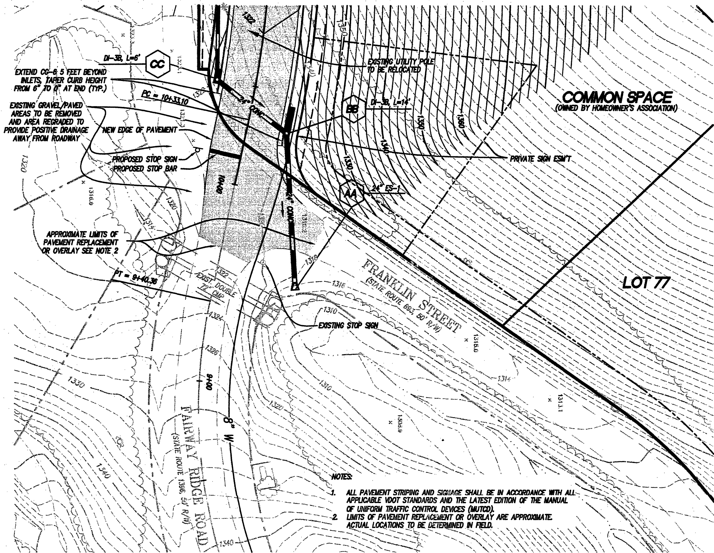
INTERSECTION DETAIL
