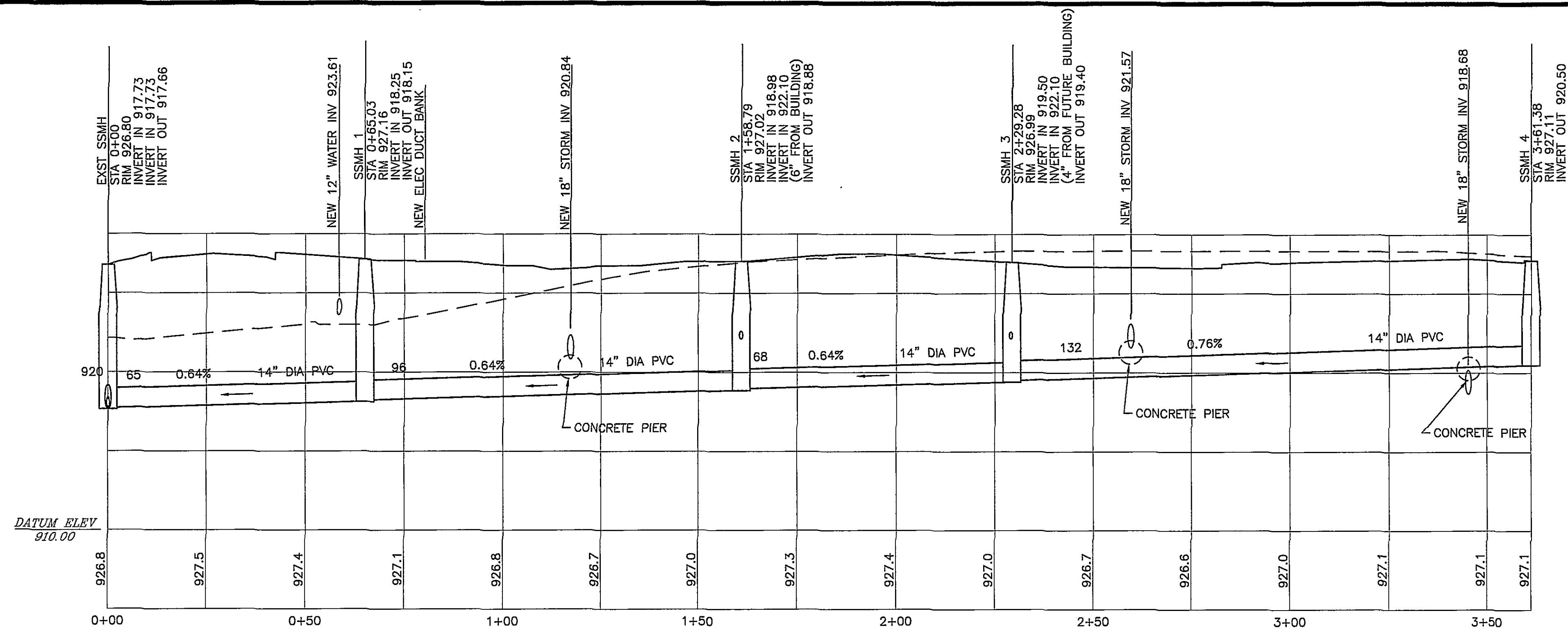
SANITARY SEWER PROFILE SCALE: HORIZ.: 1"=20'-0" VERT.: 1"=5'-0"
