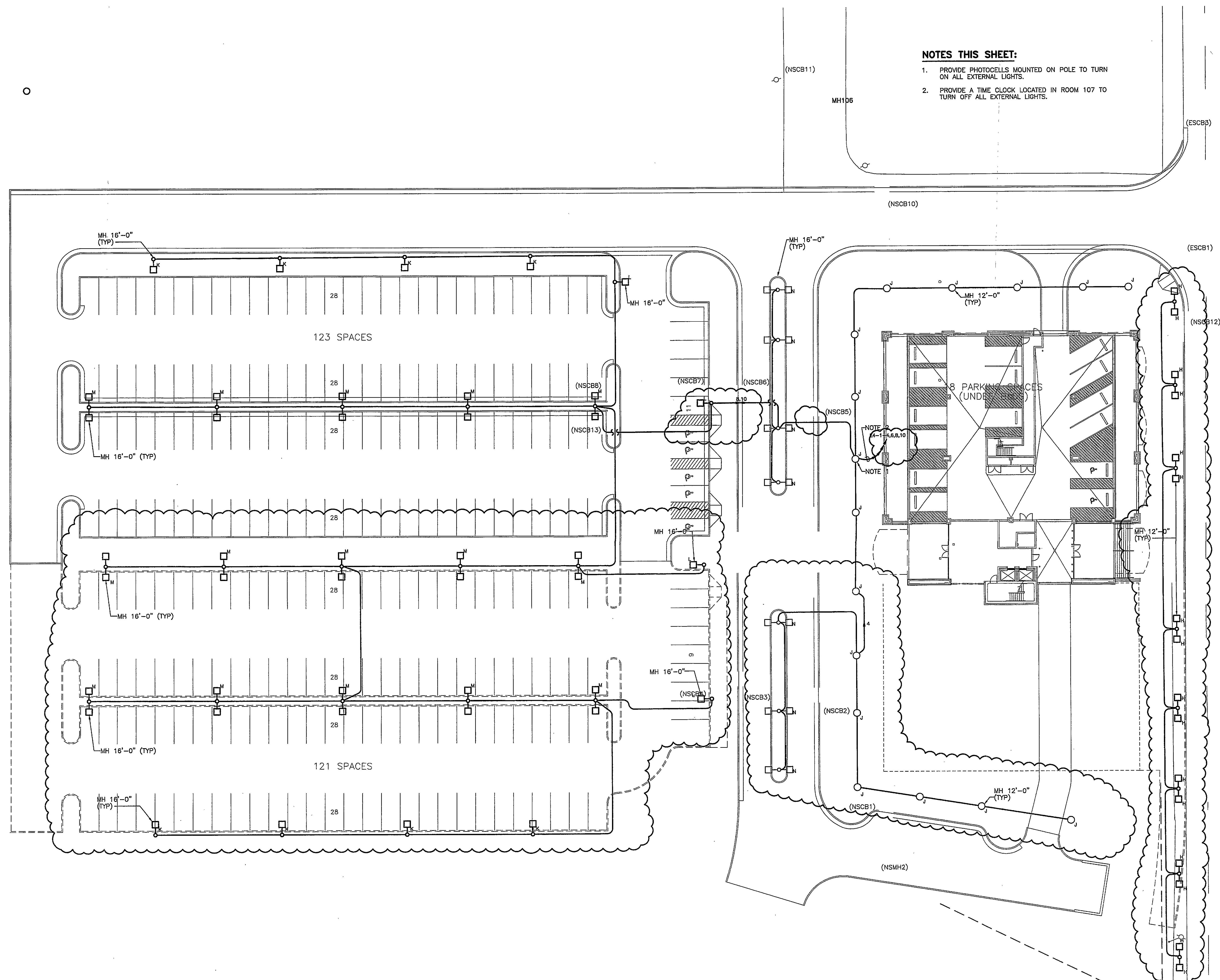
ELECTRICAL SITE LIGHTING PLAN SCALE: 1"=20'
