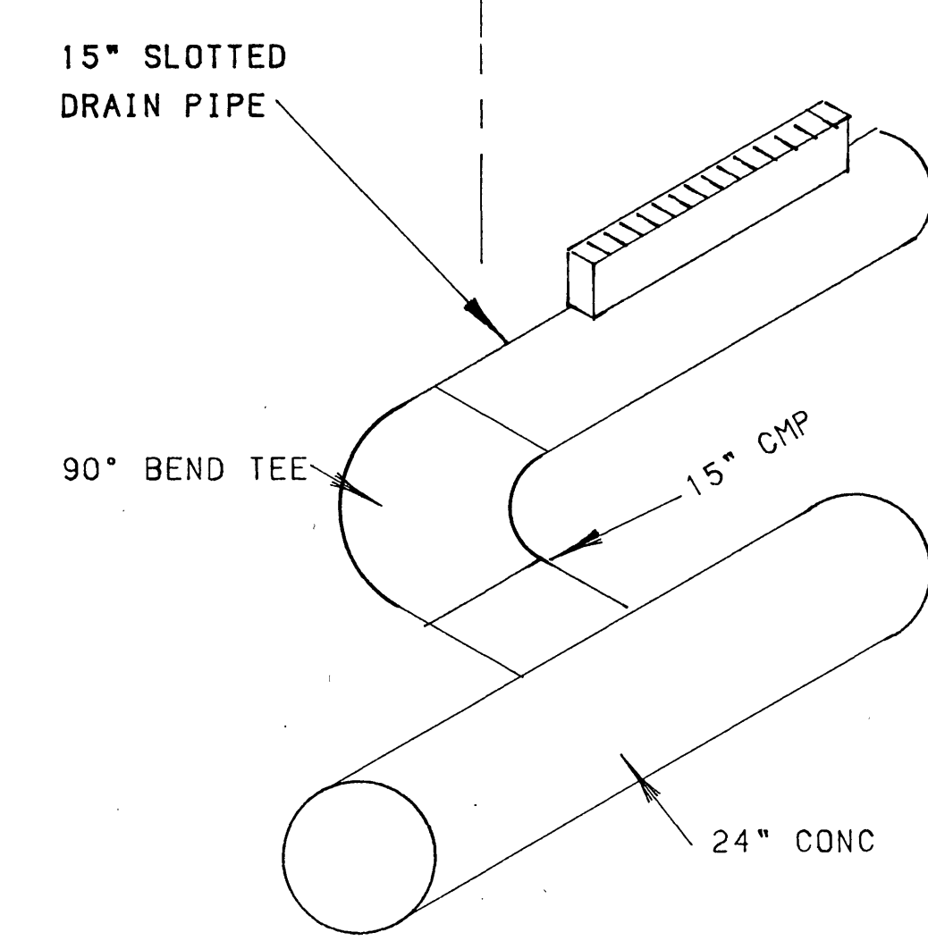
SLOTTED DRAIN PIPE ISOMETRIC NO SCALE
