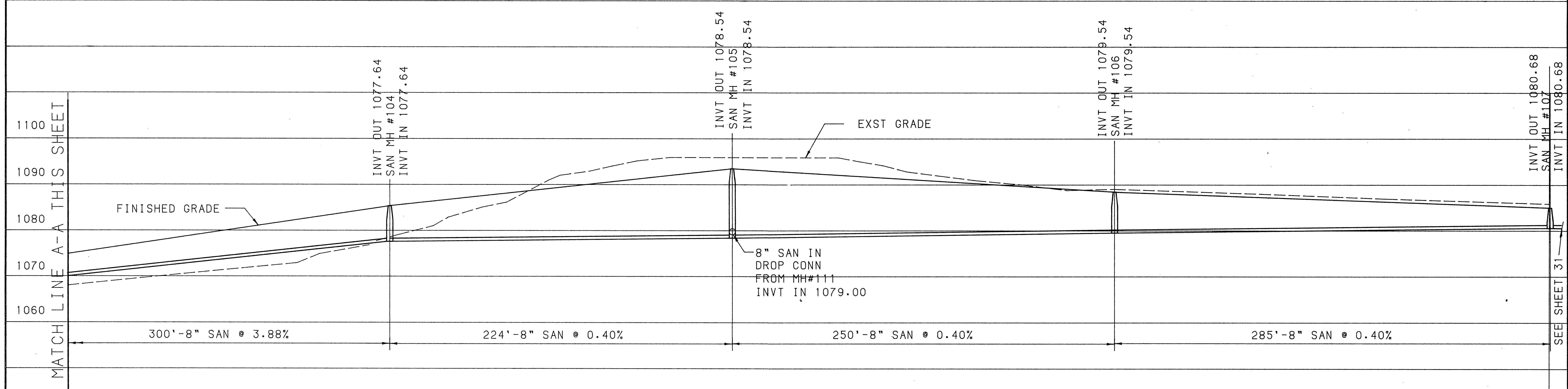
PROFILE- 8" SANITARY ALONG ROAD A - NIC TO MANHOLE # 103
