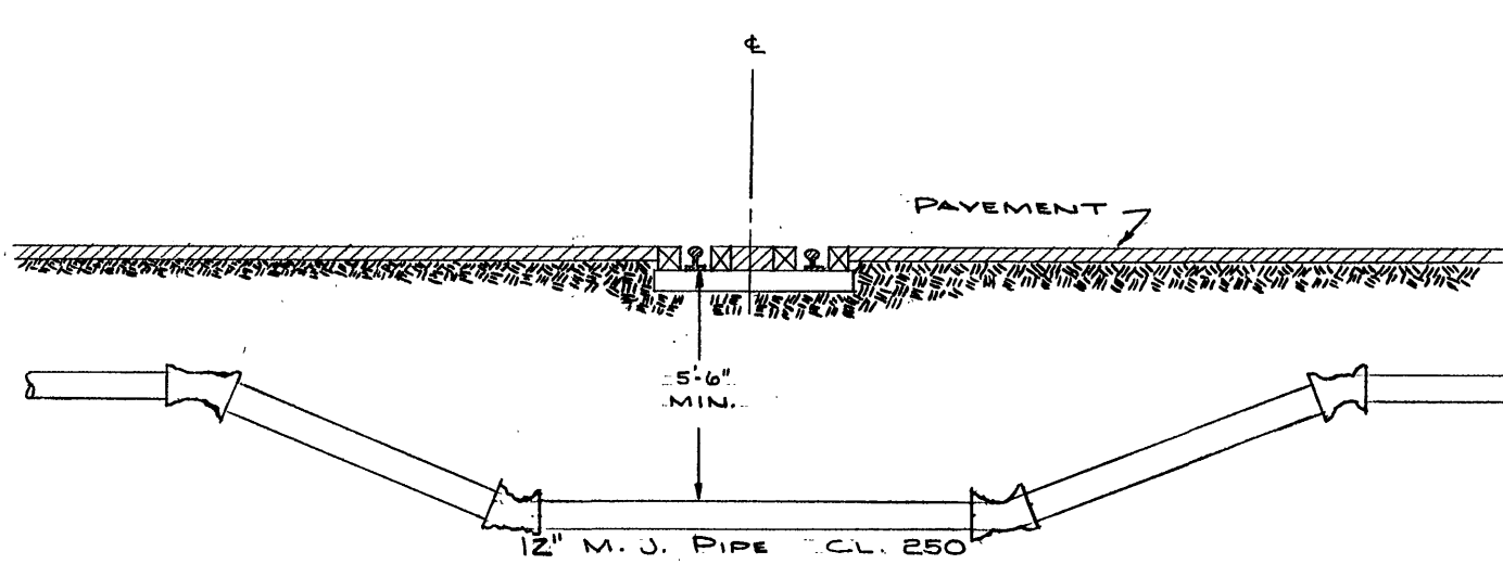
TYPICAL R.R. SIDING CROSSING SCALE - 1"=5'
