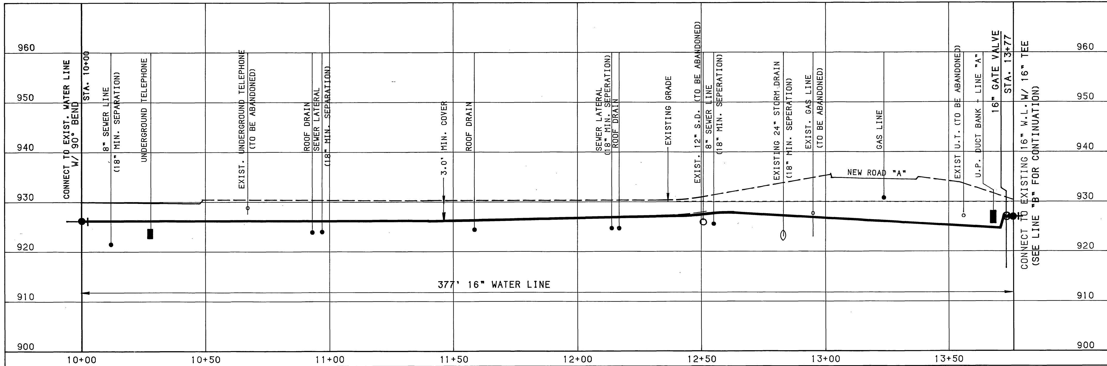
WATER LINE PROFILE "LINE A" SCALE: 1" = 20' HORIZ. 1" = 10' VERT.
