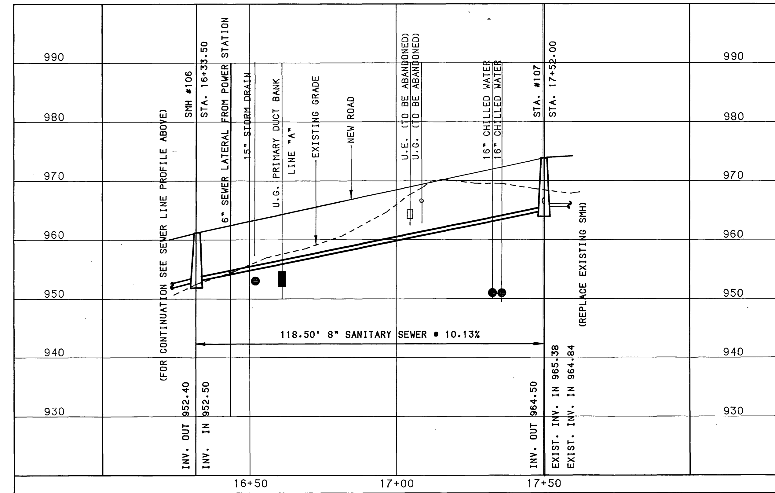
SEWER LINE PROFILE SCALE: 1" = 20' HORIZ. 1" = 10' VERT.
