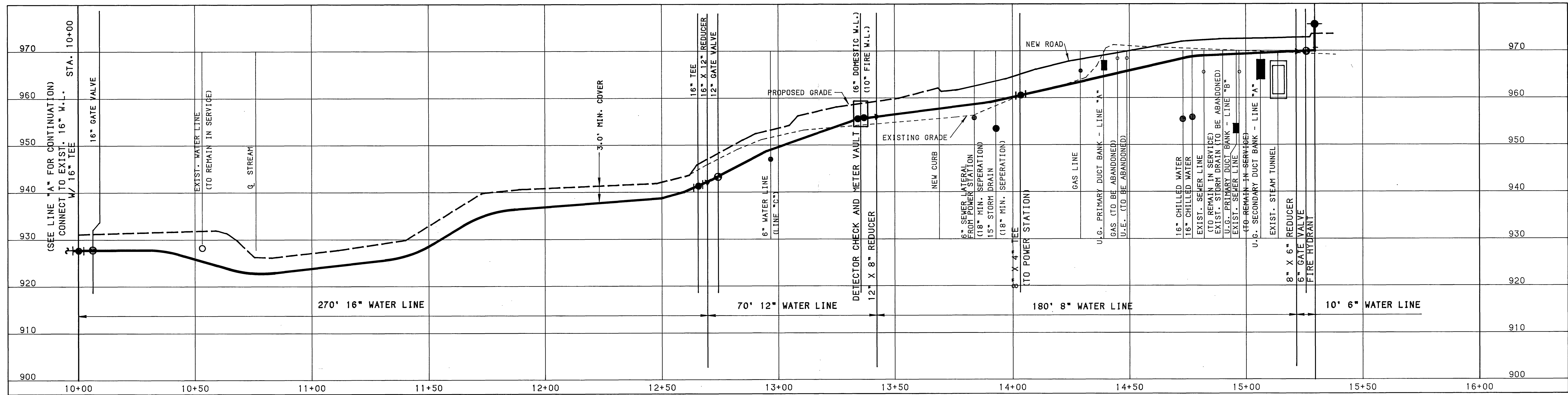
WATER LINE PROFILE "LINE B" SCALE: 1" = 20' HORIZ. 1" = 10' VERT.
