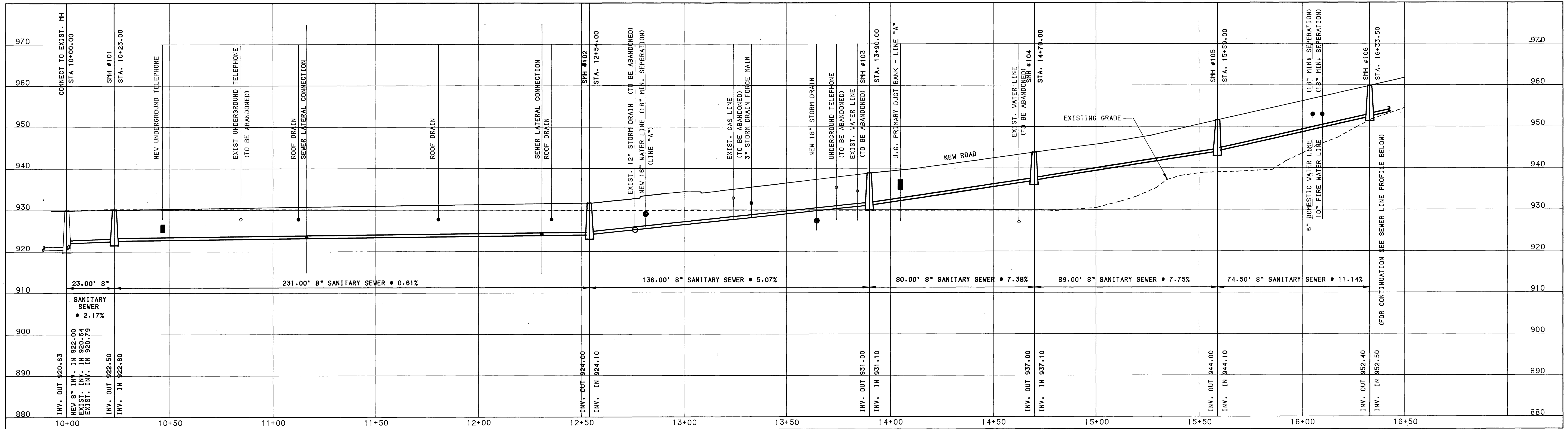
SEWER LINE PROFILE SCALE: 1" = 20' HORIZ. 1" = 10' VERT.
