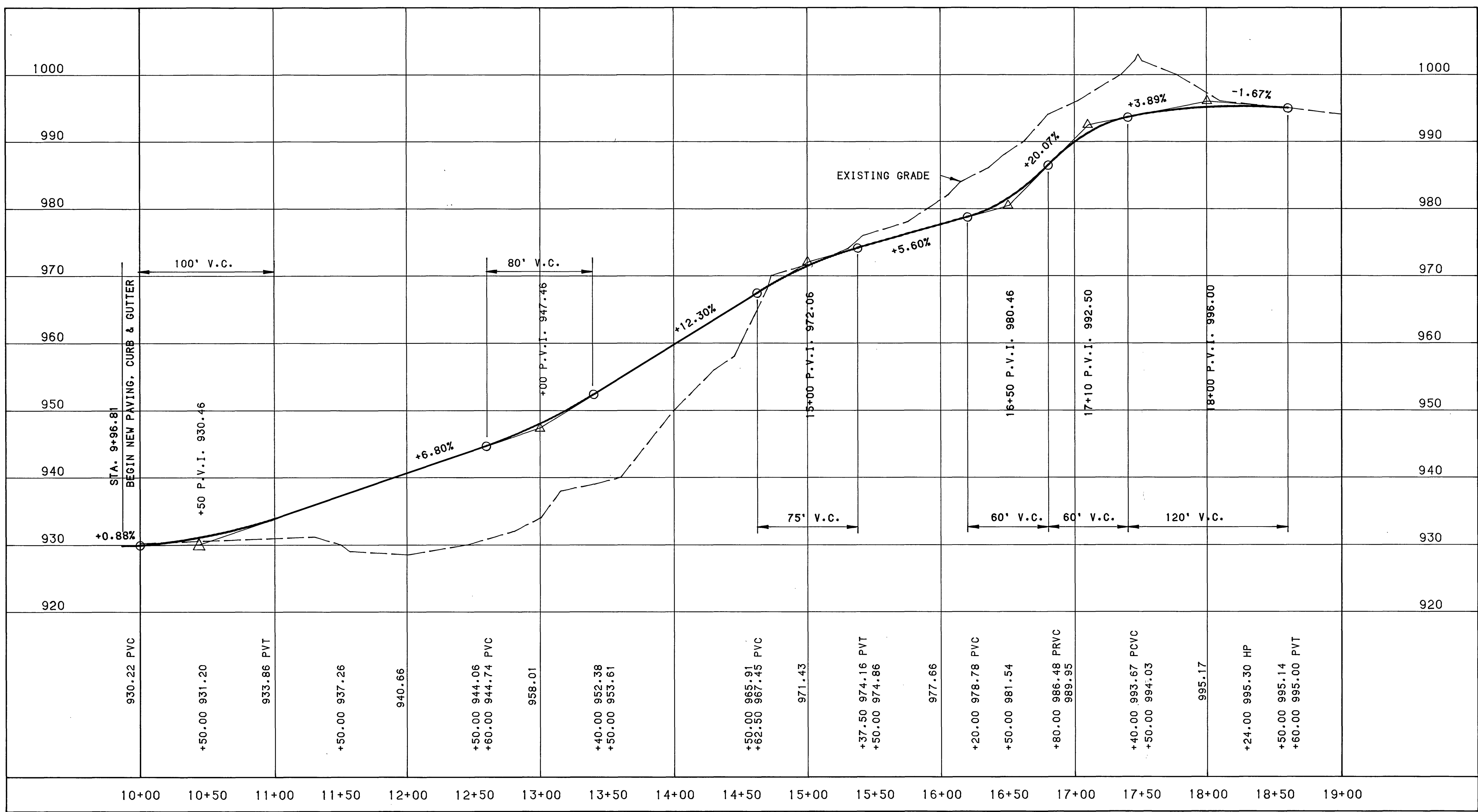
ROAD PROFILE - ROAD "A"
