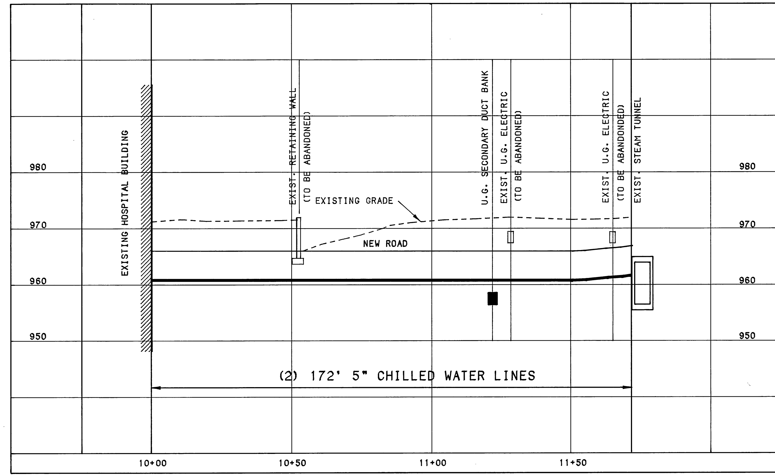
CHILLED WATER LINE PROFILE SCALE: 1" = 20' HORIZ. 1" = 10' VERT.
