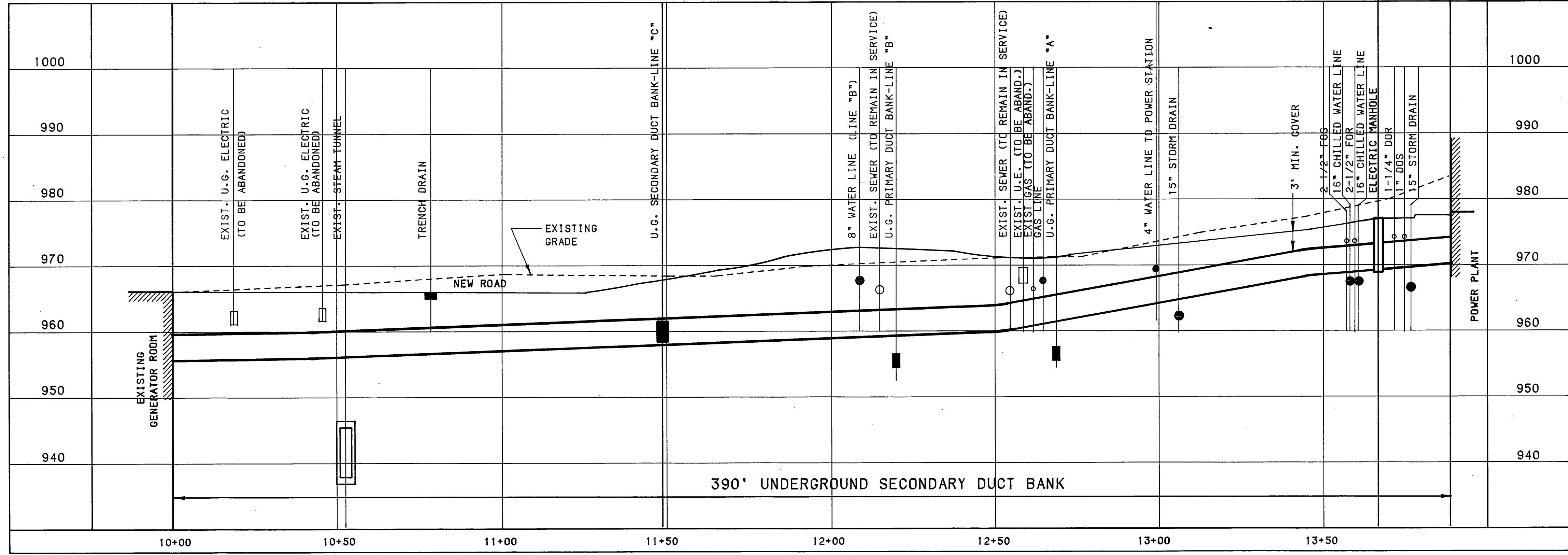
UNDERGROUND SECONDARY DUCT BANK PROFILE - LINE "A" SCALE: 1" = 20' HORIZ. 1" = 10' VERT.
