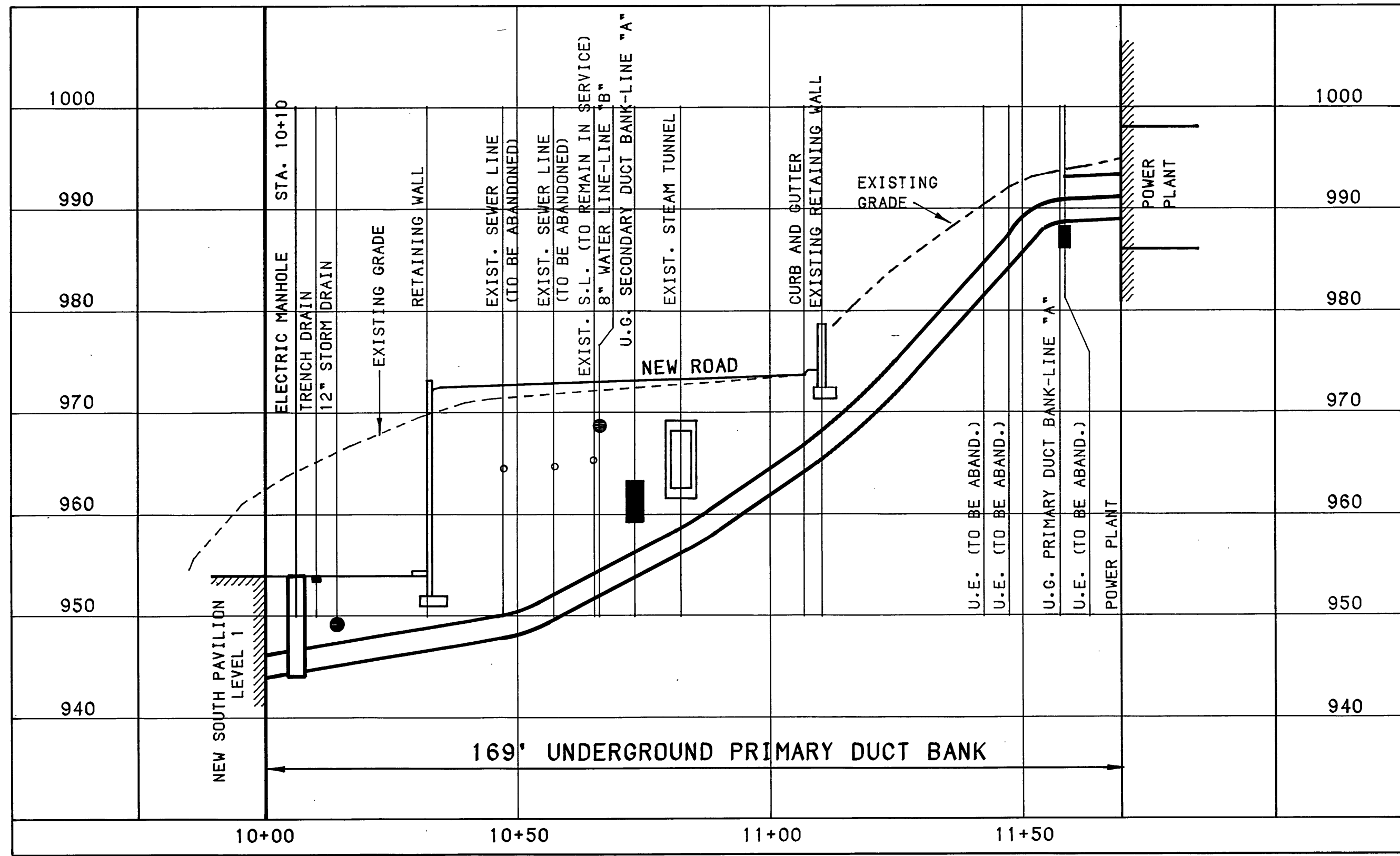
UNDERGROUND PRIMARY DUCT BANK PROFILE - LINE "B" SCALE: 1" = 20' HORIZ. 1" = 10' VERT.
