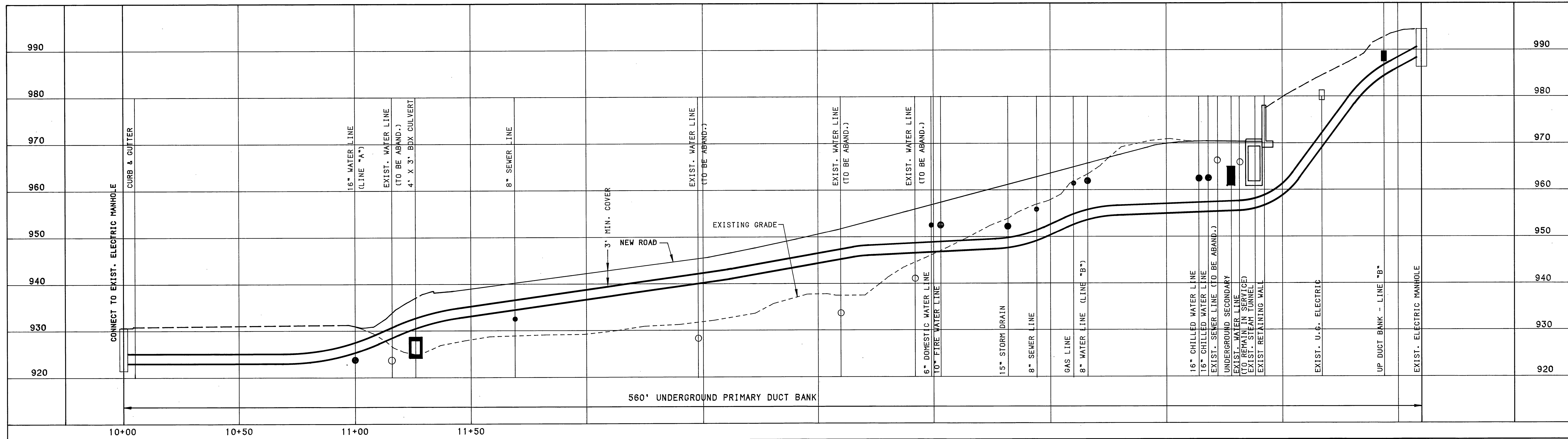
UNDERGROUND PRIMARY DUCT BANK PROFILE - LINE "A" SCALE: 1" = 20' HORIZ. 1" = 10' VERT.
