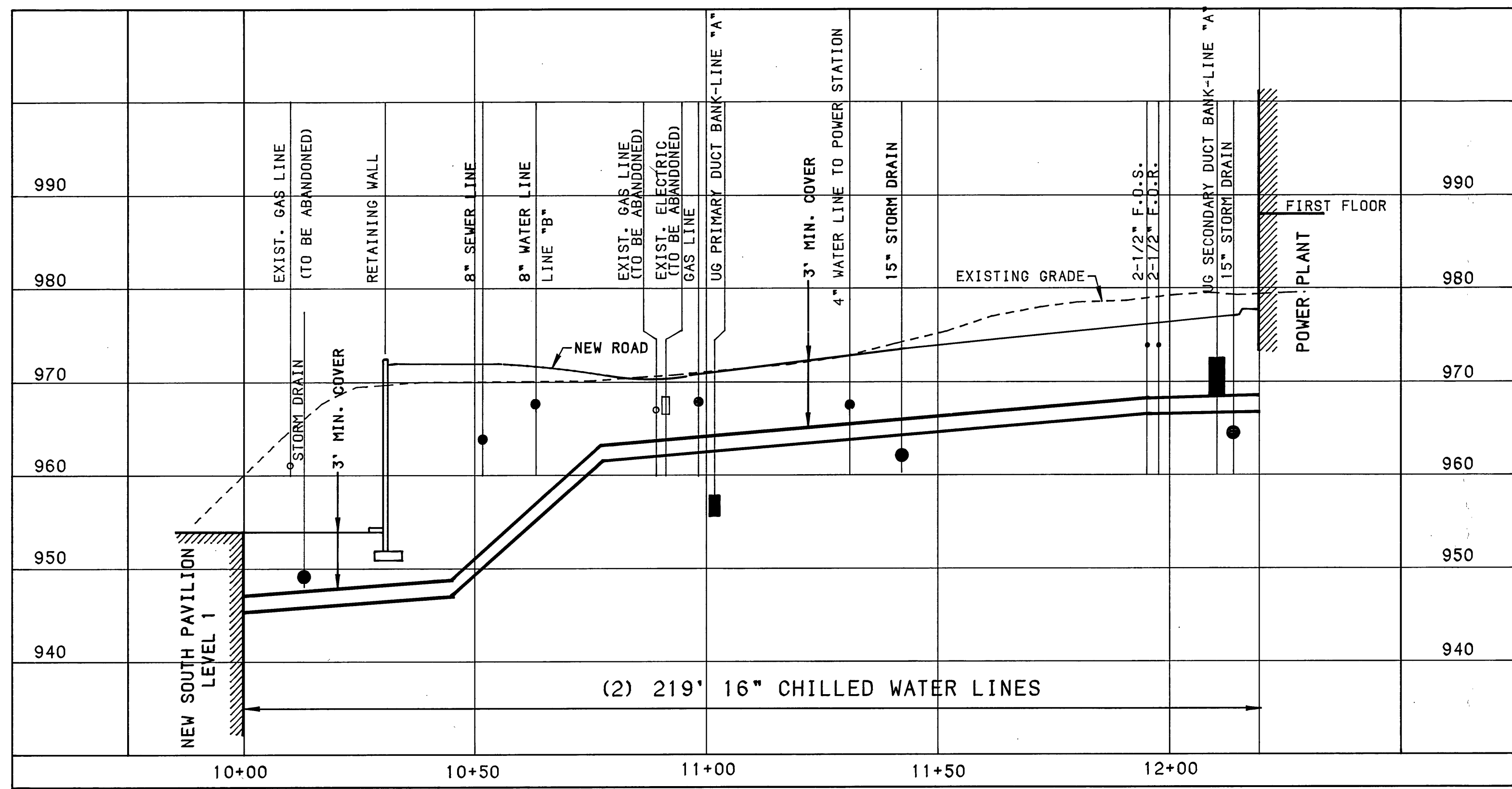
CHILLED WATER LINE PROFILE SCALE: 1" = 20' HORIZ. 1" = 10' VERT.
