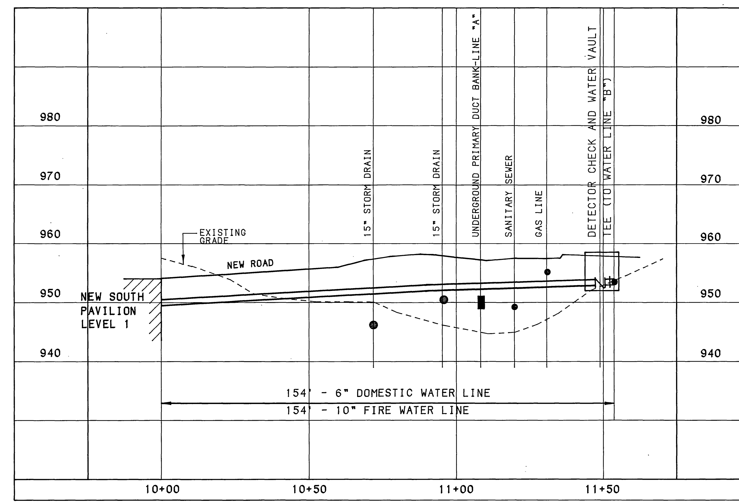
DOMESTIC AND FIRE WATER LINE PROFILES SCALE: 1" = 20' HORIZ. 1" = 10' VERT.
