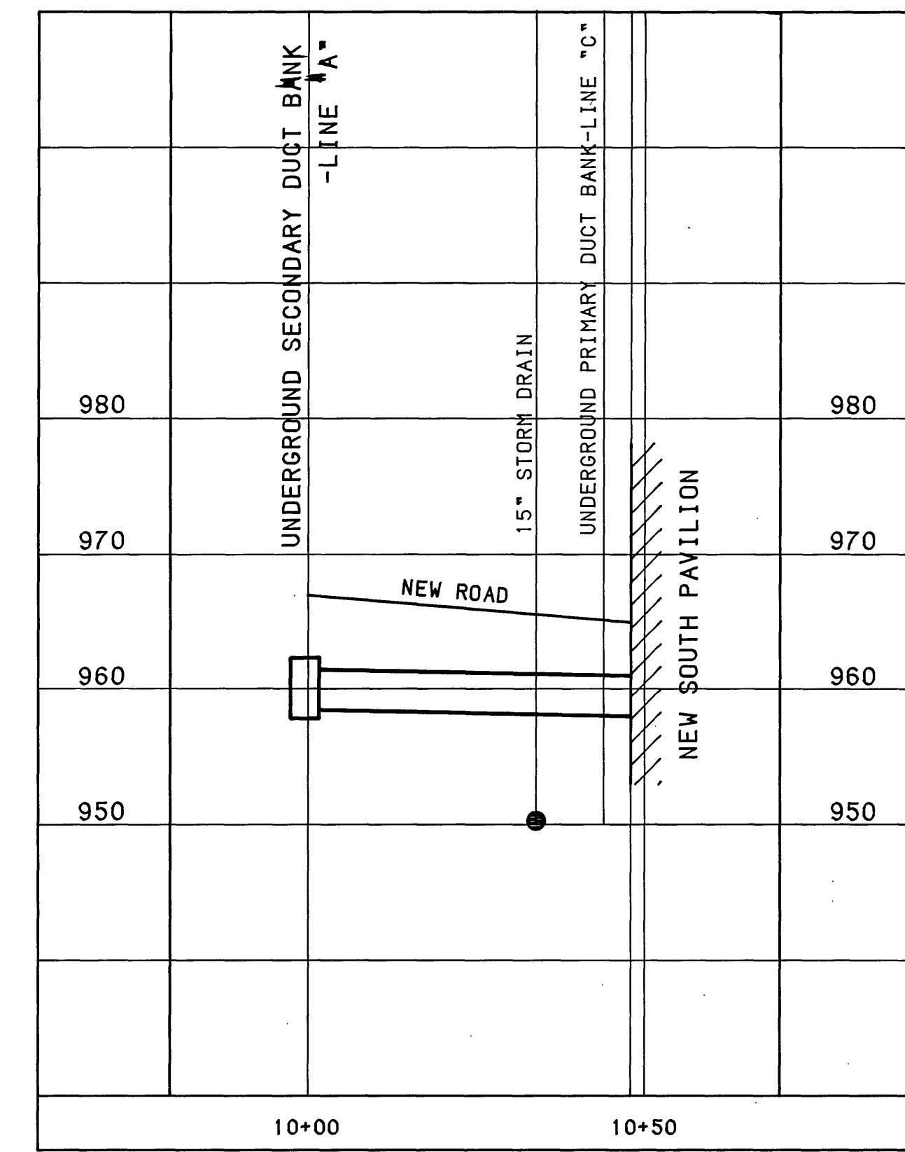
UNDERGROUND SECONDARY DUCT BANK SCALE: 1" = 20' HORIZ. 1" = 10' VERT.
