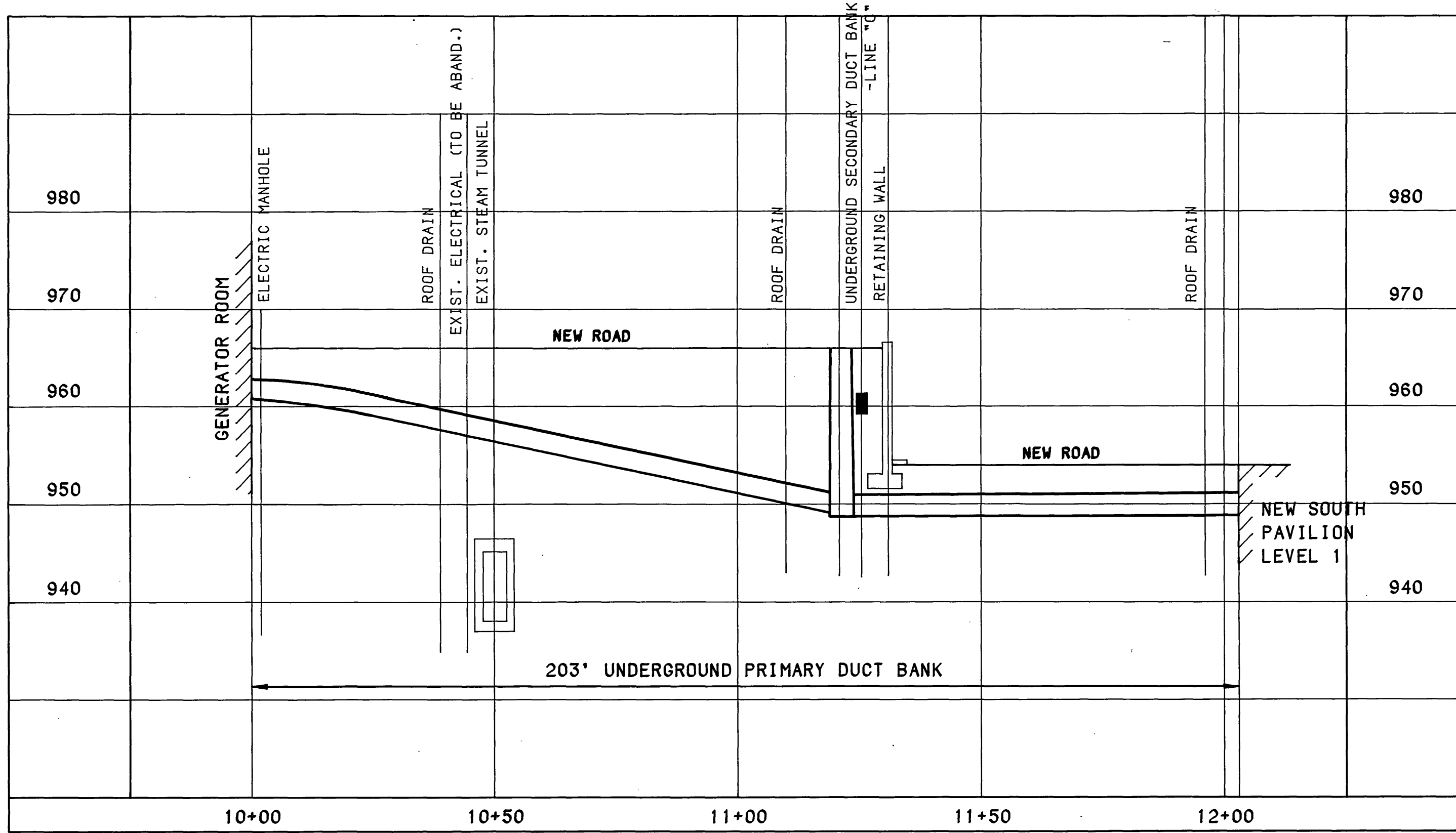
UNDERGROUND PRIMARY DUCT BANK - LINE "C" SCALE: 1" = 20' HORIZ. 1" = 10' VERT.
