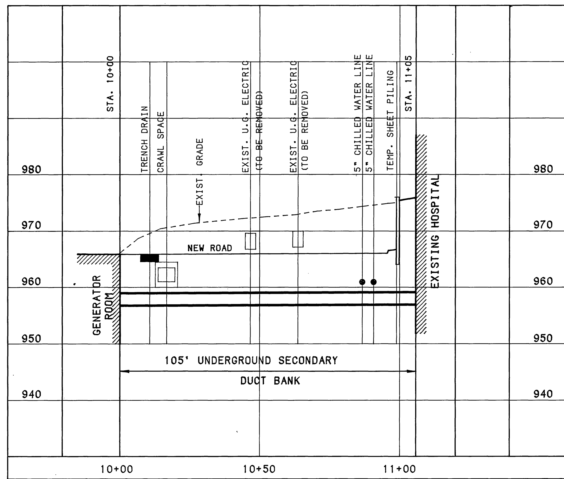
UNDERGROUND SECONDARY DUCT BANK - LINE "B" SCALE: 1" = 20' HORIZ. 1" = 10' VERT.
