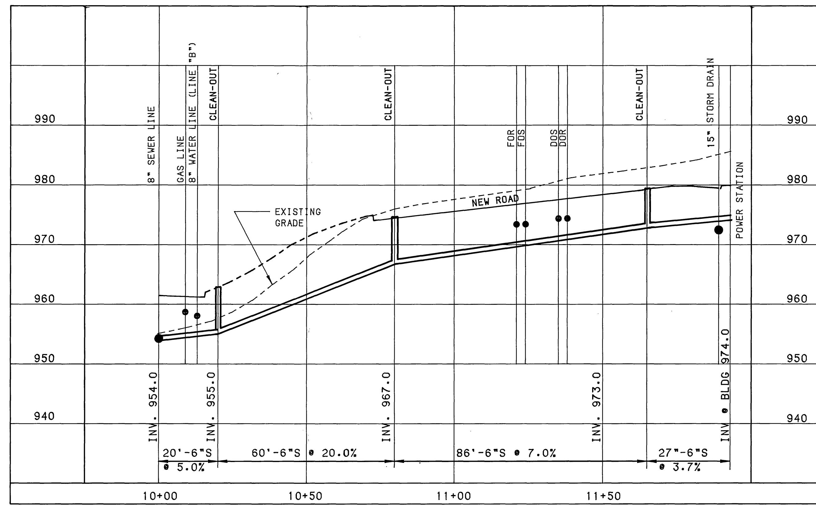
POWER PLANT SEWER LINE PROFILE SCALE: 1" = 20' HORIZ. 1" = 10' VERT.
