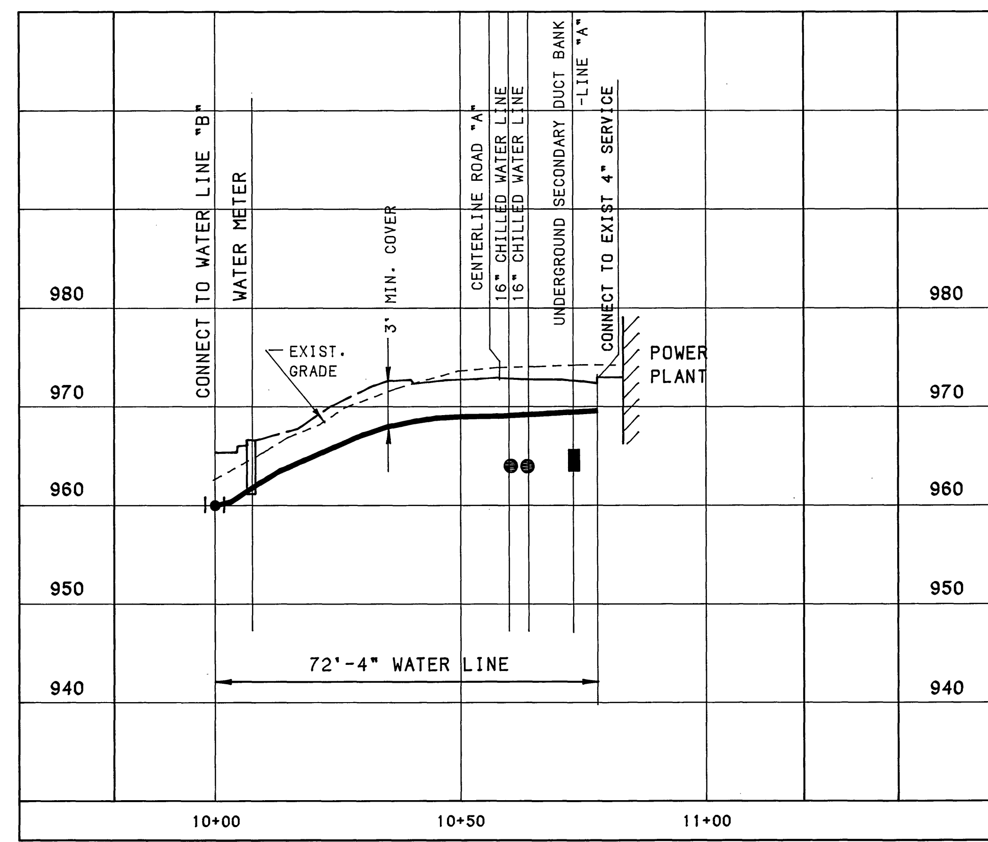
POWER PLANT WATER LINE PROFILE SCALE: 1" = 20' HORIZ. 1" = 10' VERT.
