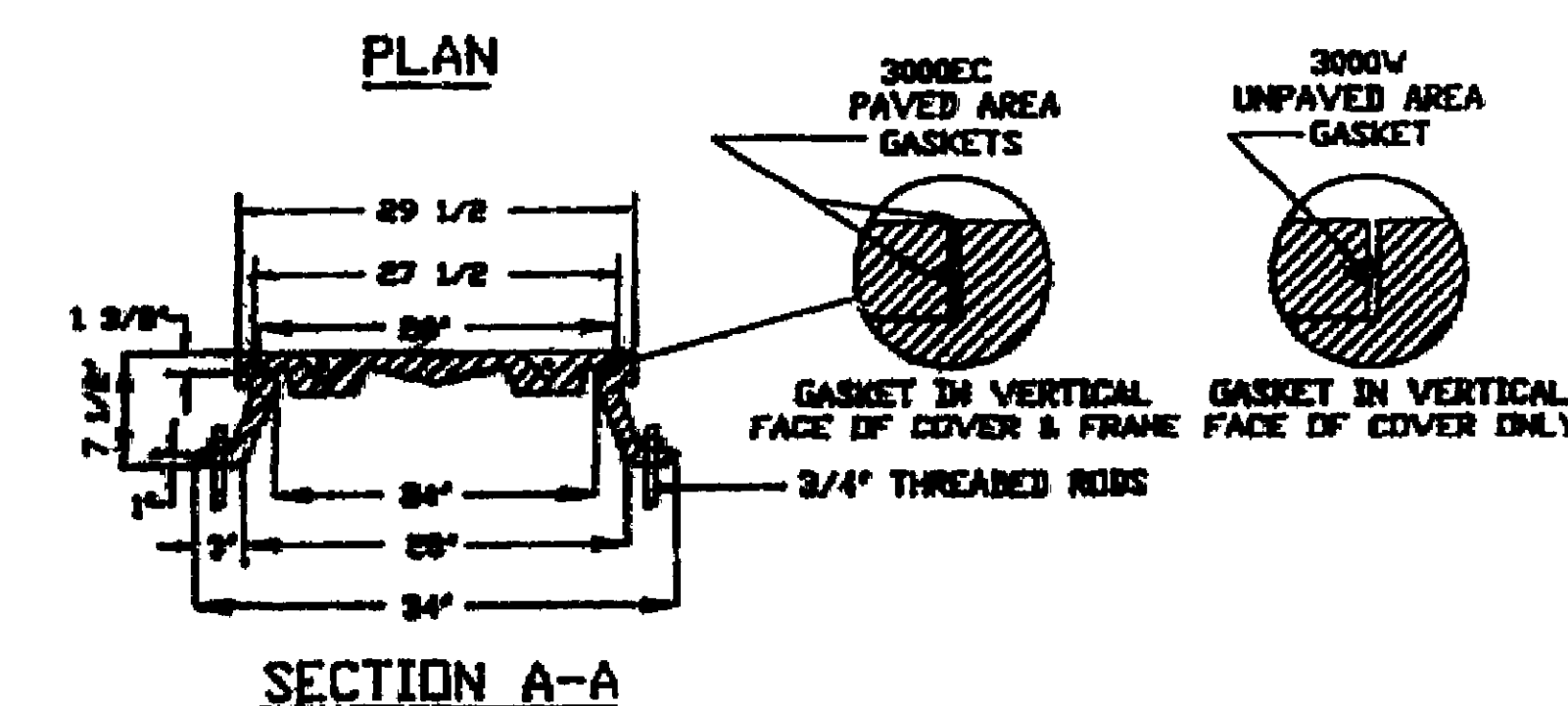
WATERTIGHT MANHOLE FRAME AND COVER
