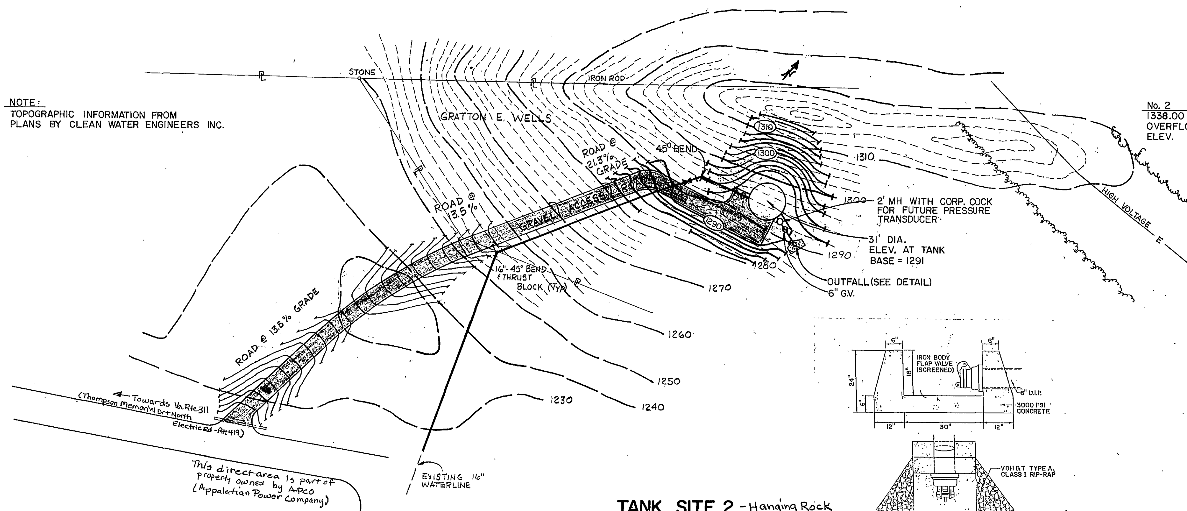
TANK SITE 2 - Hanging Rock SCALE: 1" = 50' T# 036.01-01-17.01-0000 1850 Loch Haven Dr.
