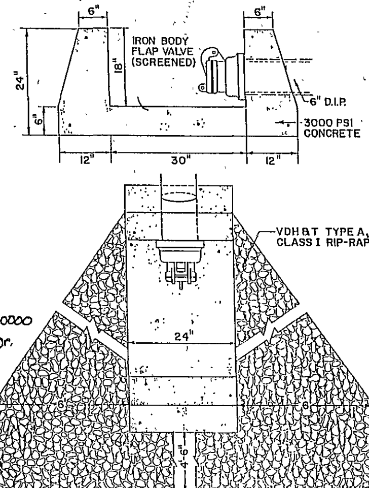
TANK DRAIN OUTFALL DETAIL NO SCALE
