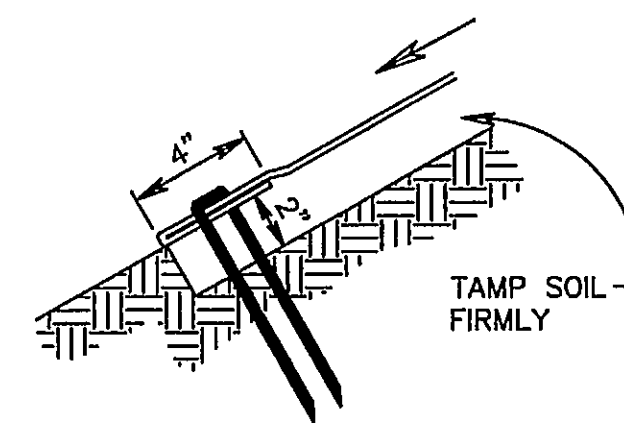
TERMINAL FOLD
