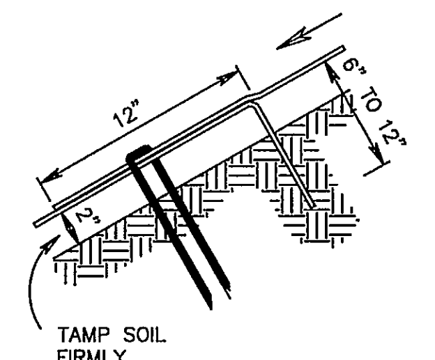
JUNCTION SLOT
