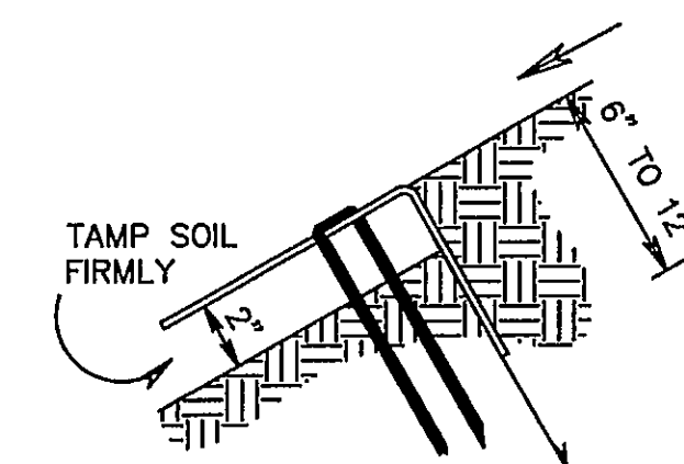
ANCHOR SLOT
