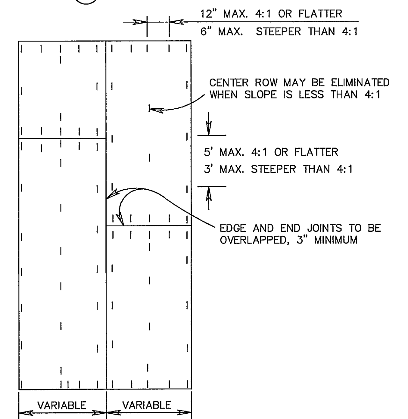
PLAN VIEW
