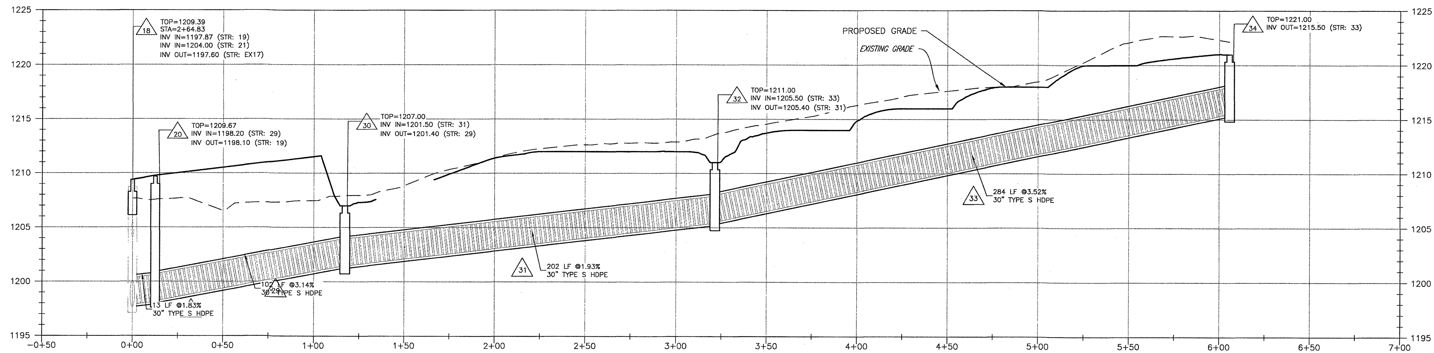
STORM 34-40 PROFILE
