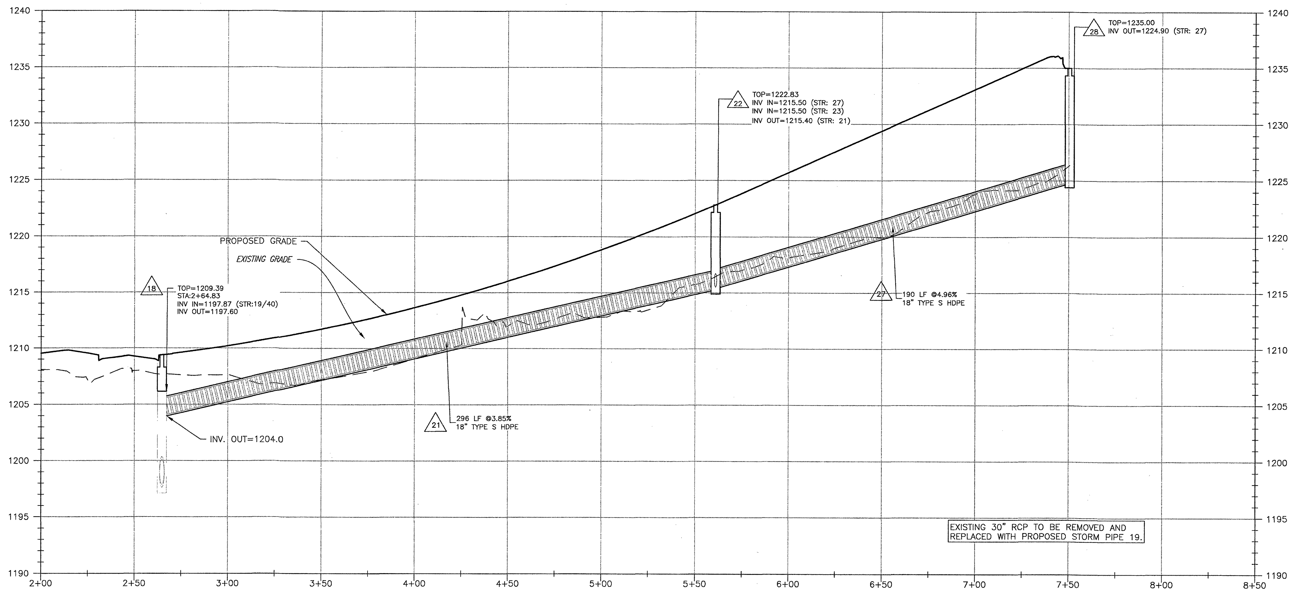
STORM 28-18 PROFILE
