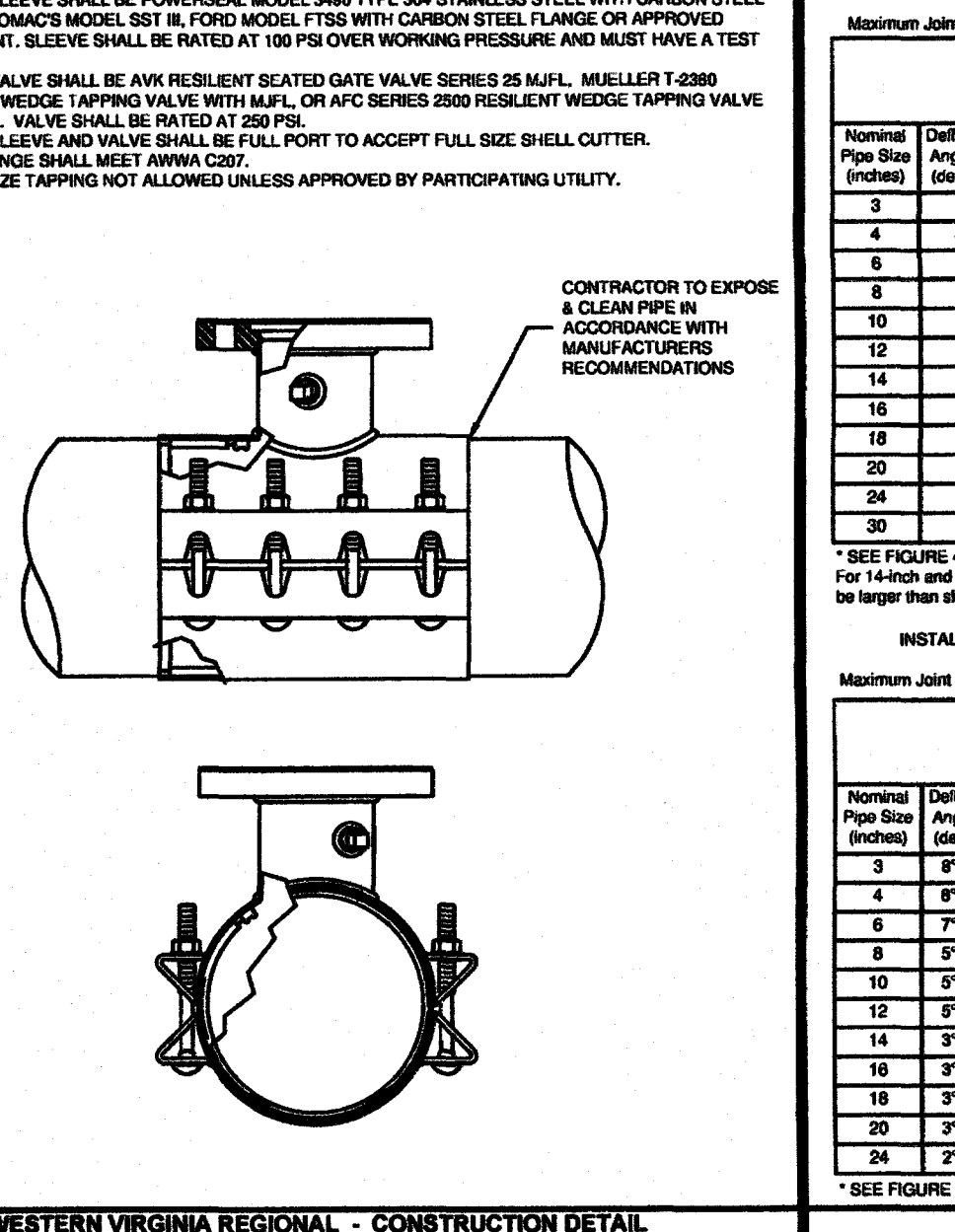
WESTERN VIRGINIA REGIONAL - CONSTRUCTION DETAIL TAPPING SLEEVE AND VALVE 01/01/14
