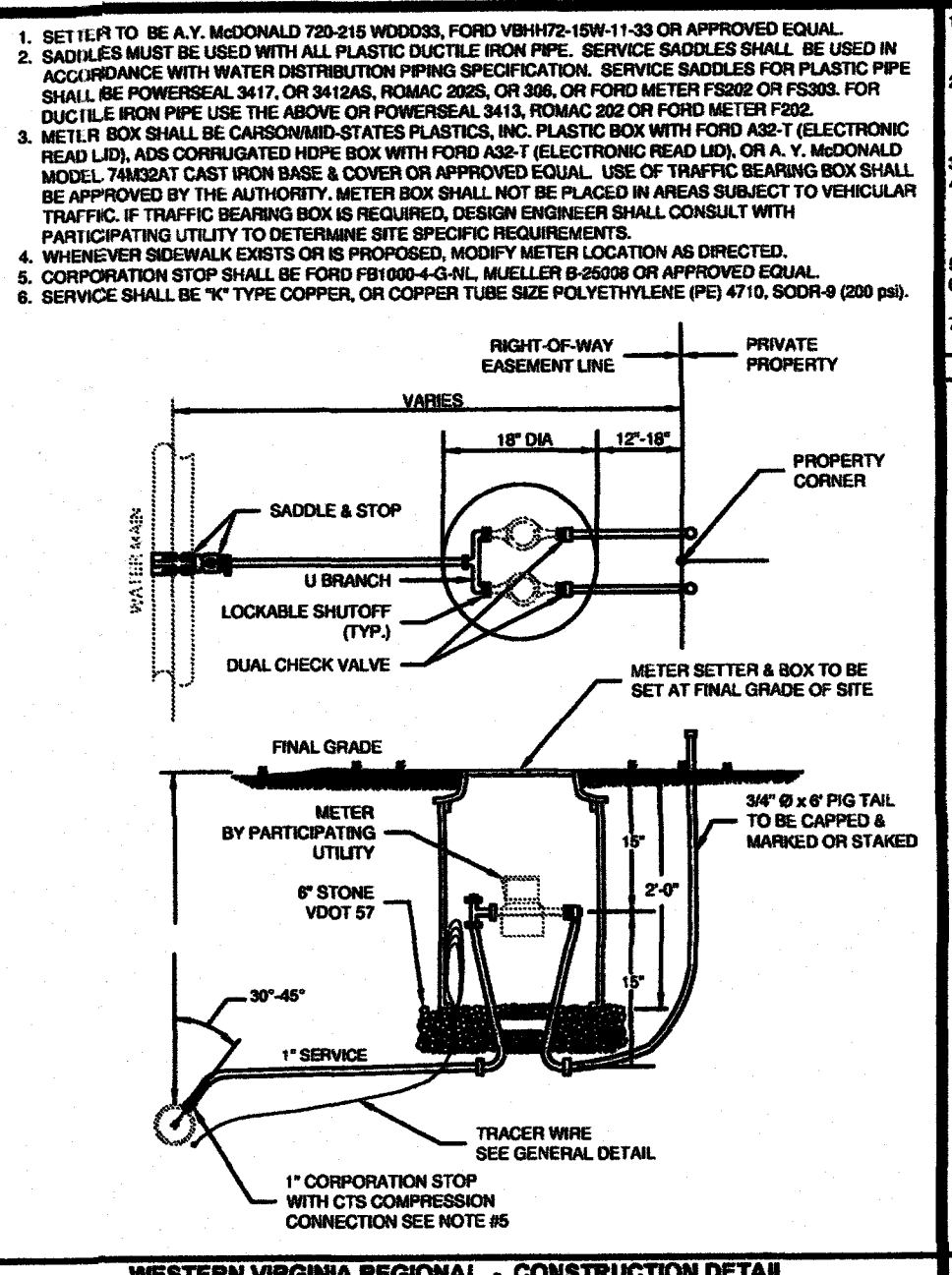
WESTERN VIRGINIA REGIONAL - CONSTRUCTION DETAIL DOUBLE RESIDENTIAL WATER SERVICE 02/10/15
