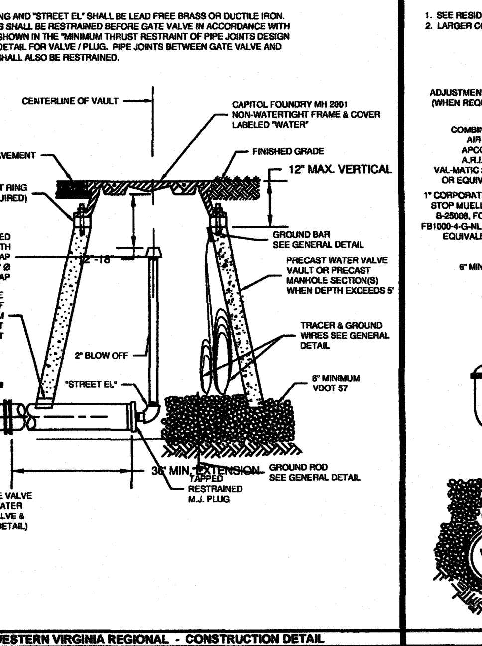
WESTERN VIRGINIA REGIONAL - CONSTRUCTION DETAIL TEMPORARY END OF LINE BLOW-OFF ASSEMBLY 01/01/14
