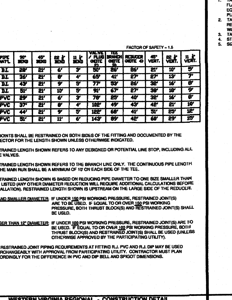
WESTERN VIRGINIA REGIONAL - CONSTRUCTION DETAIL MINIMUM THRUST RESTRAINT OF PIPE JOINTS DESIGN LENGTHS 02/10/15
