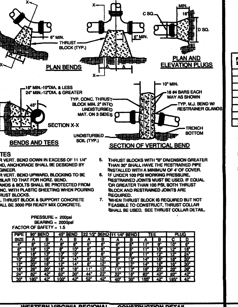
WESTERN VIRGINIA REGIONAL - CONSTRUCTION DETAIL THRUST BLOCK REQUIREMENTS 01/01/14
