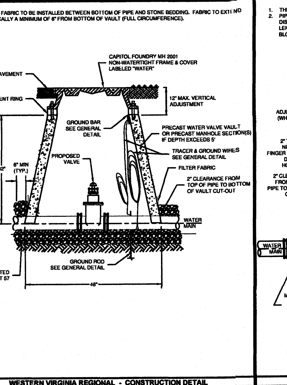
WESTERN VIRGINIA REGIONAL - CONSTRUCTION DETAIL WATER LINE VALVE & VAULT 01/01/14
