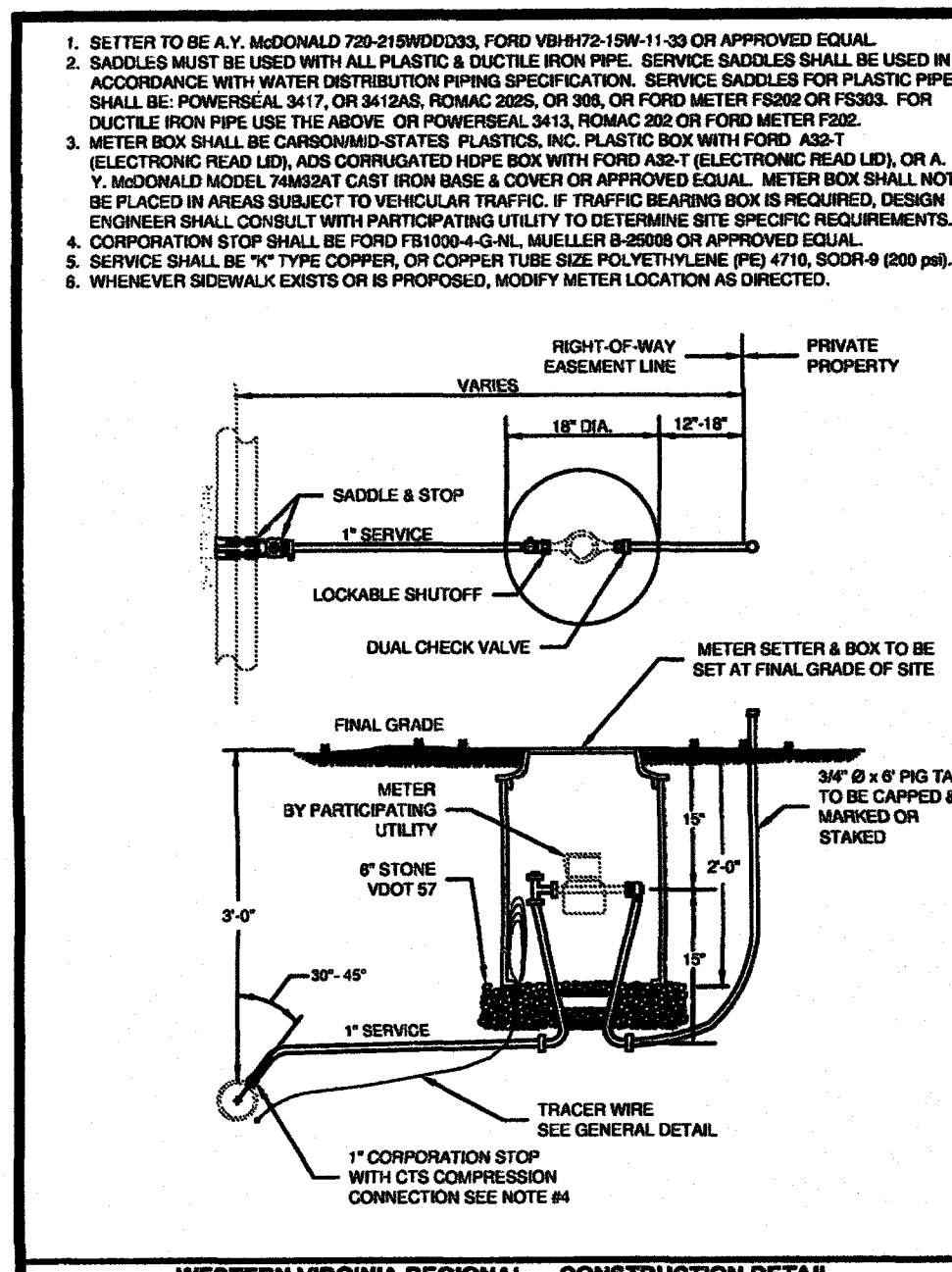
WESTERN VIRGINIA REGIONAL - CONSTRUCTION DETAIL SINGLE RESIDENTIAL WATER SERVICE (NEW DEVELOPMENT) 01/01/15
