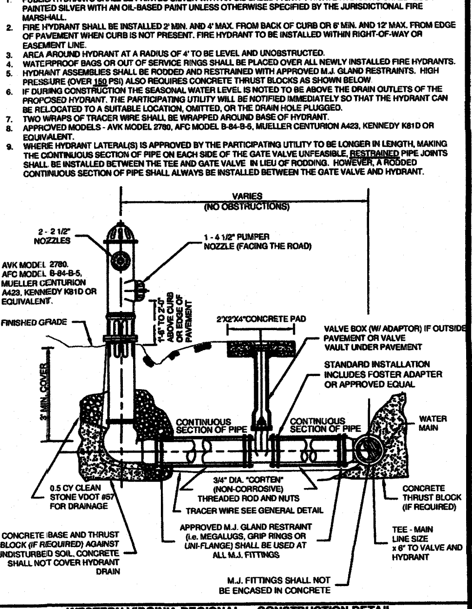
WESTERN VIRGINIA REGIONAL - CONSTRUCTION DETAIL FIRE HYDRANT ASSEMBLY 02/10/15
