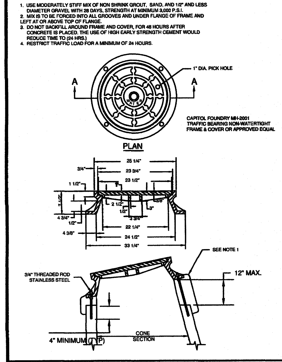
WESTERN VIRGINIA REGIONAL - CONSTRUCTION DETAIL VAULT FRAME AND COVER 01/01/14
