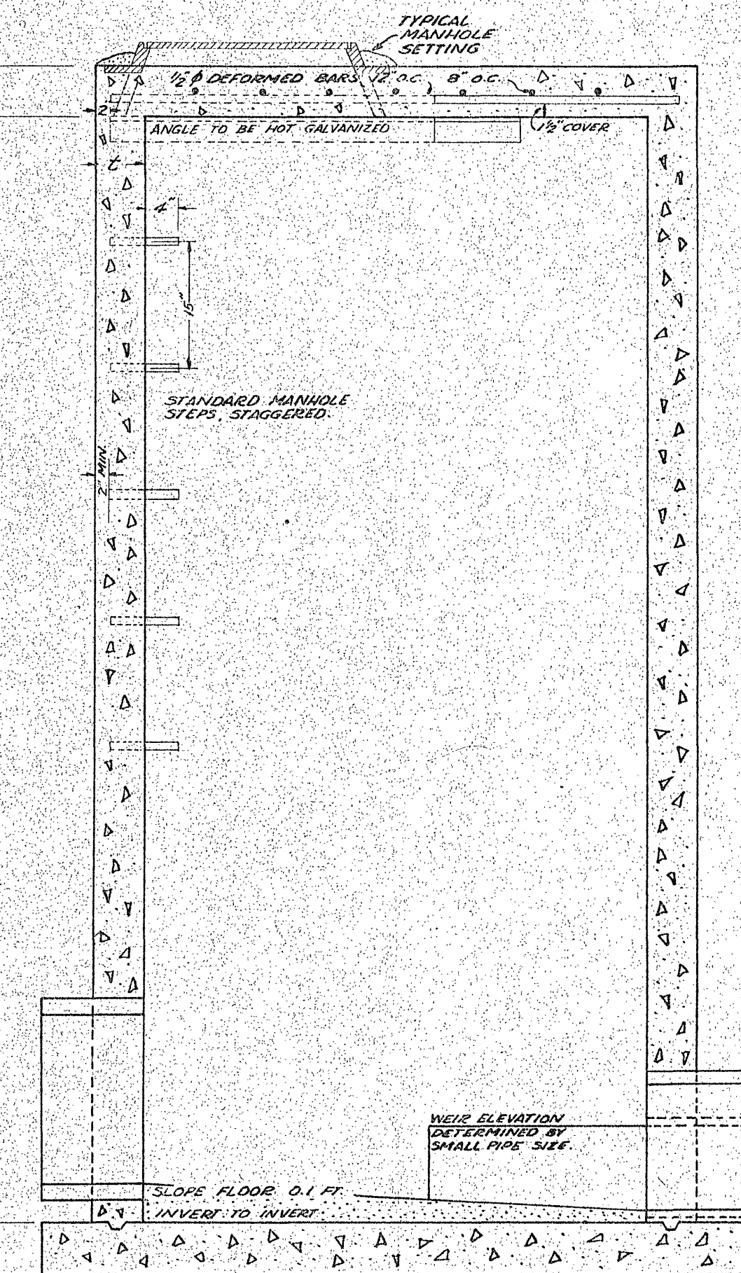
SECTION BB
