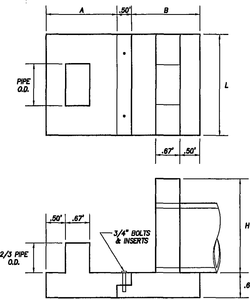
EW-1 MODIFIED WITH ENERGY DISSIPATER
