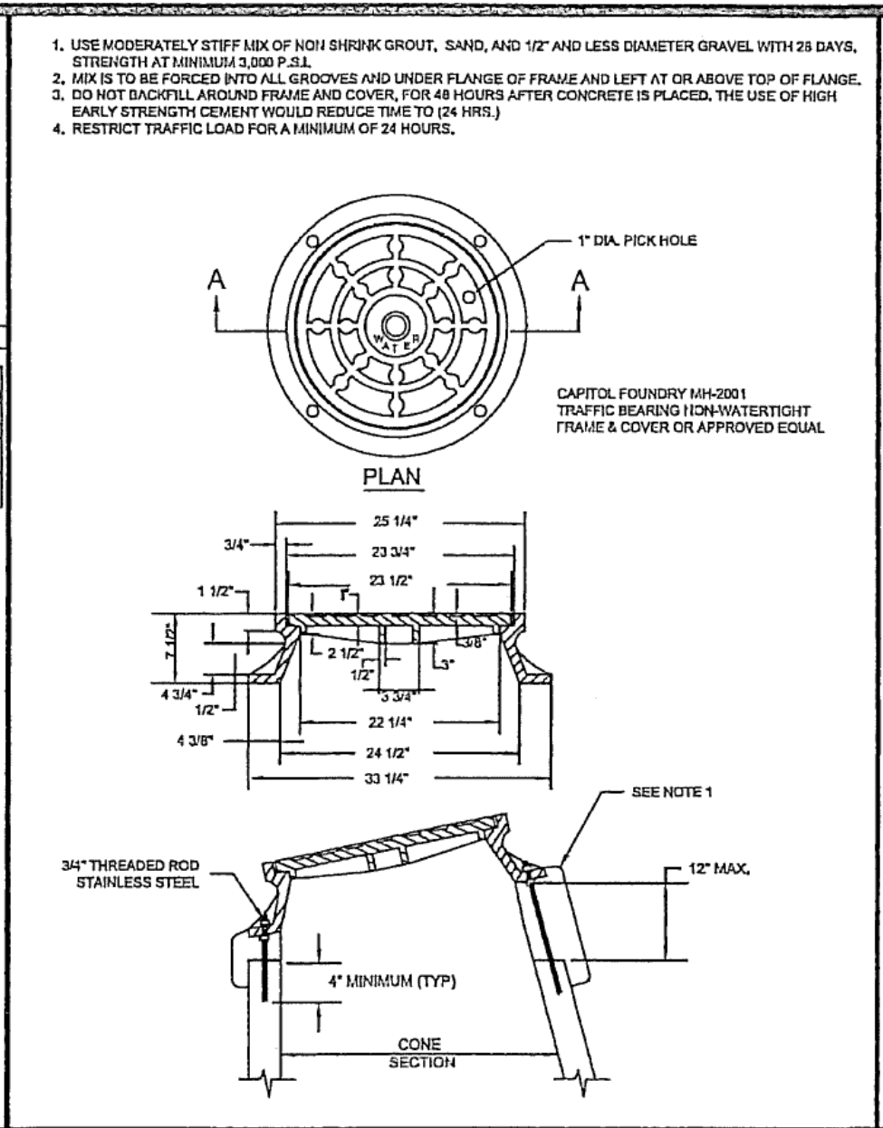
WESTERN VIRGINIA REGIONAL - CONSTRUCTION DETAIL W-16 01/01/14
