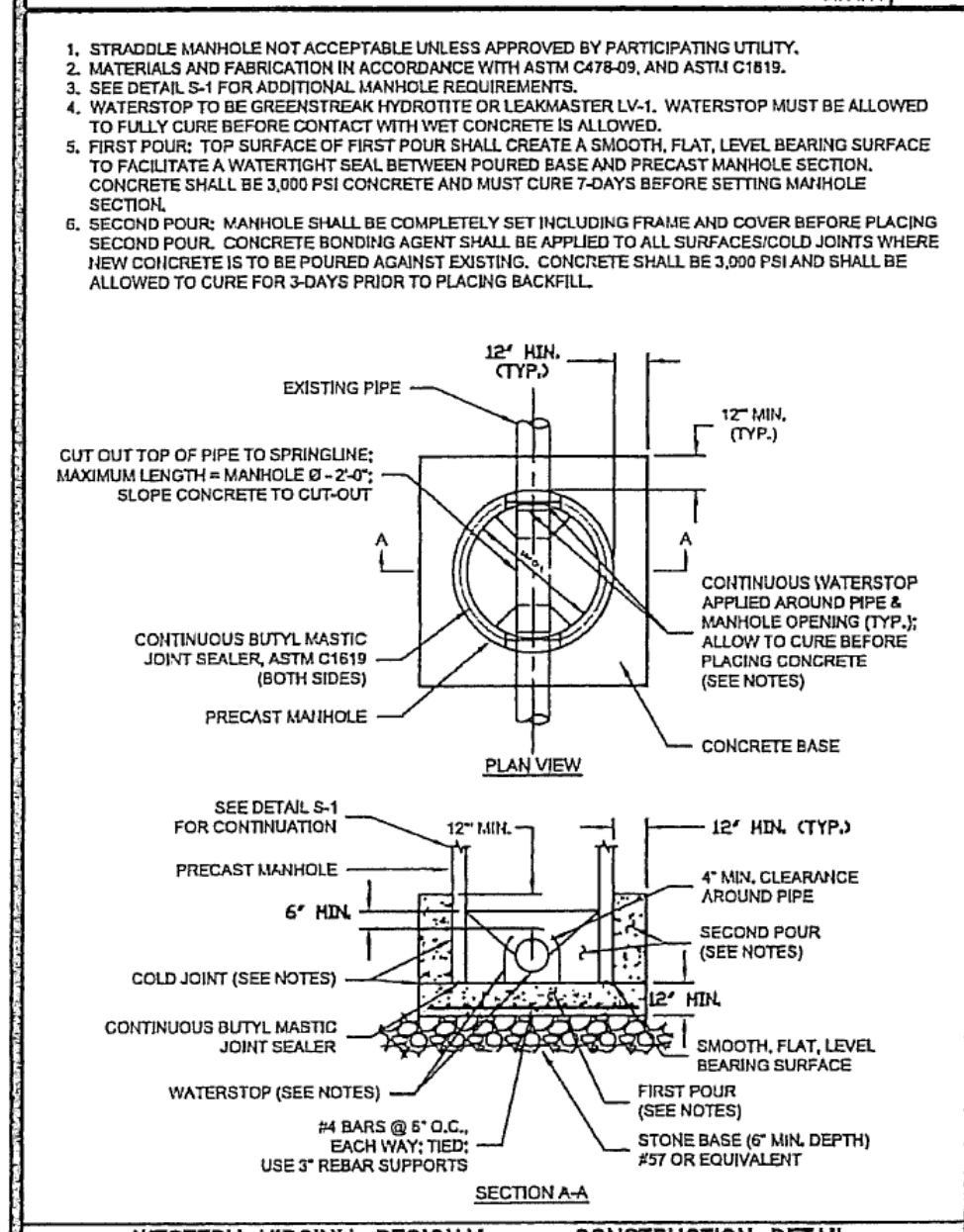
WESTERN VIRGINIA REGIONAL - CONSTRUCTION DETAIL G-11 01/01/14
