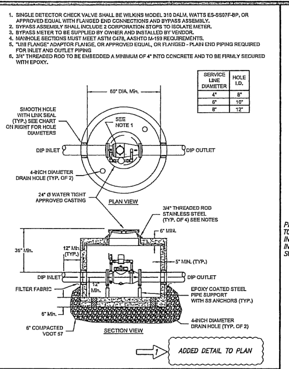
WESTERN VIRGINIA REGIONAL - CONSTRUCTION DETAIL W-8 01/01/14
