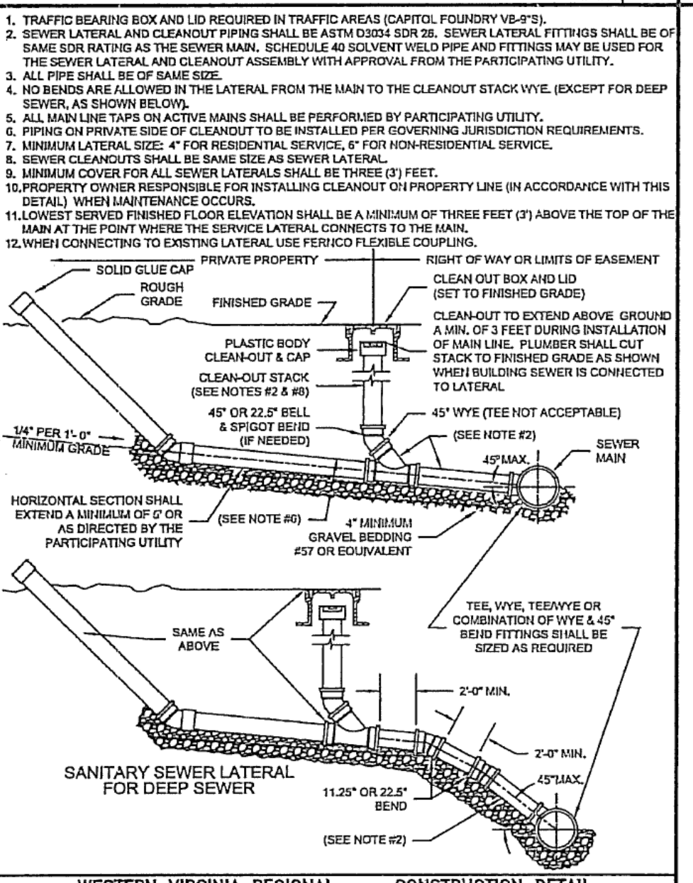
WESTERN VIRGINIA REGIONAL - CONSTRUCTION DETAIL S-2 01/01/14
