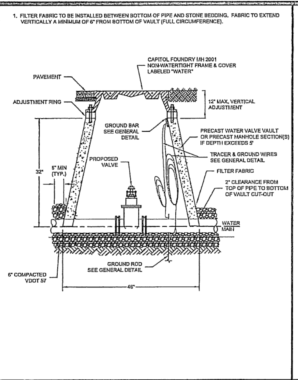
WESTERN VIRGINIA REGIONAL - CONSTRUCTION DETAIL W-9 01/01/14
