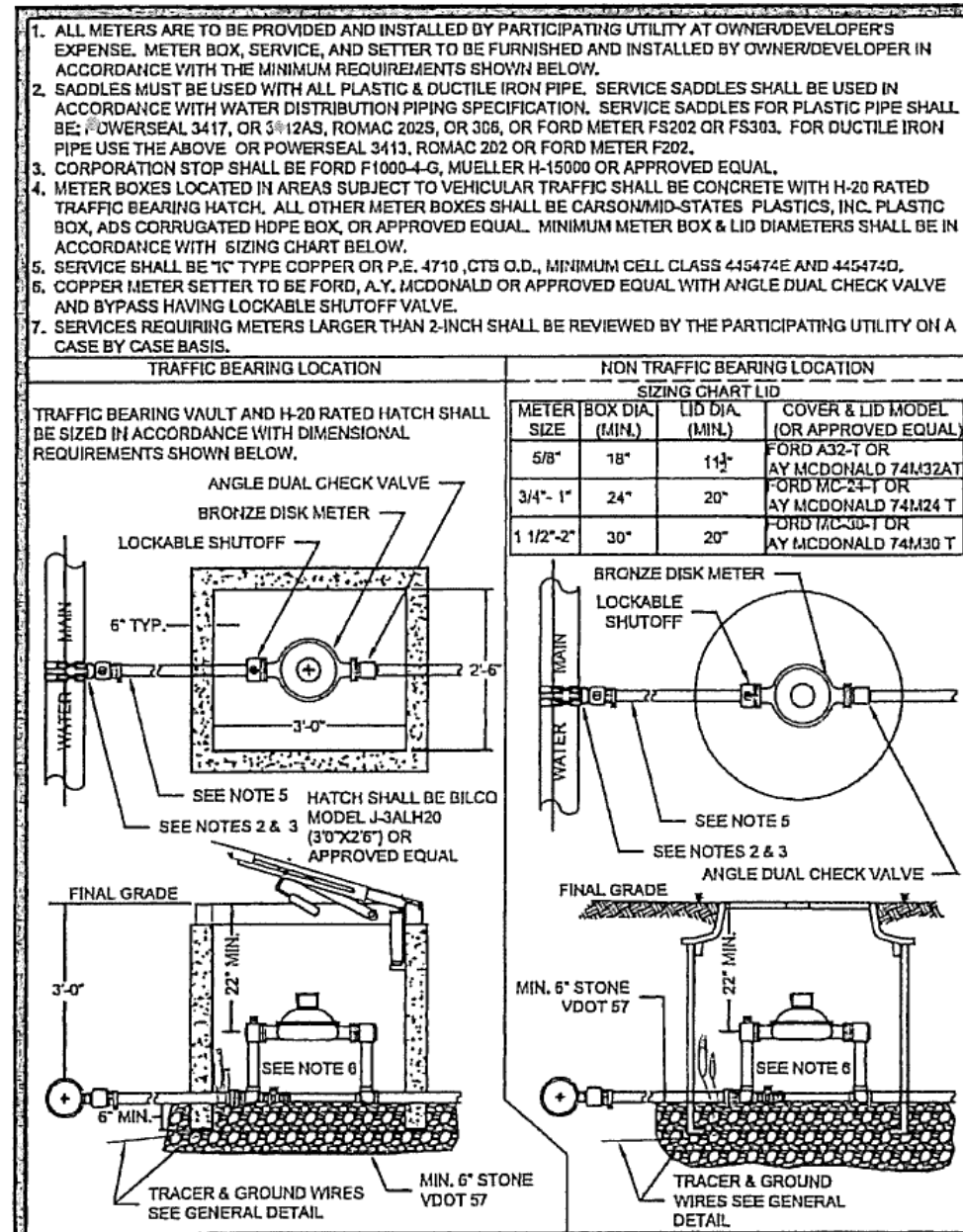
WESTERN VIRGINIA REGIONAL - CONSTRUCTION DETAIL W-5 01/01/14
