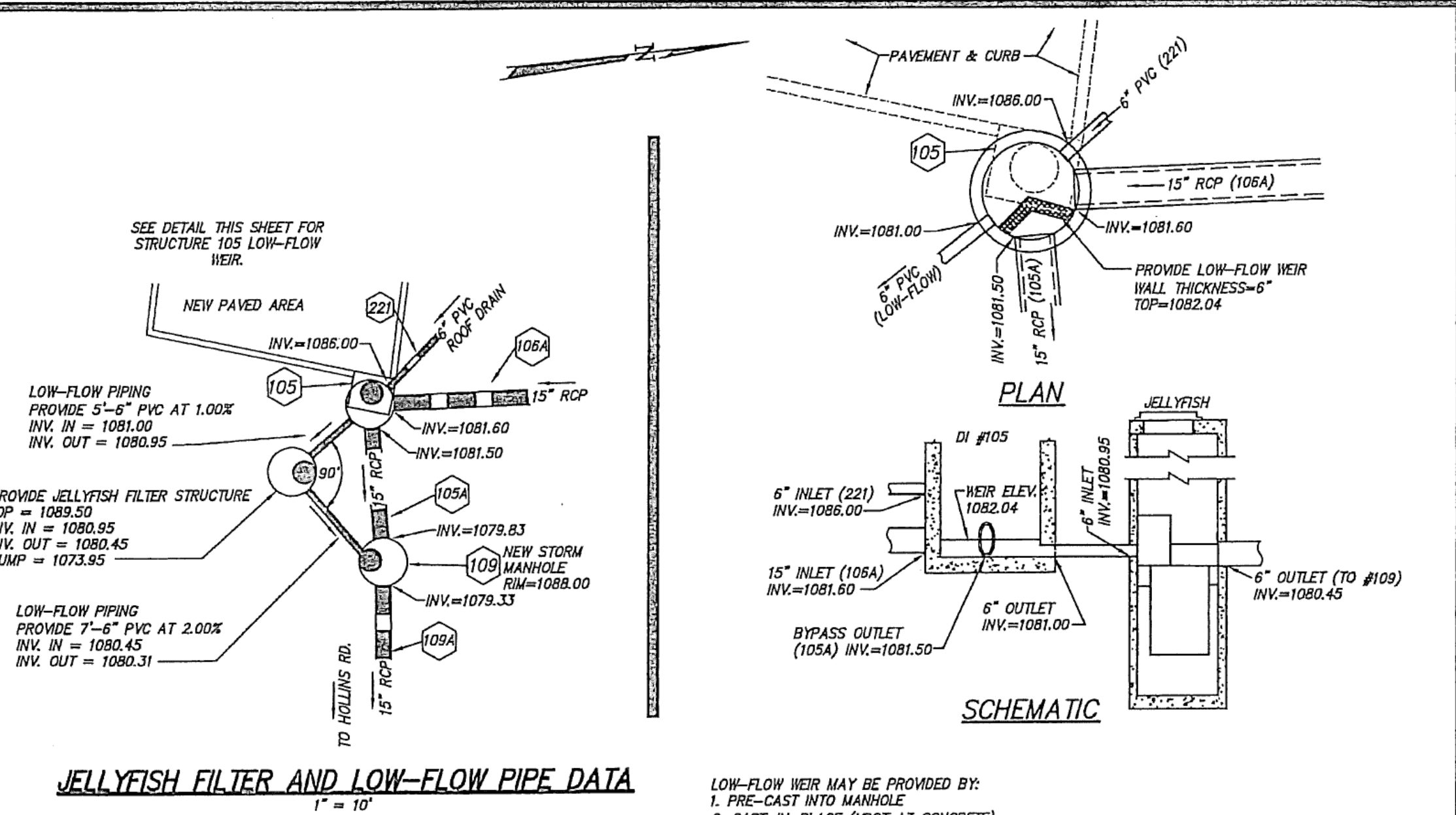
WESTERN VIRGINIA REGIONAL - CONSTRUCTION DETAIL S-2 01/01/14
