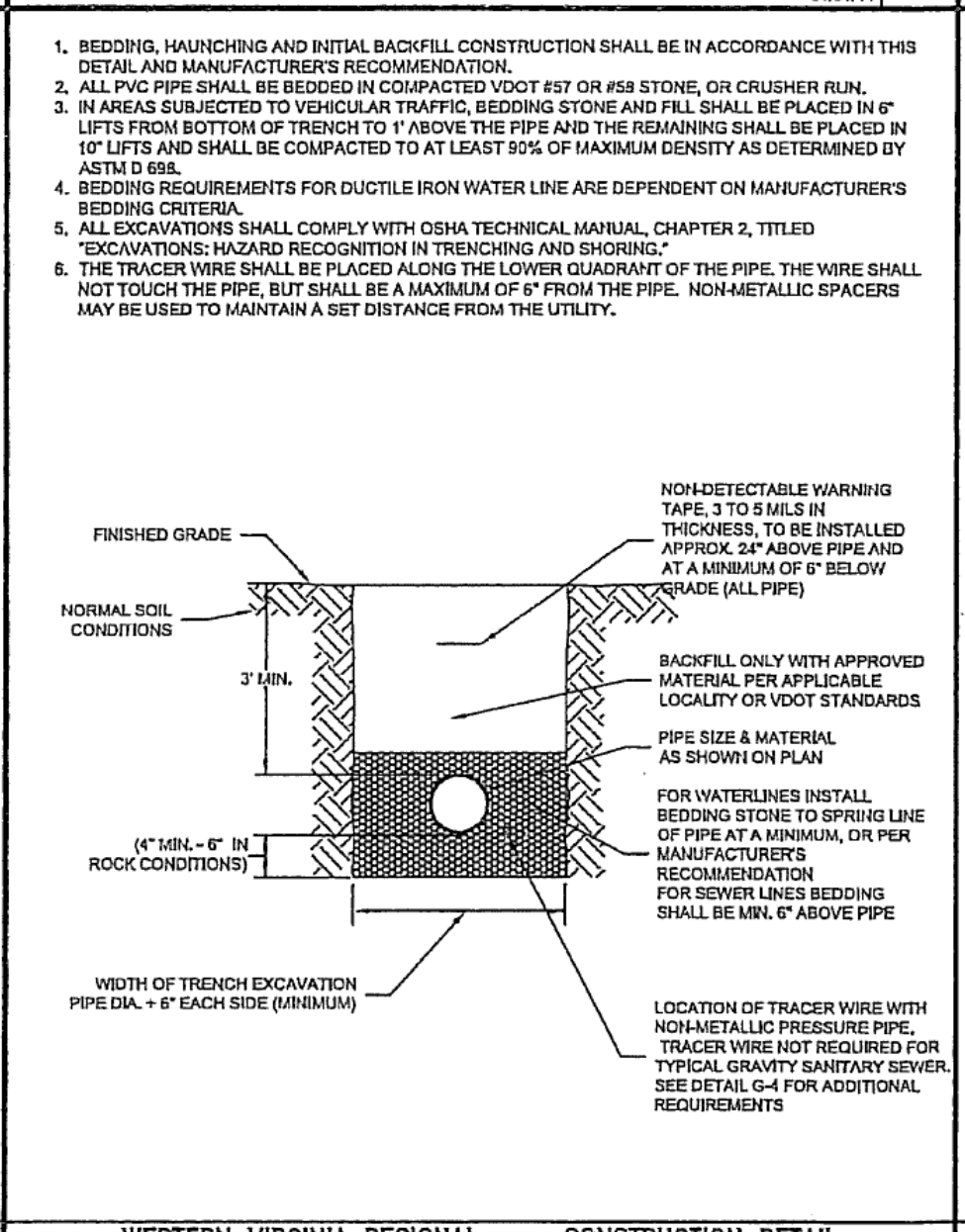
WESTERN VIRGINIA REGIONAL - CONSTRUCTION DETAIL S-6 01/01/14
