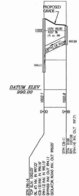
STORM LINE PROFILE @ CB-13 THRU MH-14 VERTICAL SCALE 1"=5' HORIZONTAL SCALE 1"=50'
