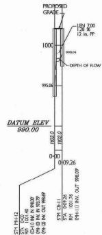
STORM LINE PROFILE @ CB-11 THRU MH-12 VERTICAL SCALE 1"=5' HORIZONTAL SCALE 1"=50'
