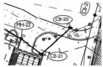
STORM LINE PLAN @ CB-20 THRU MH-22 1"=50'
