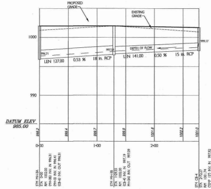
STORM LINE PROFILE @ CB-4 THRU MH-3B VERTICAL SCALE 1"=5' HORIZONTAL SCALE 1"=50'
