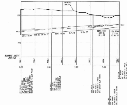
STORM LINE PROFILE @ MH-14 THRU CB-8 VERTICAL SCALE 1"=5' HORIZONTAL SCALE 1"=50'
