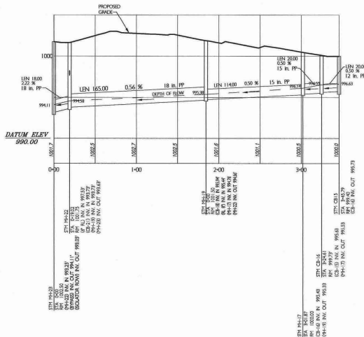
STORM LINE PROFILE @ CB-15 THRU MH-23 VERTICAL SCALE 1"=5' HORIZONTAL SCALE 1"=50'
