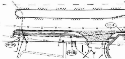
STORM LINE PLAN @ CB-4 THRU CB-6 1"=50'
