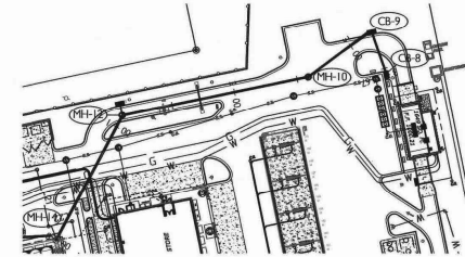
STORM LINE PLAN @ MH-14 THRU CB-8 1"=50'
