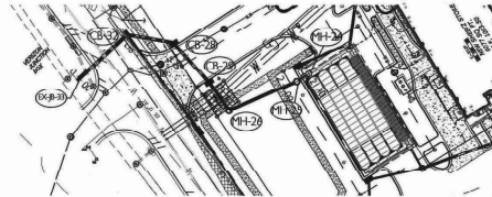
STORM LINE PLAN @ MH-24 THRU EX-JB-32 1"=50'
