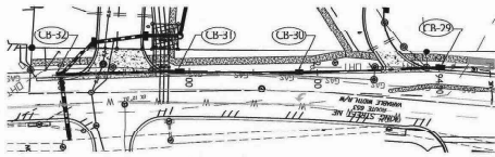
STORM LINE PLAN @ CB-29 THRU CB-32 1"=50'
