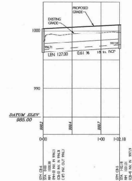
STORM LINE PROFILE @ CB-5 THRU CB-6 VERTICAL SCALE 1"=5' HORIZONTAL SCALE 1"=50'
