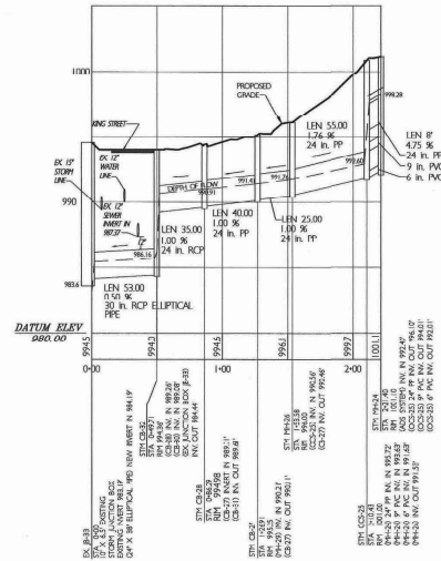
STORM LINE PROFILE @ MH-24 THRU EX-JB-32 VERTICAL SCALE 1"=5' HORIZONTAL SCALE 1"=50'
