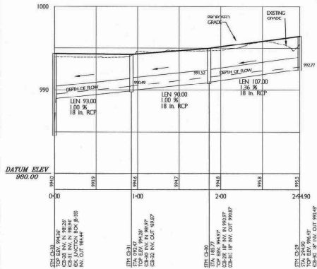
STORM LINE PROFILE @ CB-29 THRU CB-32 VERTICAL SCALE 1"=5' HORIZONTAL SCALE 1"=50'
