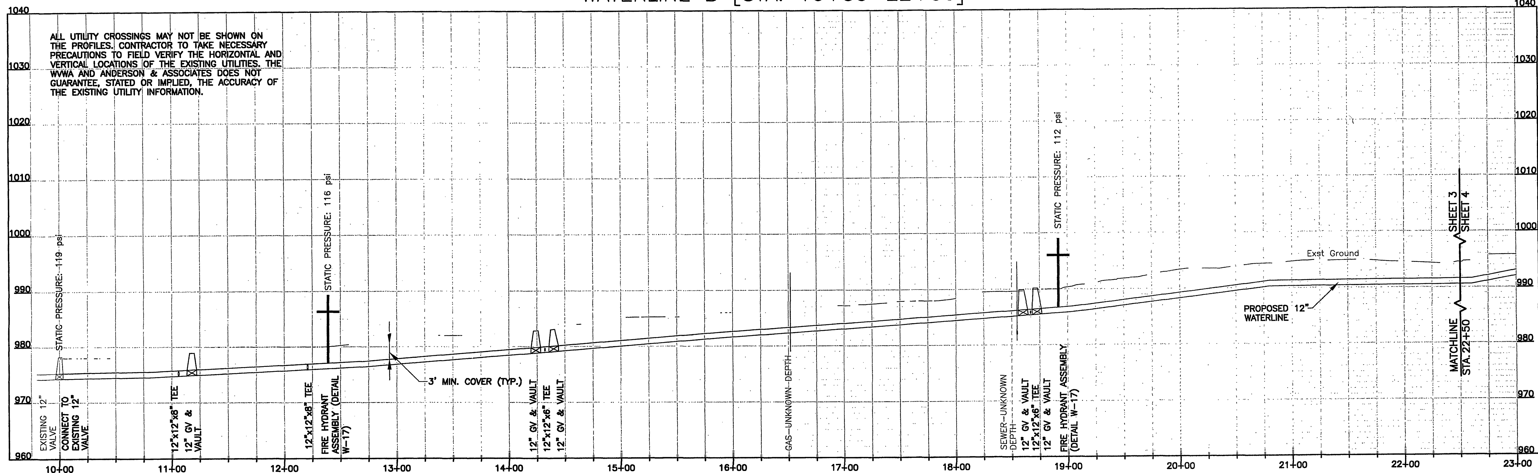
WATERLINE B [STA. 10+00-22+50]
