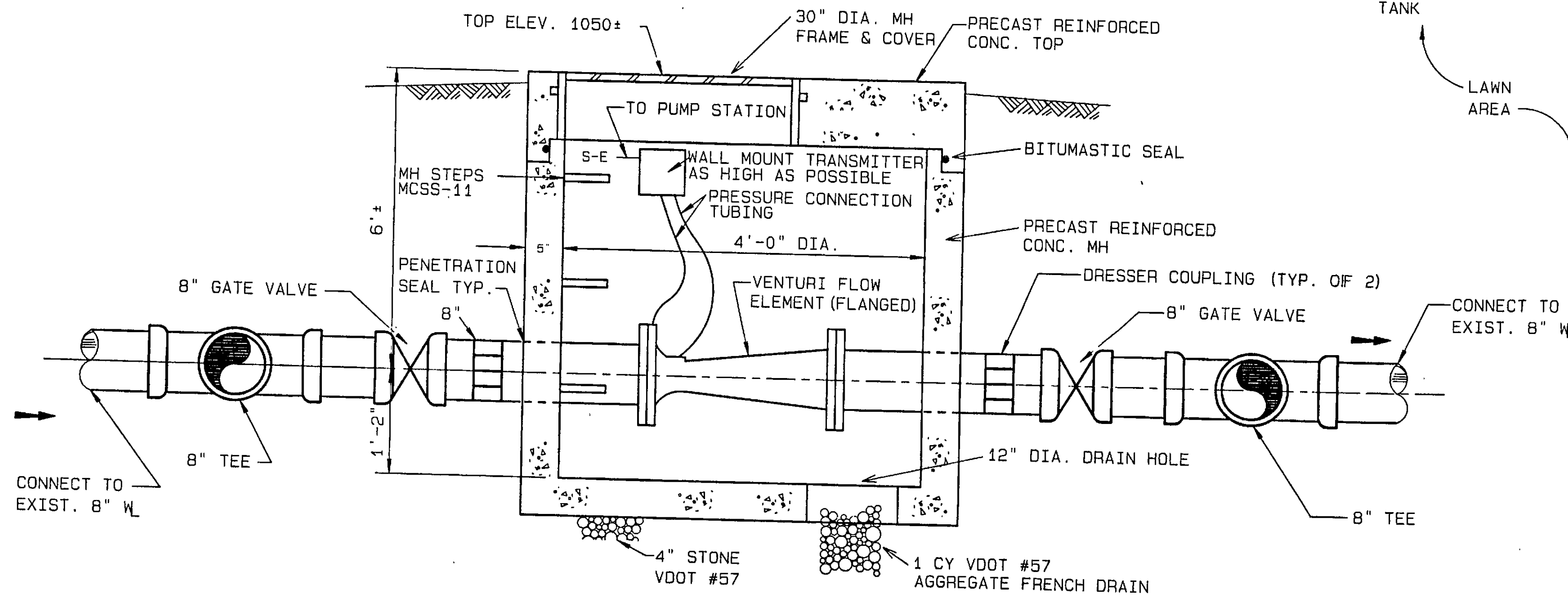
SECTION - FLOW MEASUREMENT VAULT NO SCALE
