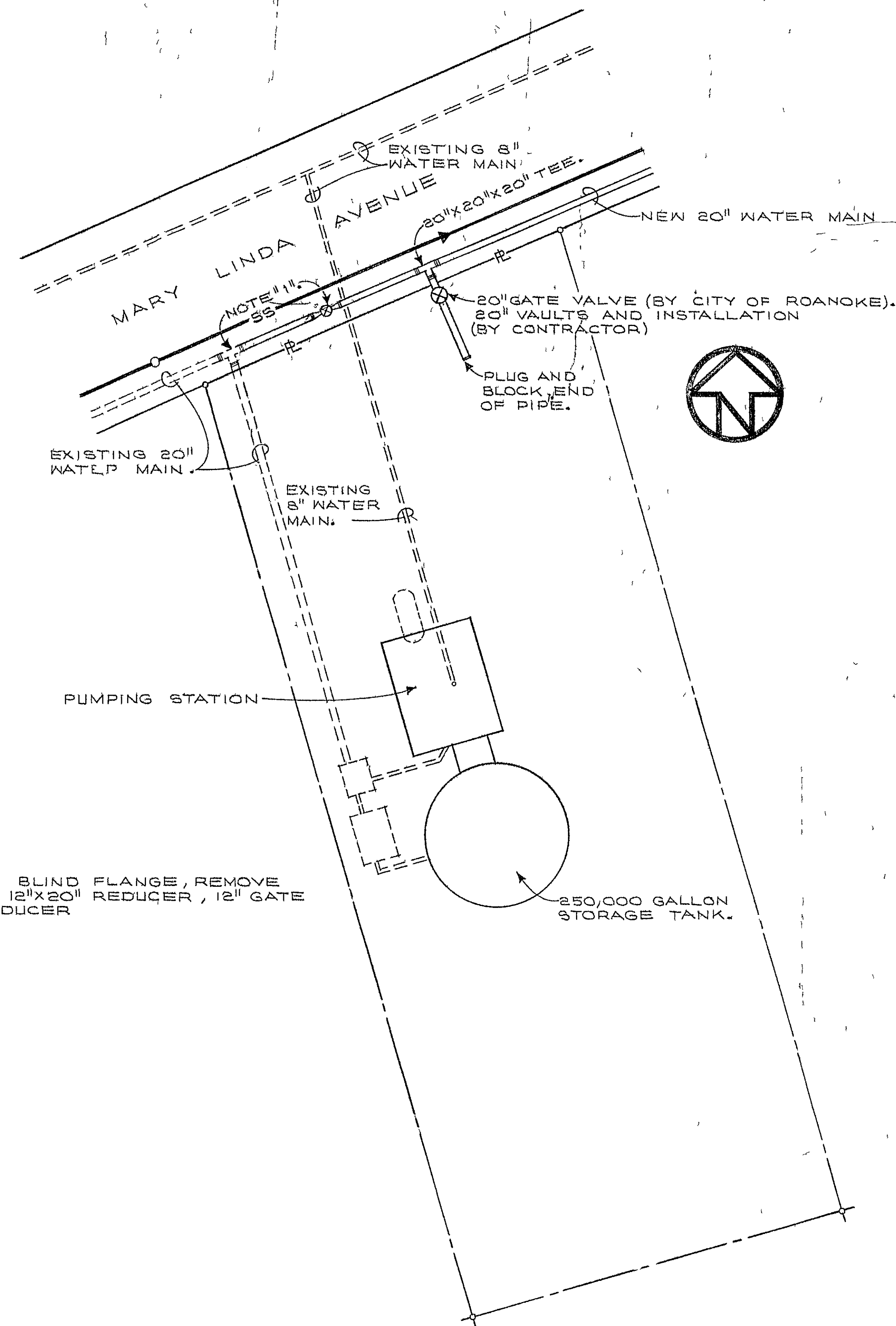
SITE PLAN - PUMPING STATION SCALE 1" = 20'-0"
