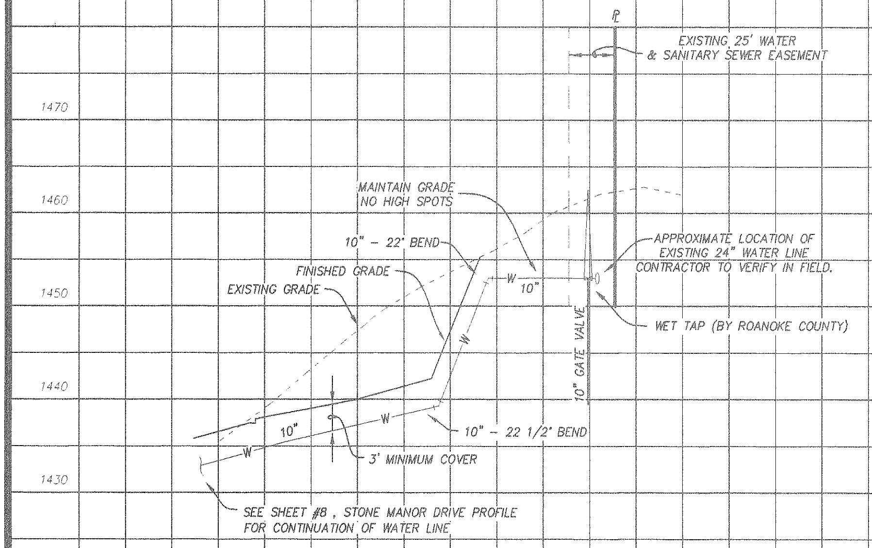
WATER LINE PROFILES SCALE: 1" = 50' HORIZ. 1" = 10' VERT.
