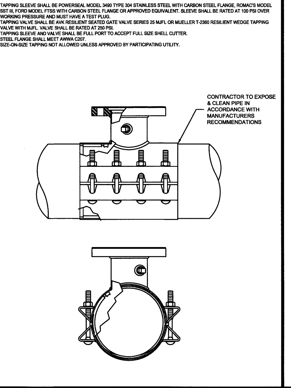
WESTERN VIRGINIA REGIONAL - CONSTRUCTION DETAIL TAPPING SLEEVE AND VALVE 01/01/12 W-21
