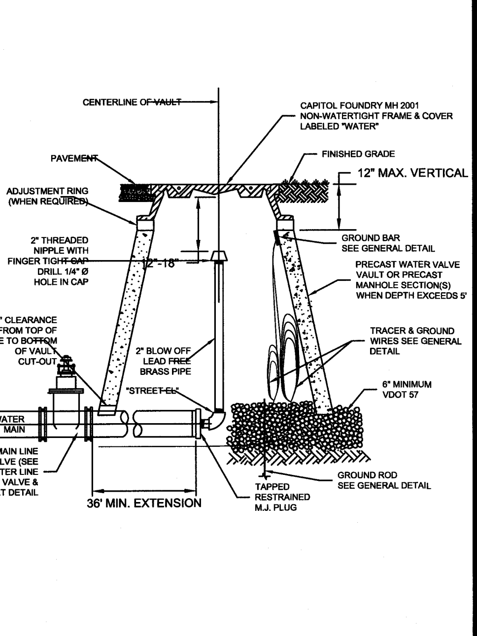
WESTERN VIRGINIA REGIONAL - CONSTRUCTION DETAIL TEMPORARY END OF LINE BLOW-OFF ASSEMBLY 01/01/12 W-11
