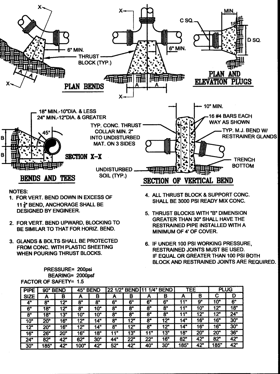
WESTERN VIRGINIA REGIONAL - CONSTRUCTION DETAIL THRUST BLOCK REQUIREMENTS 01/01/12 W-18
