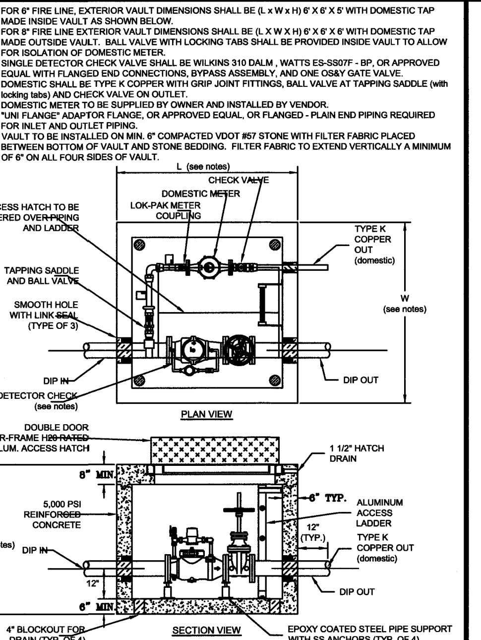
WESTERN VIRGINIA REGIONAL - CONSTRUCTION DETAIL COMMERCIAL METER VAULT 01/01/12 W-7
