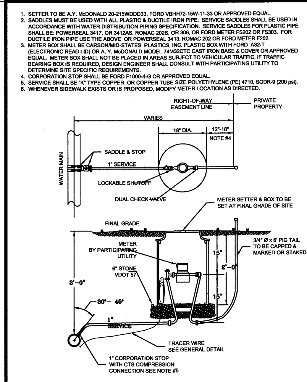
WESTERN VIRGINIA REGIONAL - CONSTRUCTION DETAIL SINGLE RESIDENTIAL WATER SERVICE - (NEW DEVELOPMENT) (LINE PRESSURE UNDER 150 PSI) 01/01/12 W-1
