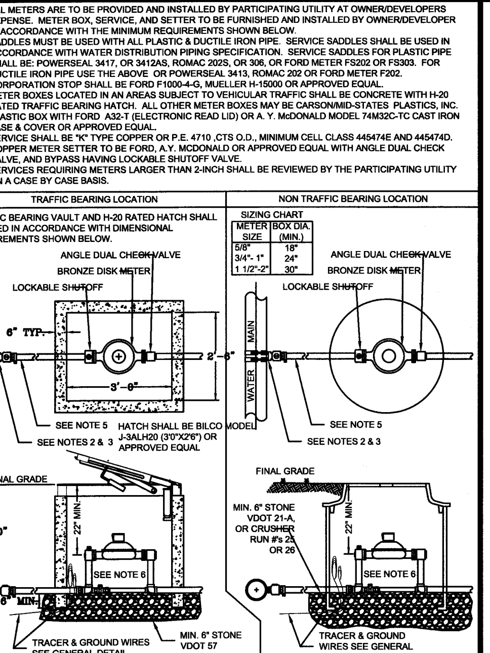
WESTERN VIRGINIA REGIONAL - CONSTRUCTION DETAIL COMMERCIAL WATER SERVICE METER SIZES 5/8\"/>
