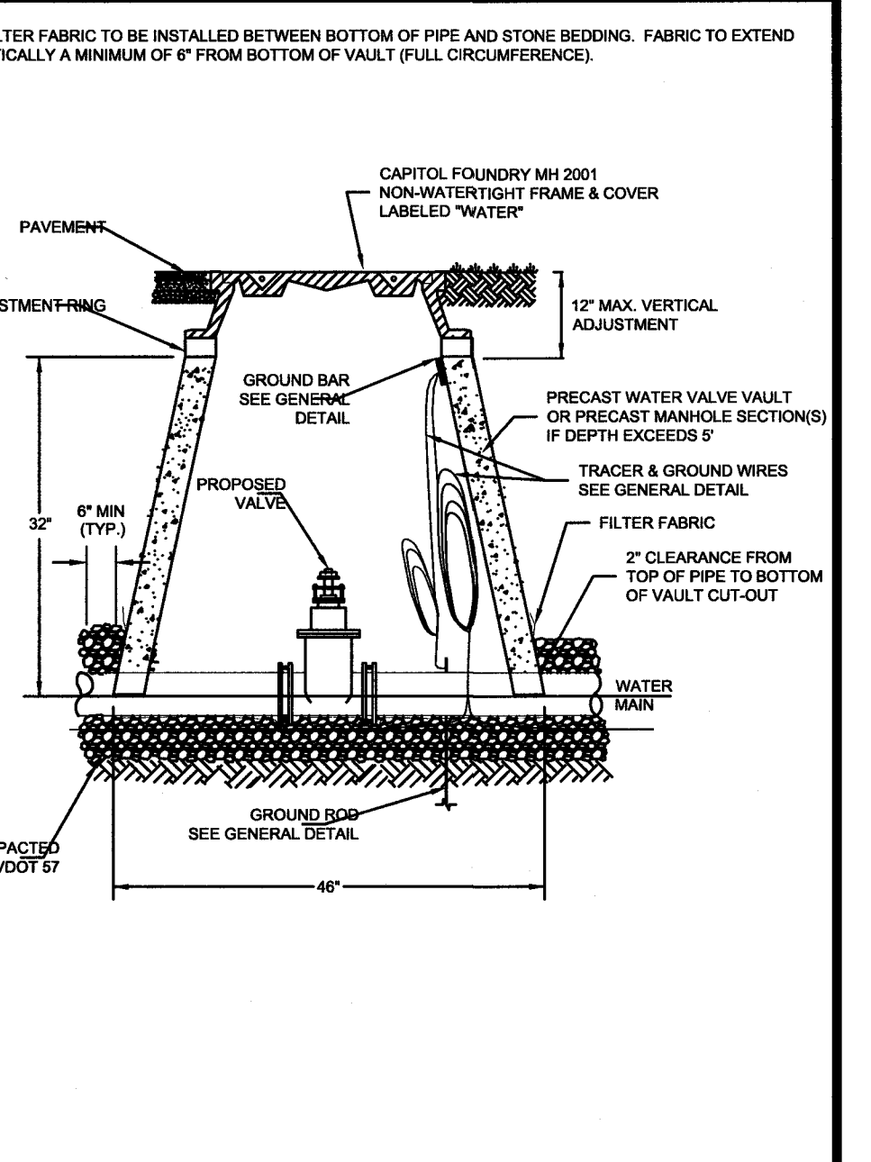
WESTERN VIRGINIA REGIONAL - CONSTRUCTION DETAIL WATER LINE VALVE & VAULT 01/01/12 W-9
