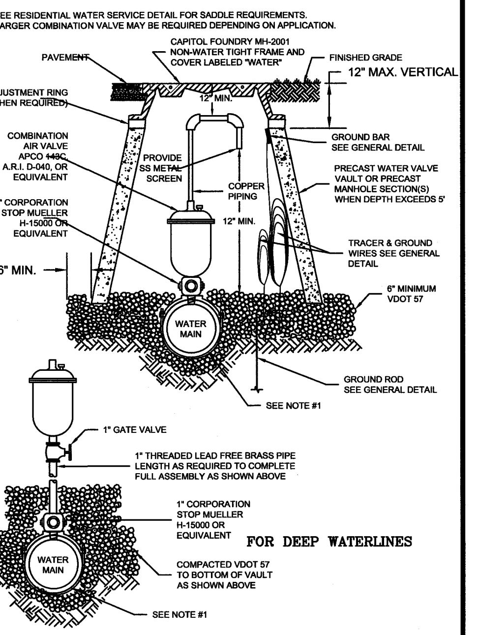
WESTERN VIRGINIA REGIONAL - CONSTRUCTION DETAIL COMBINATION AIR VALVE ASSEMBLY 01/01/12 W-13
