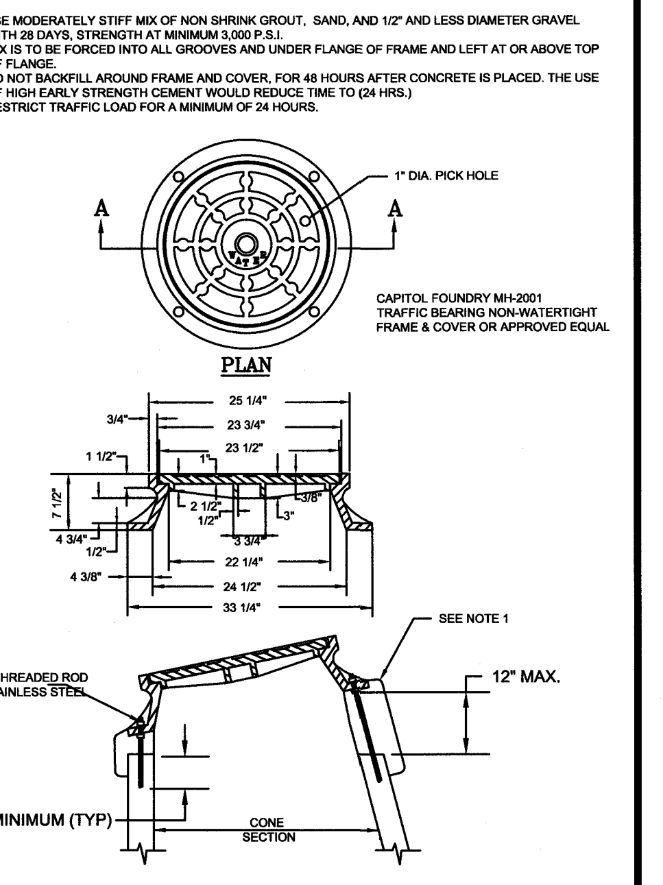
WESTERN VIRGINIA REGIONAL - CONSTRUCTION DETAIL VAULT FRAME AND COVER 01/01/12 W-16
