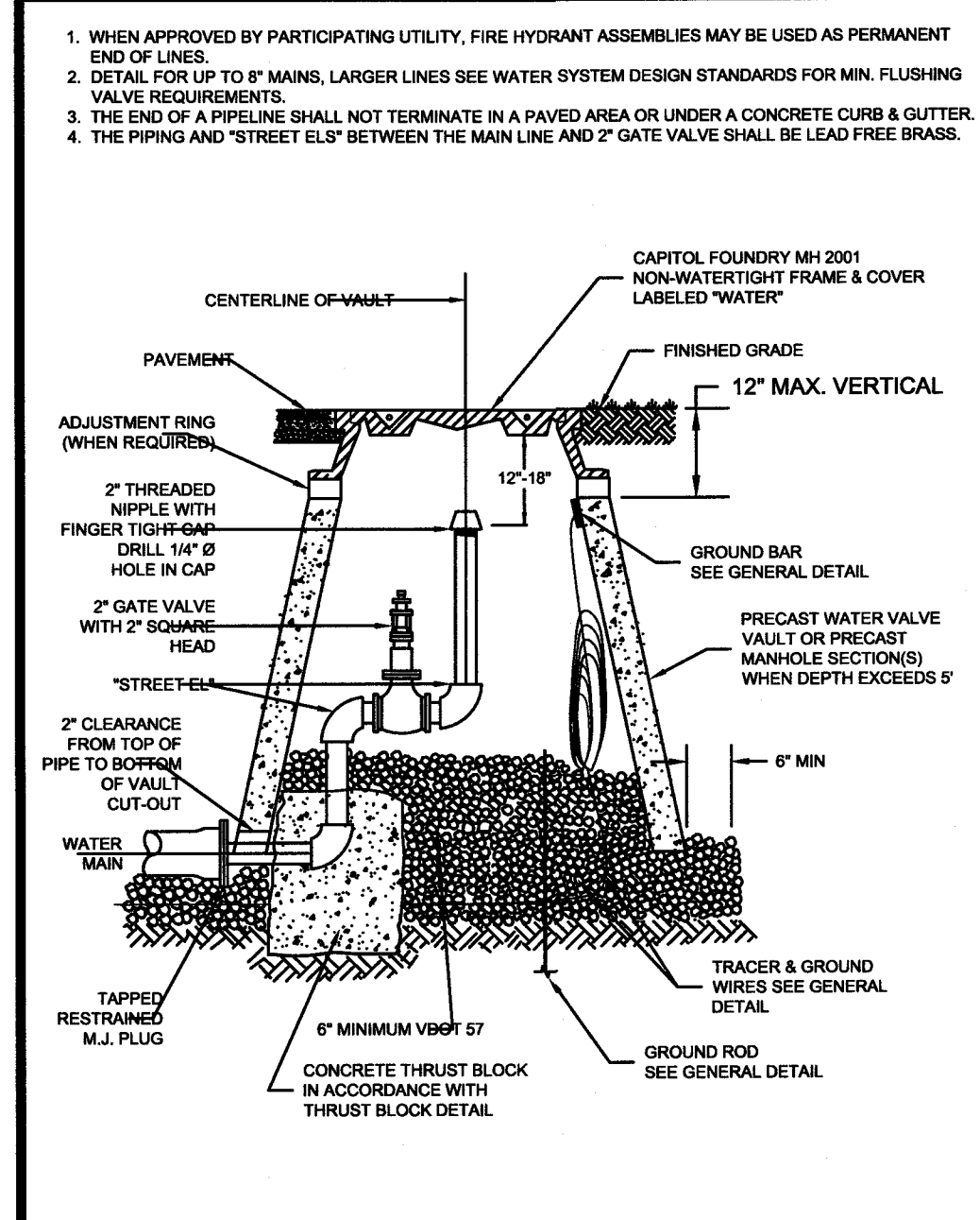
WESTERN VIRGINIA REGIONAL - CONSTRUCTION DETAIL PERMANENT END OF LINE BLOW-OFF ASSEMBLY 01/01/12 W-10
