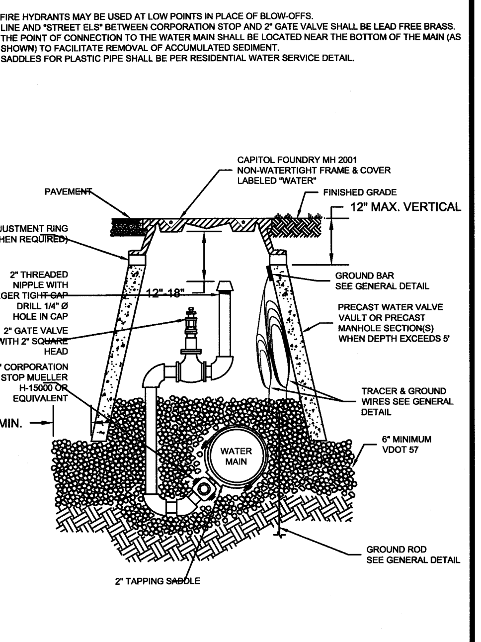
WESTERN VIRGINIA REGIONAL - CONSTRUCTION DETAIL IN-LINE BLOW-OFF ASSEMBLY 01/01/12 W-12
