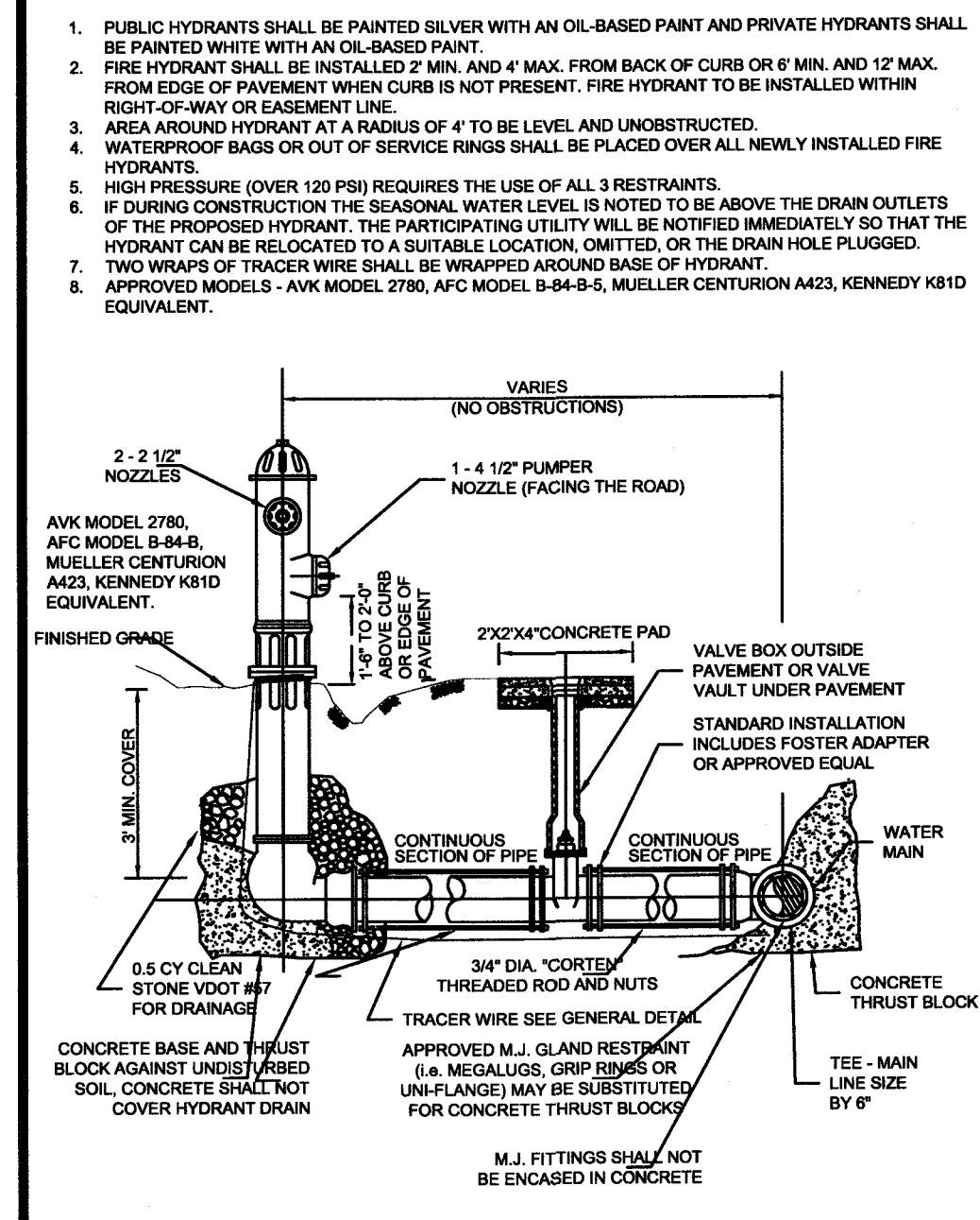
WESTERN VIRGINIA REGIONAL - CONSTRUCTION DETAIL FIRE HYDRANT ASSEMBLY 01/01/12 W-17
