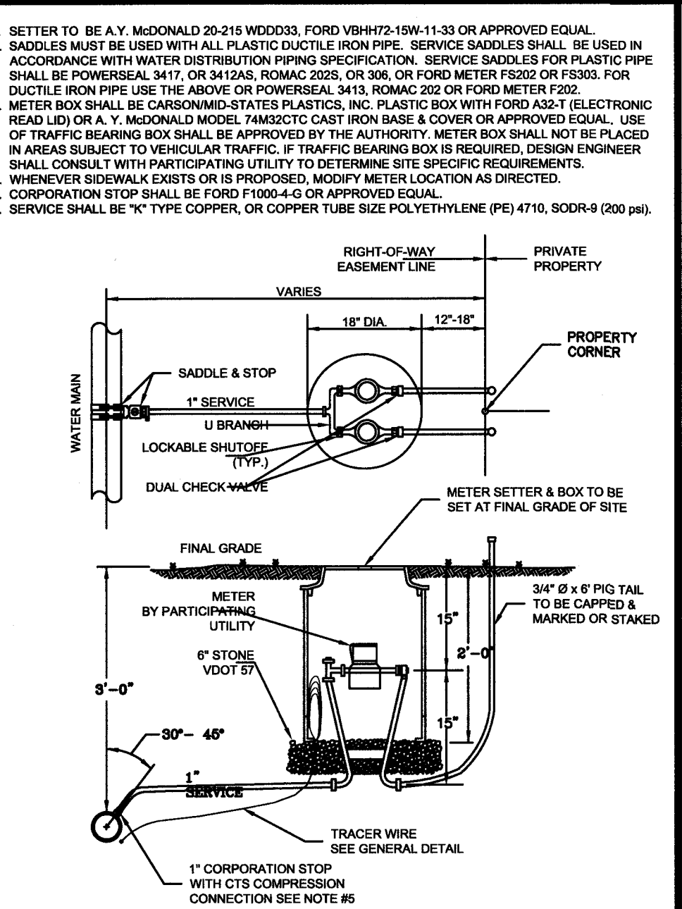
WESTERN VIRGINIA REGIONAL - CONSTRUCTION DETAIL DOUBLE RESIDENTIAL WATER SERVICE (LINE PRESSURE UNDER 150 PSI) 01/01/12 W-4
