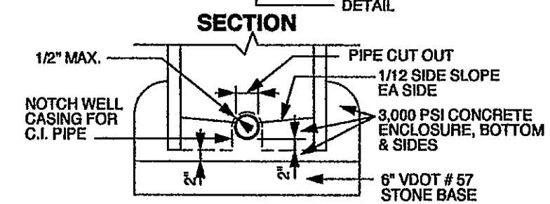
SAMPLING CATCH BASIN DETAIL C5.1 SCALE: 1/2" = 1'-0"
