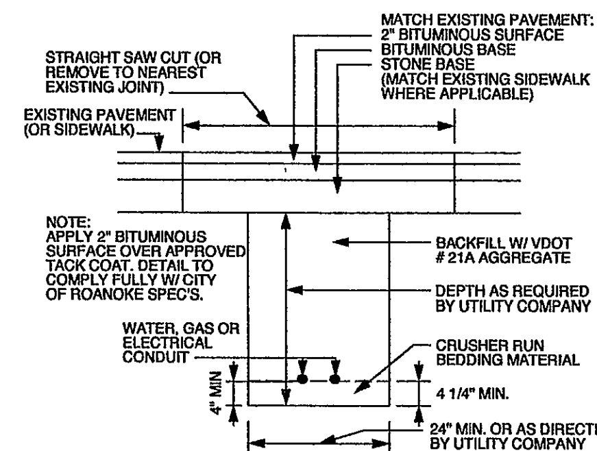
UTILITY TRENCH REPAIR DETAIL C5.2 SCALE: 1/2" = 1'-0"
